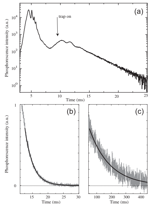
FIG. 2: Semilogarithmic plot of the phosphorescence intensity from the trap region as a function of time after production of CO molecules in the (1,0,1) level in the source chamber (a). The time at which the trap is switched on is indicated by an arrow. Phosphorescence decay curves are shown on a linear scale for CO molecules in the (1,0,1) level (b) and in the (2,0,2) level (c). The solid lines are the results of a weighted least-square fit to a single exponentially decaying curve.
