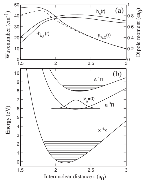
FIG. 3: Panel (a) shows the A - X electronic transition dipole moment \mu_{A,X}(r) (in ea_0 ) of the present work (the solid line) and from Ref. [21] (the dashed line), together with the diagonal [h_a(r)] and offdiagonal [h_{A,a}(r)] spin-orbit coupling (in \text{cm}^{-1} ). Panel (b) shows the RKR-potentials of the X^1\Sigma^+ , the a^3\Pi , and the A^1\Pi states of CO and the |v_a = 0\rangle vibrational wavefunction.
