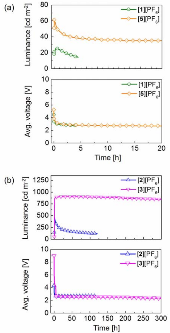
Figure 9. Luminance and average voltage for ITO/PEDOT:PSS/iTMC:[Bmim][PF 6 ] (4:1 molar ratio)/Al LEC devices measured by applying a block-wave pulsed current of 100 \text{ A}\cdot\text{m}^{-2} at a frequency of 1 kHz and duty cycles of 50%. a) iTMC = [1][\text{PF}_6] and [5][\text{PF}_6] ; b) iTMC = [2][\text{PF}_6] and [3][\text{PF}_6] .
