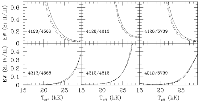
Fig. 2. Examples of calibrations between various Si line ratios and the effective temperature, as a function of \xi . The dependence on the microturbulence must in certain cases be taken into account, as the lines used may be of very different strength. Solid line: \xi=5 km s -1 ; dotted line: \xi=10 km s -1 ; dashed line: \xi=15 km s -1 . In this case we adopted \log g=3.5 [cgs], \log \epsilon(\text{Si})=7.20 dex and \xi_{\text{mod}}=8 km s -1 .
