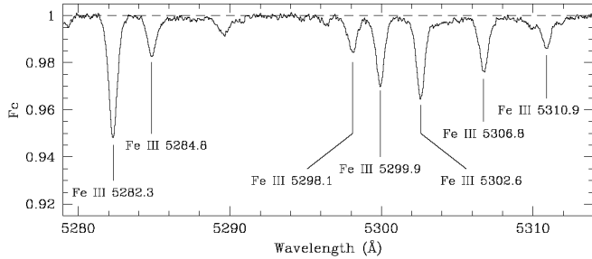
Fig. 1. Mean, normalized spectrum of \beta CMa in the spectral range 5279–5314 \text{\AA} . Some weak Fe III lines are indicated.
