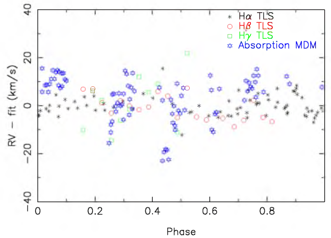
Figure 4. Residuals of the H \alpha , H \beta , H \gamma and the MDM absorption lines as compared with the best fit sinusoid to the H \alpha data.
