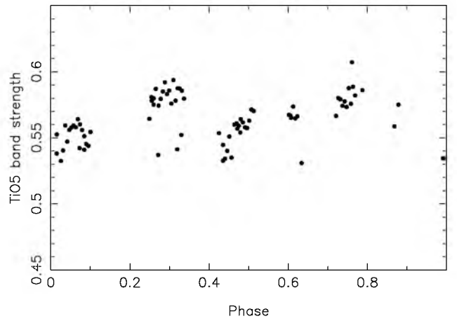
Figure 6. TiO5 band strength of the MDM spectra as a function of orbital phase. The uncertainty on each point is smaller than the symbol.
