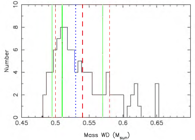
Figure 9. Distribution of the possible solutions for the mass of the white dwarf. The thick solid line (green/grey) is the most likely value that we have used. The thin solid lines (green/grey) are the values between which 68% of the possible solutions are located. The thick dashed line (red/darker grey) is the average value with the standard deviation in thin dashed lines (red/darker grey). The median of the distribution is shown as the dotted line (blue/dark grey)
