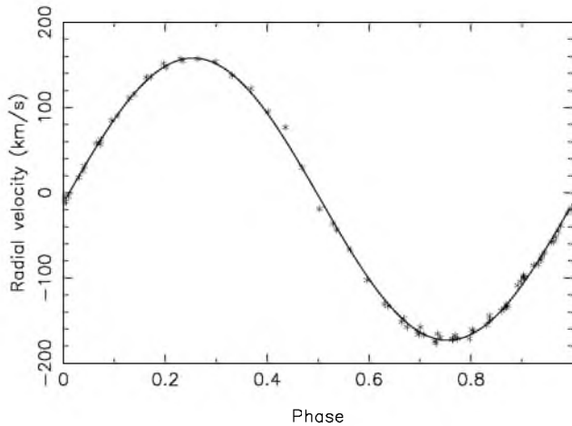
Figure 3. Radial velocity measurements for the H \alpha lines. The solid line is the best fit to these velocities, as discussed in Sect. 3.5. The uncertainties on the points are smaller than the symbols.
