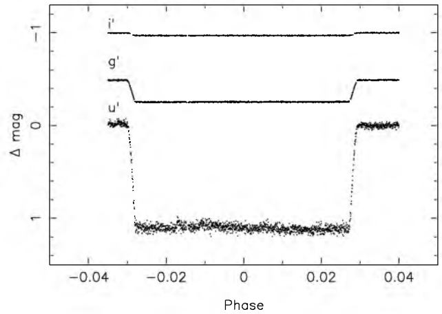
Figure 1. Primary eclipse observed with ULTRACAM.
