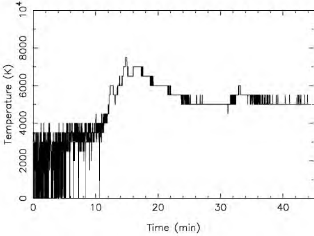
Figure 8. Temperature variation of the flaring area during the flaring period. The flaring area has a radius of 0.038R_{\odot} .
