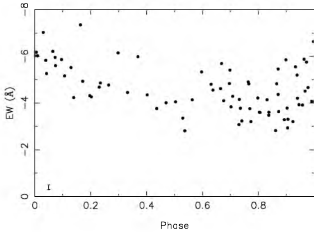
Figure 5. The equivalent width of the H\alpha line in the TLS spectra. The variations are folded on the orbital period of DE CVn. A typical error bar is shown in the bottom left corner.
