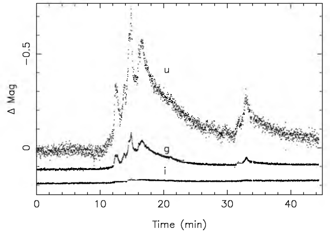
Figure 7. A flare of DE CVn observed with ULTRACAM.
