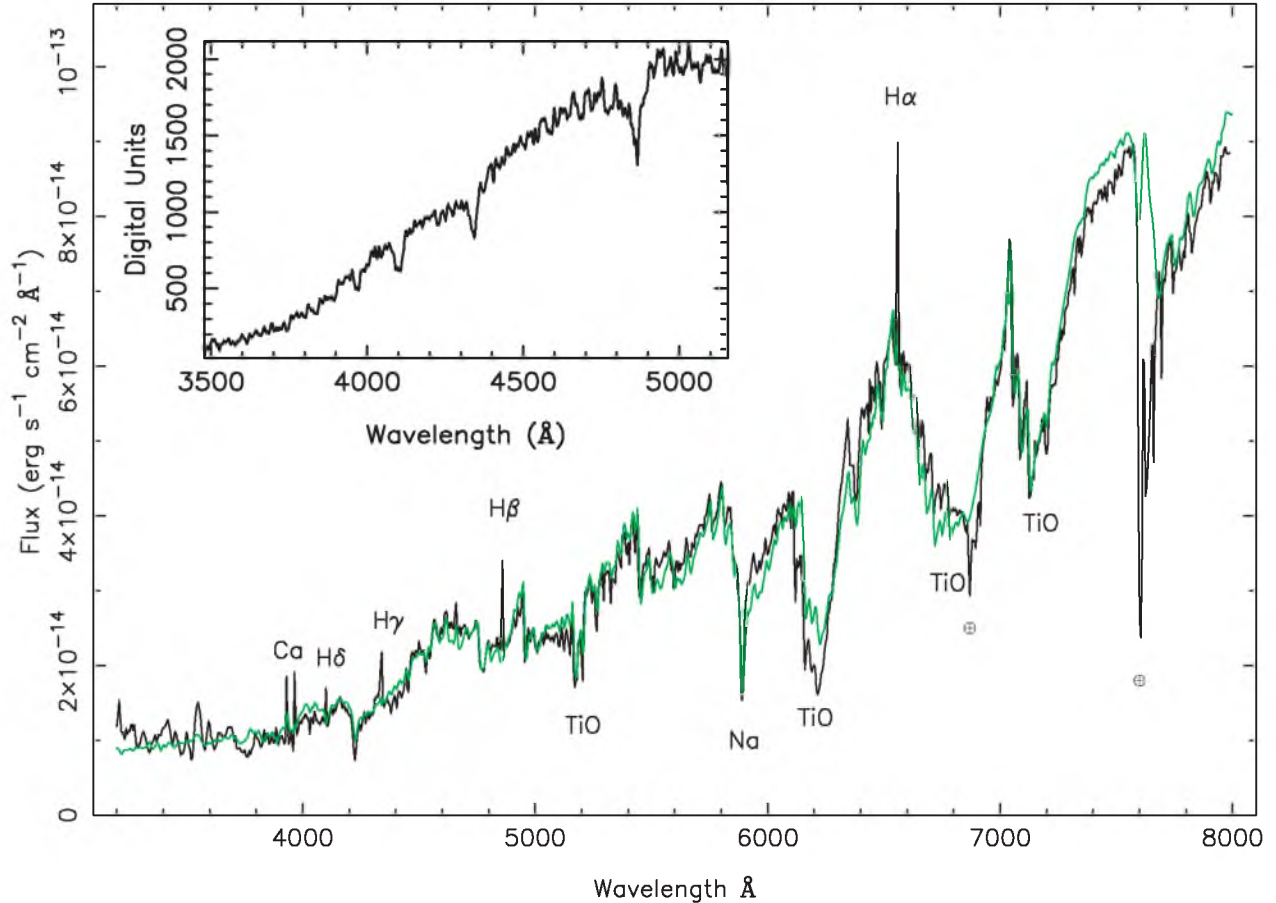
Figure 2. A combined ISIS spectrum of DE CVn (black line) together with a composite template of an M3V star from Pickles (1998) and a DA white dwarf with a temperature of 8000 K and \log g = 7.5 (grey/green line). Emission lines of H\alpha , H\beta , H\gamma and H\delta are visible in the spectrum as well as the Ca II H&K emission lines and the TiO absorption bands of the M dwarf. No spectral line signatures of the primary are visible. The difference between the in and out of eclipse spectra shows the underlying white dwarf which is plotted in the upper left corner.
