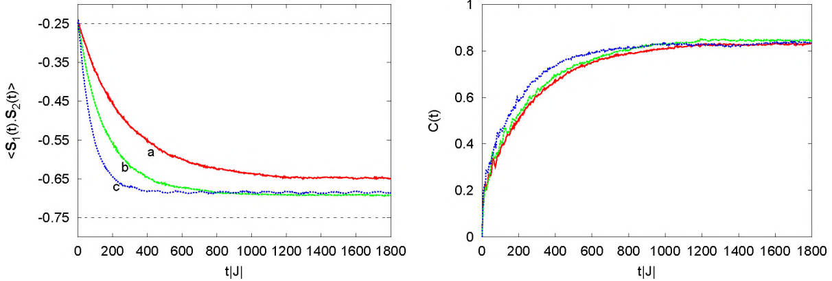
Fig. 1 (color online) Left: Time evolution of the correlation \langle \Psi(t) | \mathbf{S}_1 \cdot \mathbf{S}_2 | \Psi(t) \rangle of the two spins in the central system. Dashed horizontal line at -1/4 : Correlation in the initial state ( \langle \Psi(t=0) | \mathbf{S}_1 \cdot \mathbf{S}_2 | \Psi(t=0) \rangle = -1/4 ); Horizontal line at -3/4 : Expectation value in the singlet state; (a) Environment containing N = 14 quantum spins; (b) N = 16 ; (c) N = 18 . The parameters \Omega_{i,j}^{(\alpha)} and \Delta_{i,j}^{(\alpha)} are uniform random numbers in the range [-0.15|J|, 0.15|J|] . Right: Time evolution of the concurrence C(t) for three different random realizations of a spin glass environment. The parameters are uniform random numbers in the range -0.15|J| \leq \Omega_{i,j}^{(\alpha)}, \Delta_{i,j}^{(\alpha)} \leq 0.15|J| and the environment contains N = 14 quantum spins. The transition from an unentangled state ( C(t) = 0 ) to a nearly fully entangled state ( C(t) = 1 ) is clearly seen.
