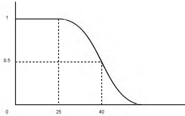
Figure 9: Membership function for young
