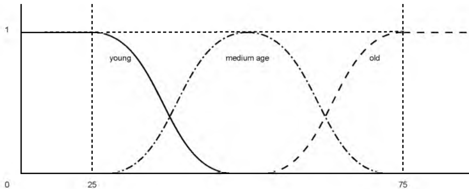
Figure 10: The linguistic variable Age
