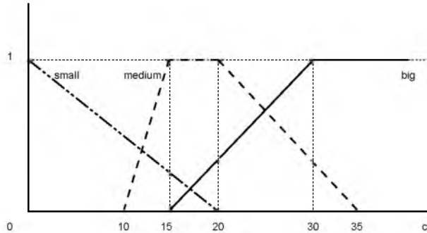
Figure 12: Probability profile for the values of the linguistic variable ‘volume’
