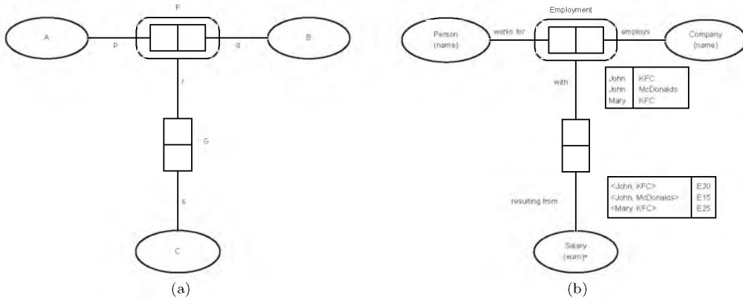
Figure 5: Example: information structure and names
