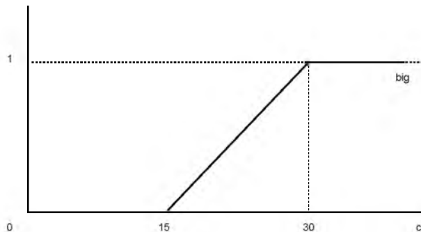
Figure 11: Probability profile for linguistic value 'big'
