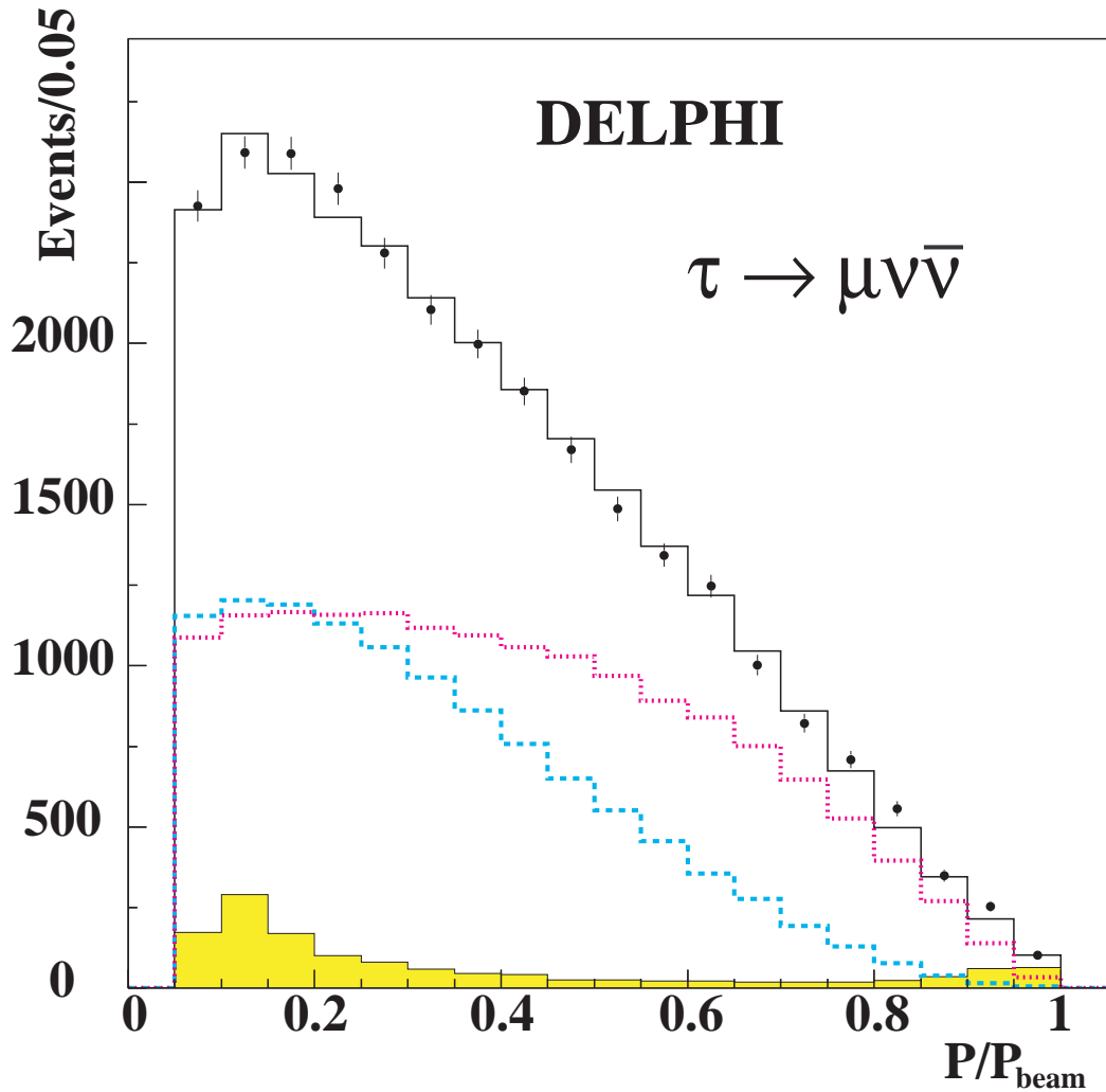
Figure 4.6: The measured spectrum of the polarisation-sensitive variable for the \tau \rightarrow \mu\nu\bar{\nu} decays in the DELPHI experiment. The variable is the ratio of the measured muon momentum to the beam energy, which is an approximation of x_\mu = E_\mu/E_\tau . The data are compared to the results of the polarisation fit. The points with error bars are data and the solid line is simulated data for the fitted values of \mathcal{A}_\tau and \mathcal{A}_e . The shaded area is background and the dashed and dotted lines correspond to the positive and negative helicity contributions respectively.
