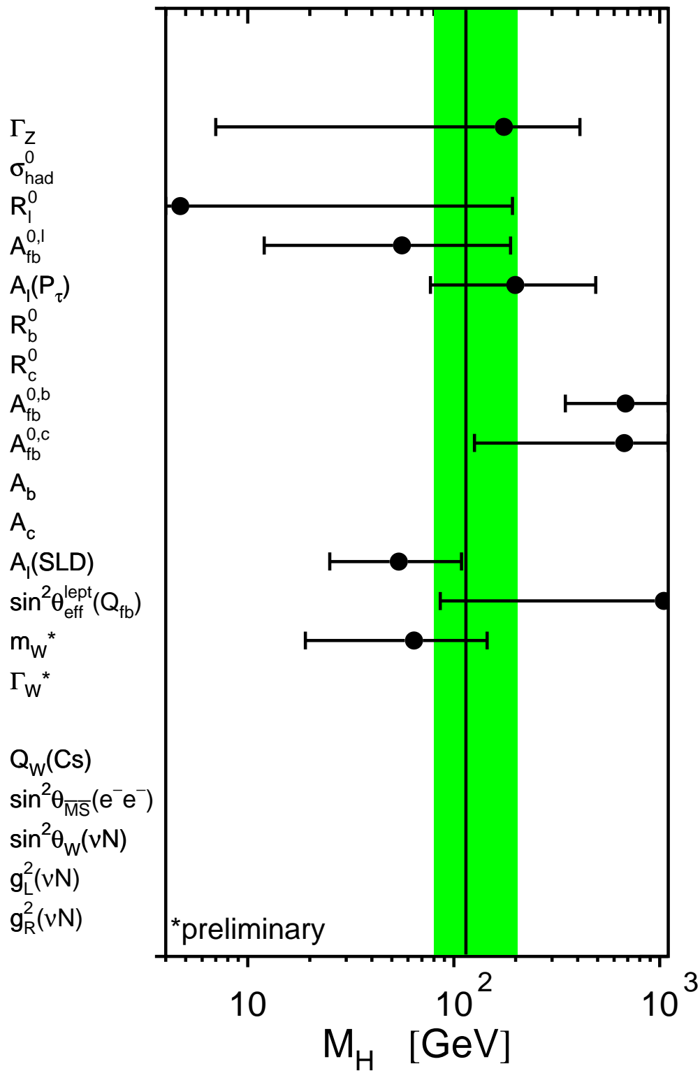
Figure 8.15: Constraints on the mass of the Higgs boson from each pseudo-observable. The Higgs-boson mass and its 68% CL uncertainty is obtained from a five-parameter SM fit to the observable, constraining \Delta\alpha_{\text{had}}^{(5)}(m_Z^2) = 0.02758 \pm 0.00035 , \alpha_S(m_Z^2) = 0.118 \pm 0.003 , m_Z = 91.1875 \pm 0.0021 GeV and Tevatron Run-I m_t = 178.0 \pm 4.3 GeV. Only significant constraints are shown. Because of these four common constraints the resulting Higgs-boson mass values cannot be combined. The shaded band denotes the overall constraint on the mass of the Higgs boson derived from all pseudo-observables reported in Table 8.3. The direct measurements of m_W and \Gamma_W used in that analysis are preliminary.
