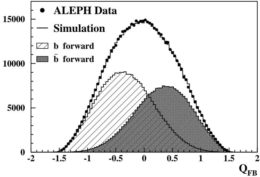
Figure 5.12: Charge separation of the ALEPH neural net tag using jet charge, vertex charge and charged kaons [142]. The asymmetry reflects A_{\text{FB}}^{b\bar{b}} diluted by the non-perfect charge tagging.
