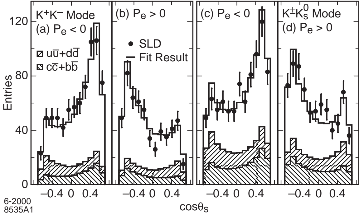
Figure F.2: Measured s -quark polar angle distributions (dots) for selected SLD events in the (a),(b) K^+K^- and (c),(d) K^\pm K_S^0 modes, produced with (a),(c) left- and (b),(d) right-polarised electron beams. The histograms represent the result of a simultaneous fit to the four distributions, and the upper (lower) hatched areas indicate the estimated u\bar{u}+d\bar{d} ( c\bar{c}+b\bar{b} ) backgrounds.
