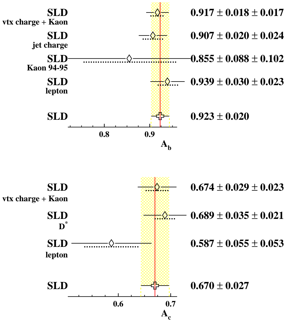
Figure 5.15: A_b and A_c measurements used in the heavy flavour combination, corrected for their dependence on parameters evaluated in the multi-parameter fit described in the text. The dotted lines indicate the size of the systematic error.
