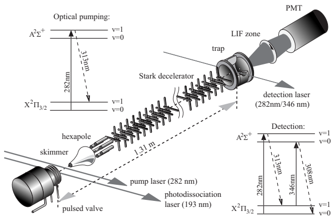
FIG. 1: Scheme of the experimental setup. A pulsed beam of OH ( v = 0 ) radicals is produced via photodissociation (193 nm) of \text{HNO}_3 molecules seeded in Xe. Prior to entering the decelerator, part of the OH radicals are prepared in the v = 1 state by Franck-Condon pumping via the A^2\Sigma^+ state (upper left). OH radicals in the J = 3/2 level of both the v = 0 and v = 1 vibrational states of the X^2\Pi_{3/2} electronic ground state are Stark decelerated and subsequently loaded into the electrostatic trap. Molecules in the trap are state-selectively detected by imaging the laser induced fluorescence onto a PMT.
