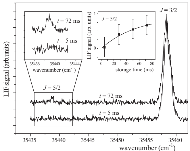
FIG. 3: Excitation spectrum of trapped OH ( v = 0 ) radicals that is recorded 5 ms (lower curve) and 72 ms (upper curve) after switching on of the trap. In the central inset, the population of trapped OH radicals in the v = 0, J = 5/2 level is shown as a function of the storage time.
