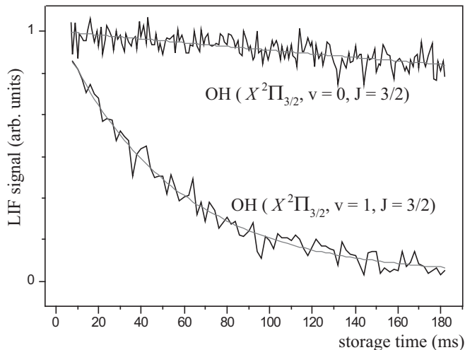
FIG. 2: Population of trapped OH radicals in the X^2\Pi_{3/2}, v = 0, J = 3/2 level (upper curve) and in the X^2\Pi_{3/2}, v = 1, J = 3/2 level (lower curve), as a function of the storage time t . The trapping potential is switched on at t = 0 ms.
