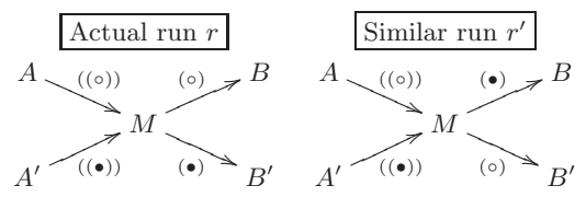
Figure 1: Onion Routing
