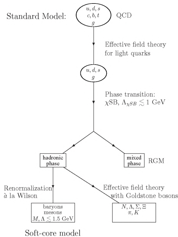
Figure 1: Overview of the theoretical basis for the soft-core meson-baryon interactions.
