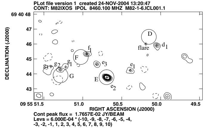
Fig. 1. Map of M 82 around the ULXs D and F (see Table 4). The brightest radio source in the field is e_2 which is coincident with the X-ray point source E. The FWHM of all X-ray point sources has been set to 1'' . Even though the radio source d_1 is outside of the r = 0.5'' circle for ULX D, its offset ( 0.77'' ) is consistent with the ULX X-ray position.
