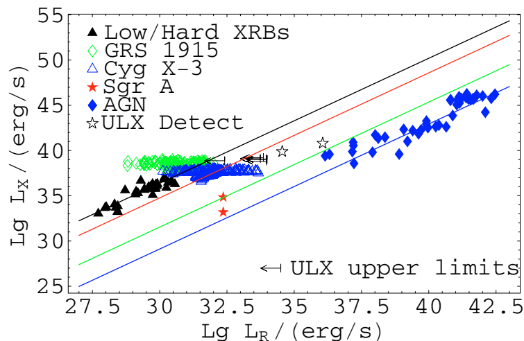
Fig. 3. The upper limits of the ULXs with respect to the low/hard state XRB and AGN population. The lines correspond to different black hole masses. From top to bottom 6, 6 \times 10^2, 6 \times 10^6, 6 \times 10^9 M_{\odot} . The left ULX radio detection represents NGC 5408, while the right is the radio flare in M 82. The correlation should not hold for fares; this was just plotted for comparison. As GRS 1915 and Cyg X-3 are both radio transients, they are not expected to follow the correlation.
