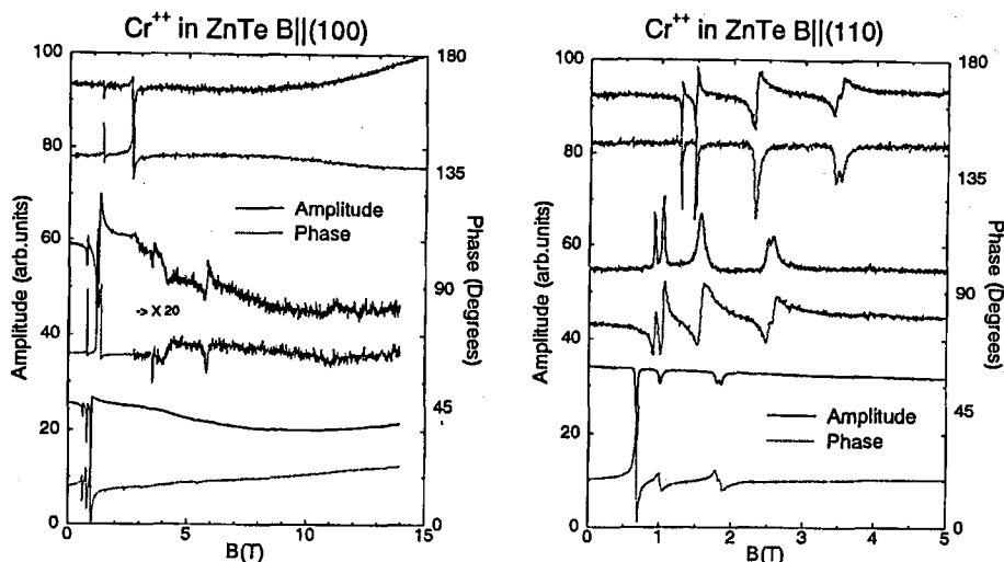
Fig. 1. Some representative MVNA absorption spectra for B \parallel (100) (left) and B \parallel (110) (right). The spectra were taken at T = 1.2 K for frequencies 149, 100, 89 GHz (left, top to bottom) and 138, 110, 87 GHz (right, top to bottom).
