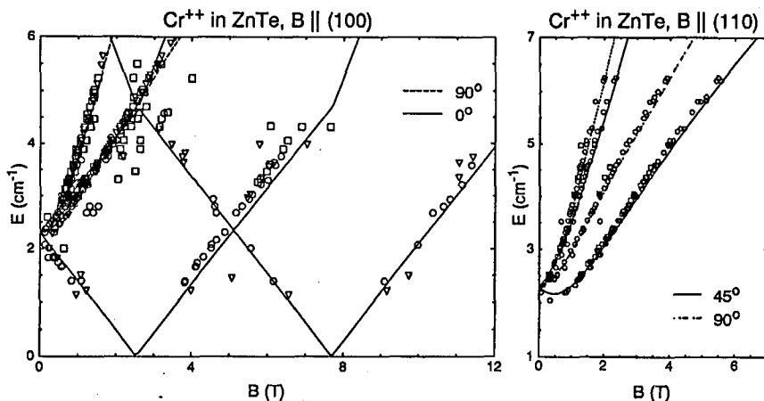
Fig. 2. Transition energy versus magnetic field for B \parallel (100) (left) and B \parallel (110) (right). \square and \nabla are data taken on sample 2642, \circ on sample 2720. The results of the model calculations (as described in the text) are plotted by solid and dashed lines.
