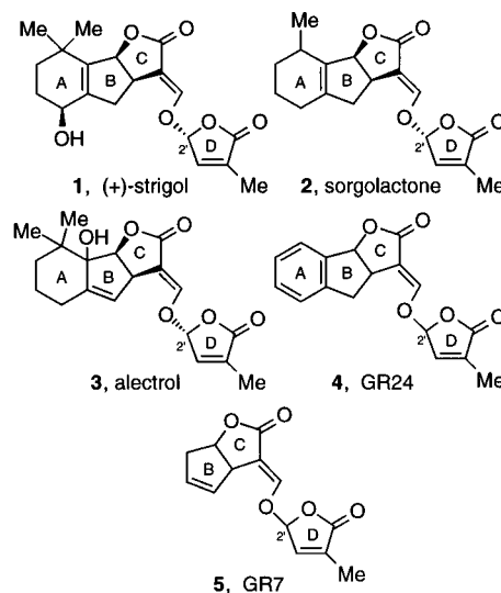
Figure 1. Structures of strigolactones 1–3 and analogues 4 and 5 .
