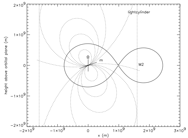
Fig. 1. The Binary System AE Aquarii. Shown are the system Roche Lobes, the orientation of the spin axis (here vertical), the position of the light cylinder, and the position of the magnetic dipole axis as it passes the plain of the drawing. Also shown are some of the unperturbed dipolar field lines including the last closed field lines and the two field lines which would pass through the inner Lagrangian point at the epoch represented and, respectively, half a spin period later.
