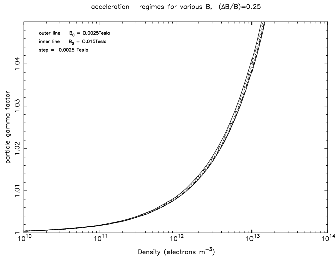
Fig. 6. The low energy end of Fig. 5.
