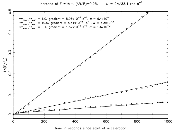
Fig. 2. The increase of energy with time by homogeneous magnetic pumping in the non-relativistic regime, for 3 values of the pitch-angle scattering to field oscillation time. The straight lines are fits to the numerical data, given by the points. \alpha is calculated given the field parameters indicated.
