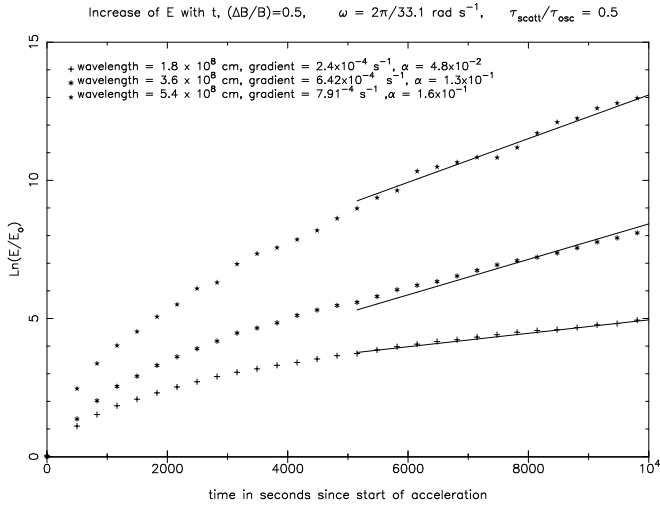
Fig. 4. The increase of energy with time of particles accelerated by travelling magnetic compressions.
