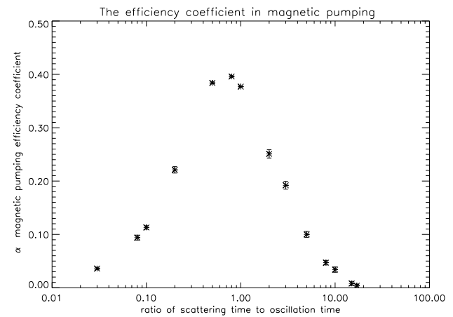
Fig. 3. The parameter \alpha as a function of the ratio of pitch-angle scattering time to field oscillation time.
