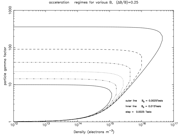
Fig. 5. Allowed acceleration regimes for \tau_{scatt}/\tau_{osc} = 1 and various field strengths (0.0025 – 0.015 T). A net acceleration will occur in the regions inside the curves.
