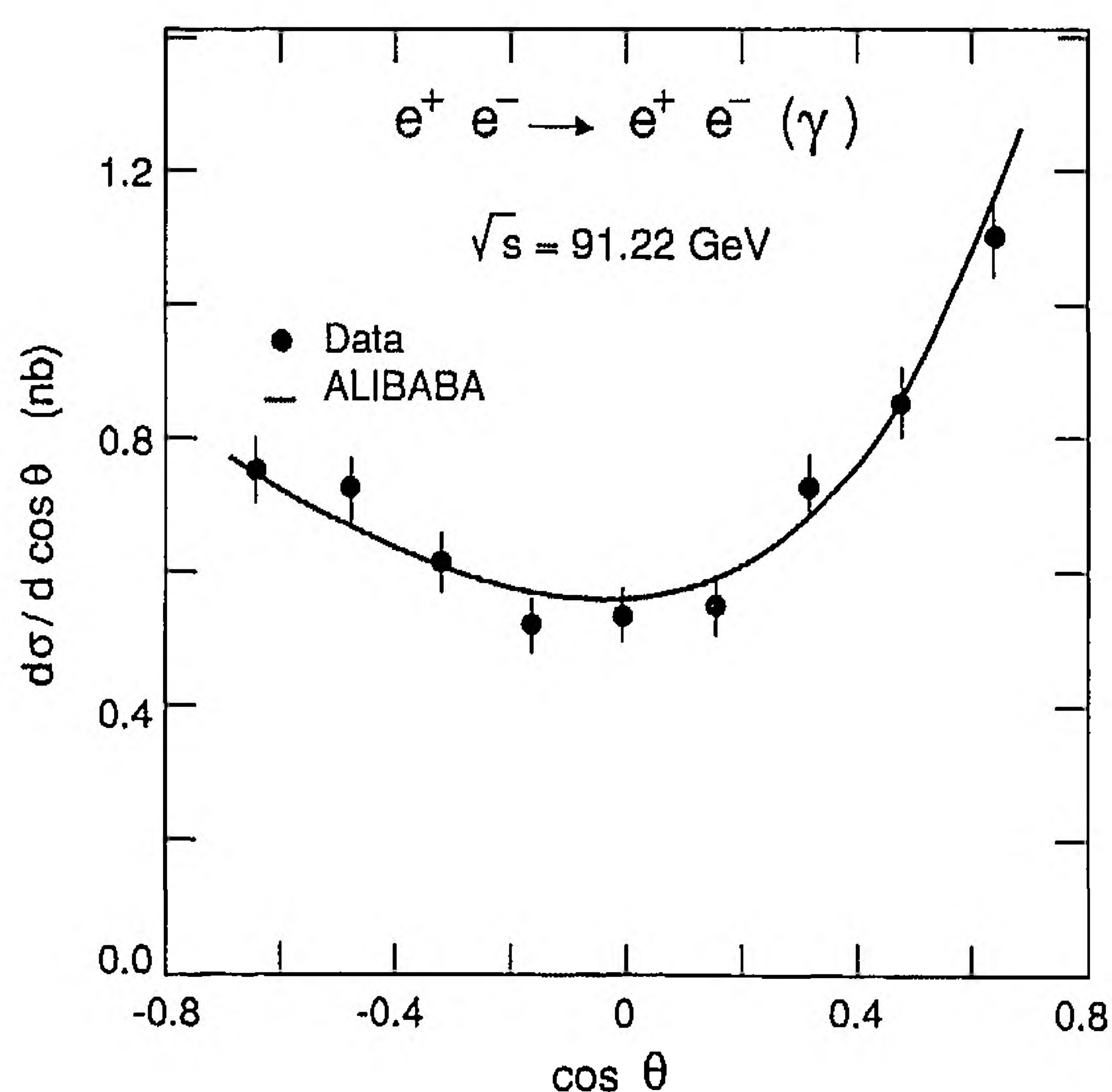
Fig. 15. Acceptance corrected \cos \theta distribution for e^+e^- \rightarrow e^+e^- (\gamma) events at the Z^0 peak. The solid line corresponds to a Standard Model prediction obtained from ALIBABA, adapted to the fit results given in Table 11
