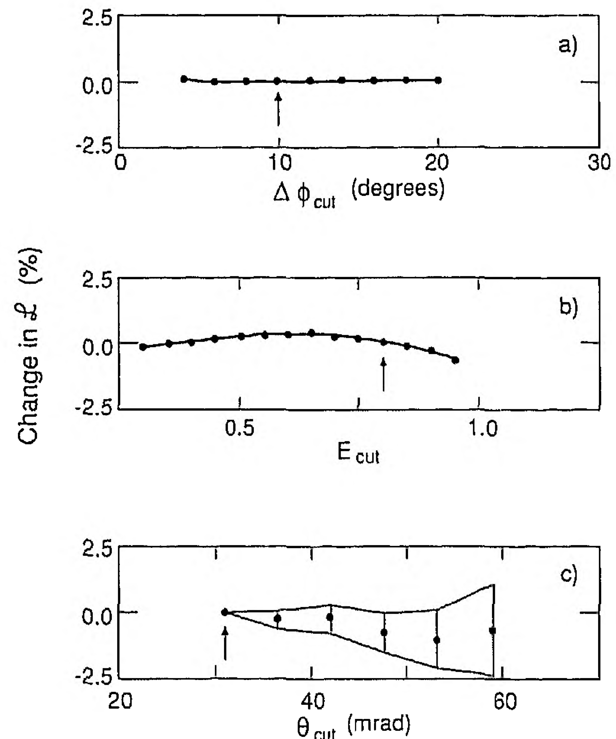
Fig. 2a-c. The relative change in the integrated luminosity as a function of a the coplanarity cut, |\Delta\phi - 180^\circ| < \Delta\phi_{\text{cut}} ; b the energy cut, one energy larger than E_{\text{cut}} E_{\text{beam}} and the other energy larger than \frac{1}{2} E_{\text{cut}} E_{\text{beam}} ; and c the tight fiducial volume cut, \theta_{\text{cut}} < \theta < 64.41 mrad. The shaded region in Fig. c indicates the statistical uncertainty (dominated by the Monte Carlo simulation) with respect to the nominal cut value. These nominal cut values are indicated by the arrows
