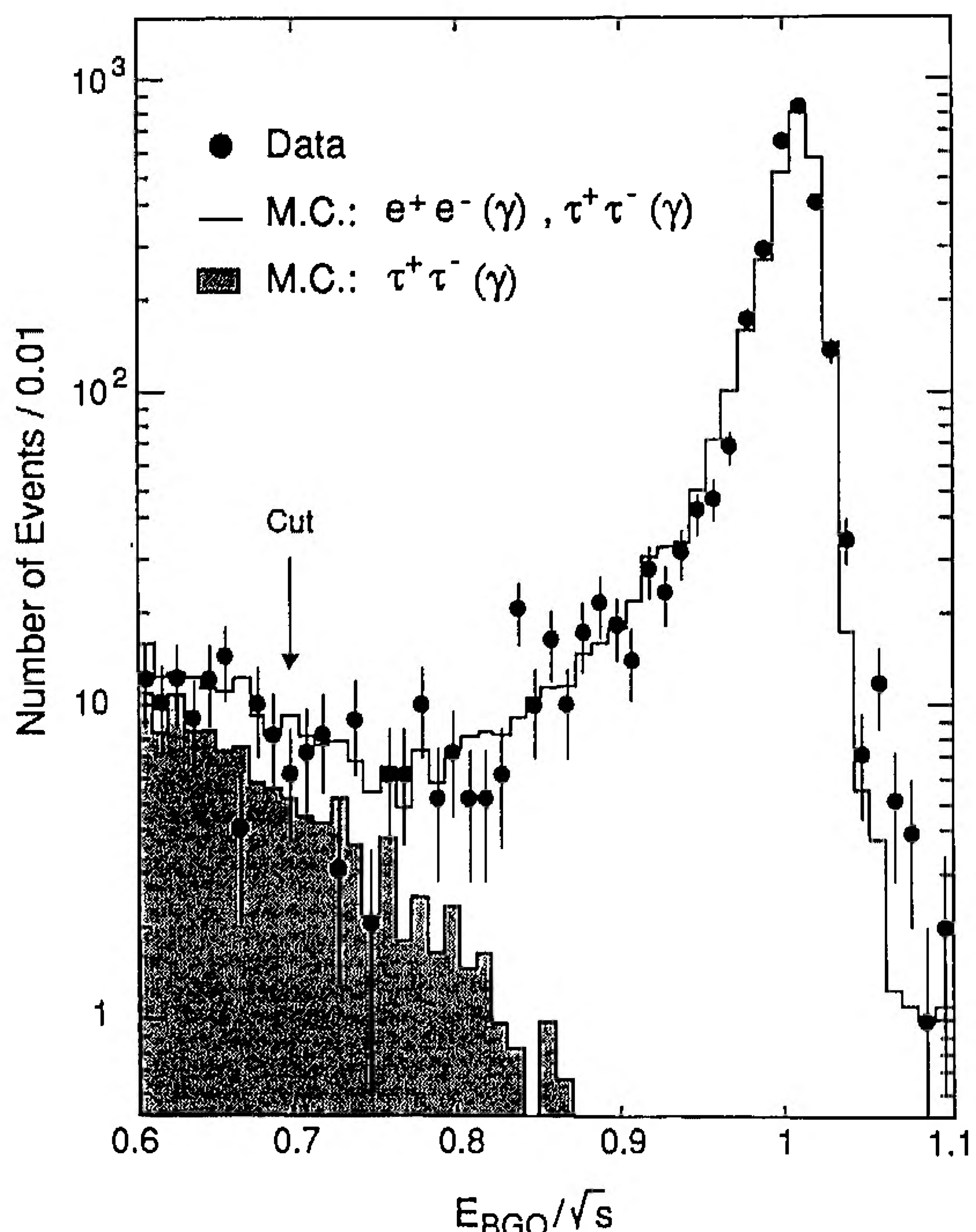
Fig. 11. The total energy distribution in the BGO calorimeter normalized to the center of mass energy for e^+e^- \rightarrow e^+e^- (\gamma) events. The distribution is compared with the Monte Carlo simulation, including the simulation of the e^+e^- \rightarrow \tau^+\tau^- (\gamma) background. In this figure all event selection cuts are imposed, except the cut on the variable plotted
