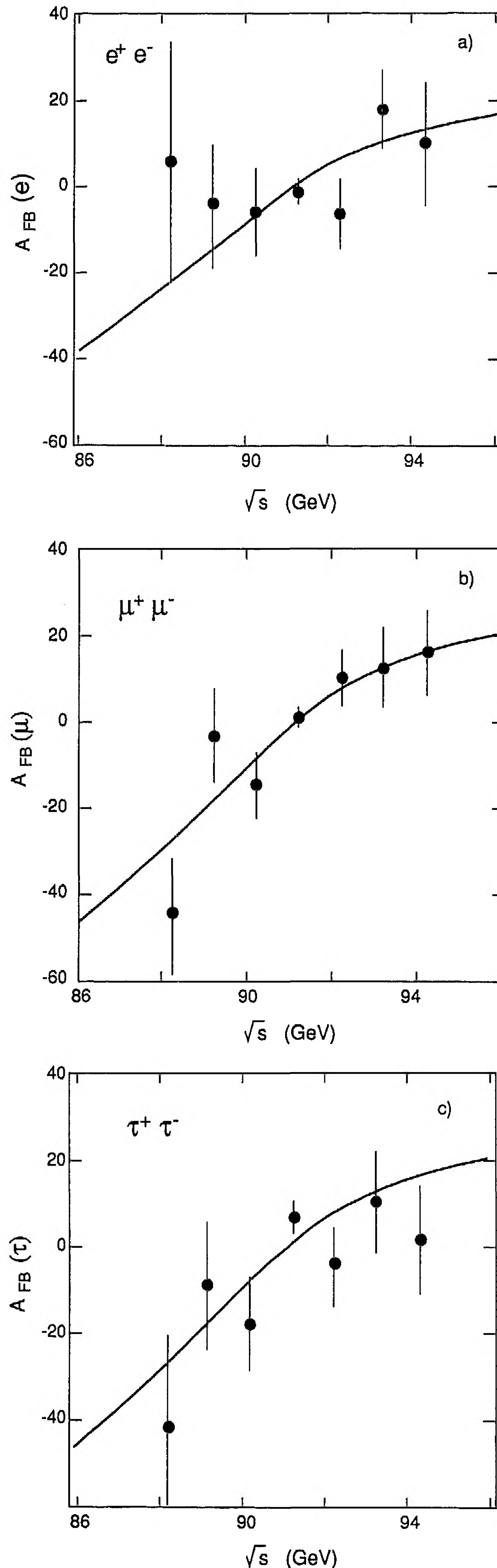
Fig. 19a-c. The forward-backward asymmetry for a e^+e^- \rightarrow e^+e^- in the 44^\circ < \theta < 136^\circ angular range and with \zeta < 25^\circ , b e^+e^- \rightarrow \mu^+\mu^- , and c e^+e^- \rightarrow \tau^+\tau^- events as a function of \sqrt{s} . The solid curves represent the fit with the parameters given in Table 13
