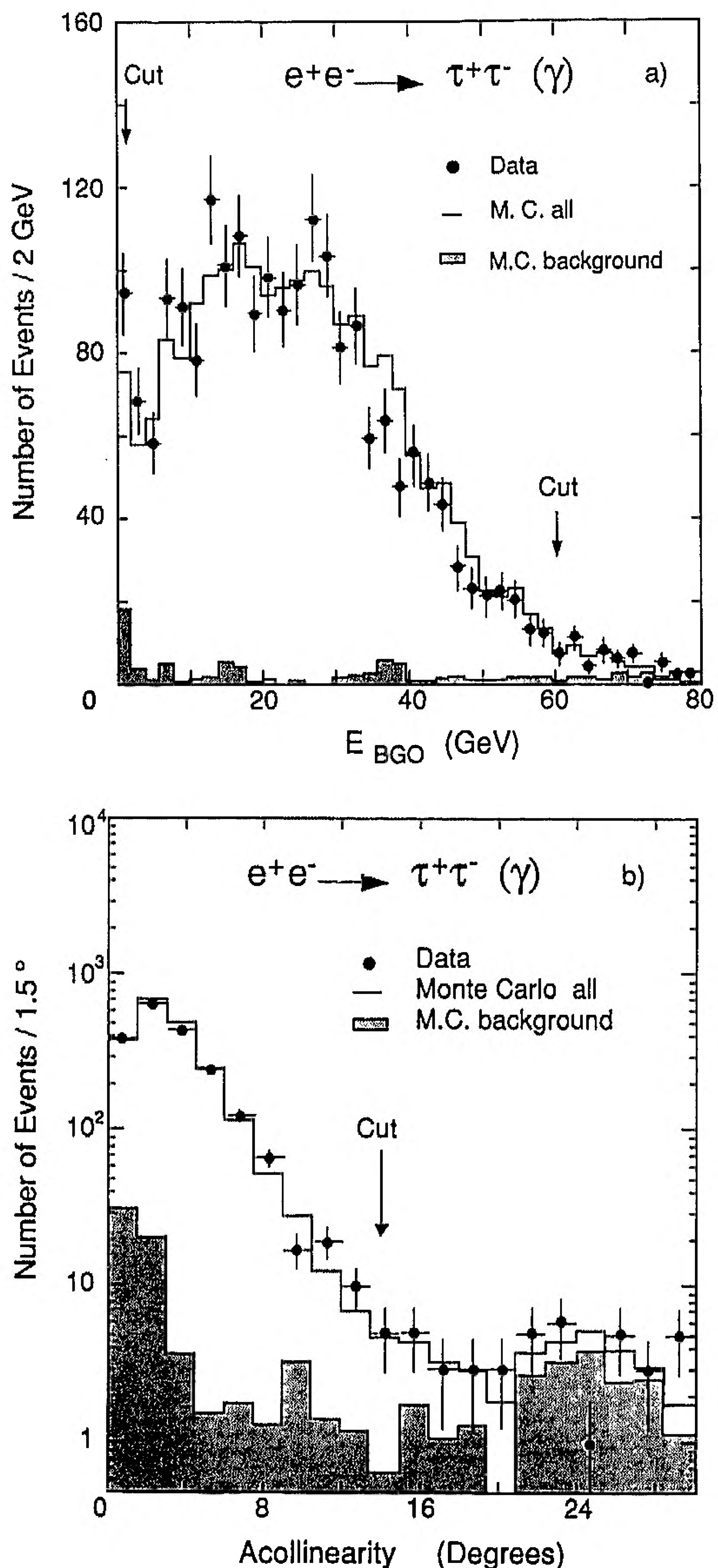
Fig. 9a, b. a The distribution of the energy deposited in the BGO calorimeter and b the distribution of the acollinearity for e^+e^- \rightarrow \tau^+\tau^- (\gamma) events. Both distributions are compared to the Monte Carlo simulations, including background simulations for e^+e^- \rightarrow e^+e^- (\gamma) , e^+e^- \rightarrow \mu^+\mu^- (\gamma) and e^+e^- \rightarrow \text{hadrons} . In these figures all event selection cuts are imposed, except the cut on the variable plotted
