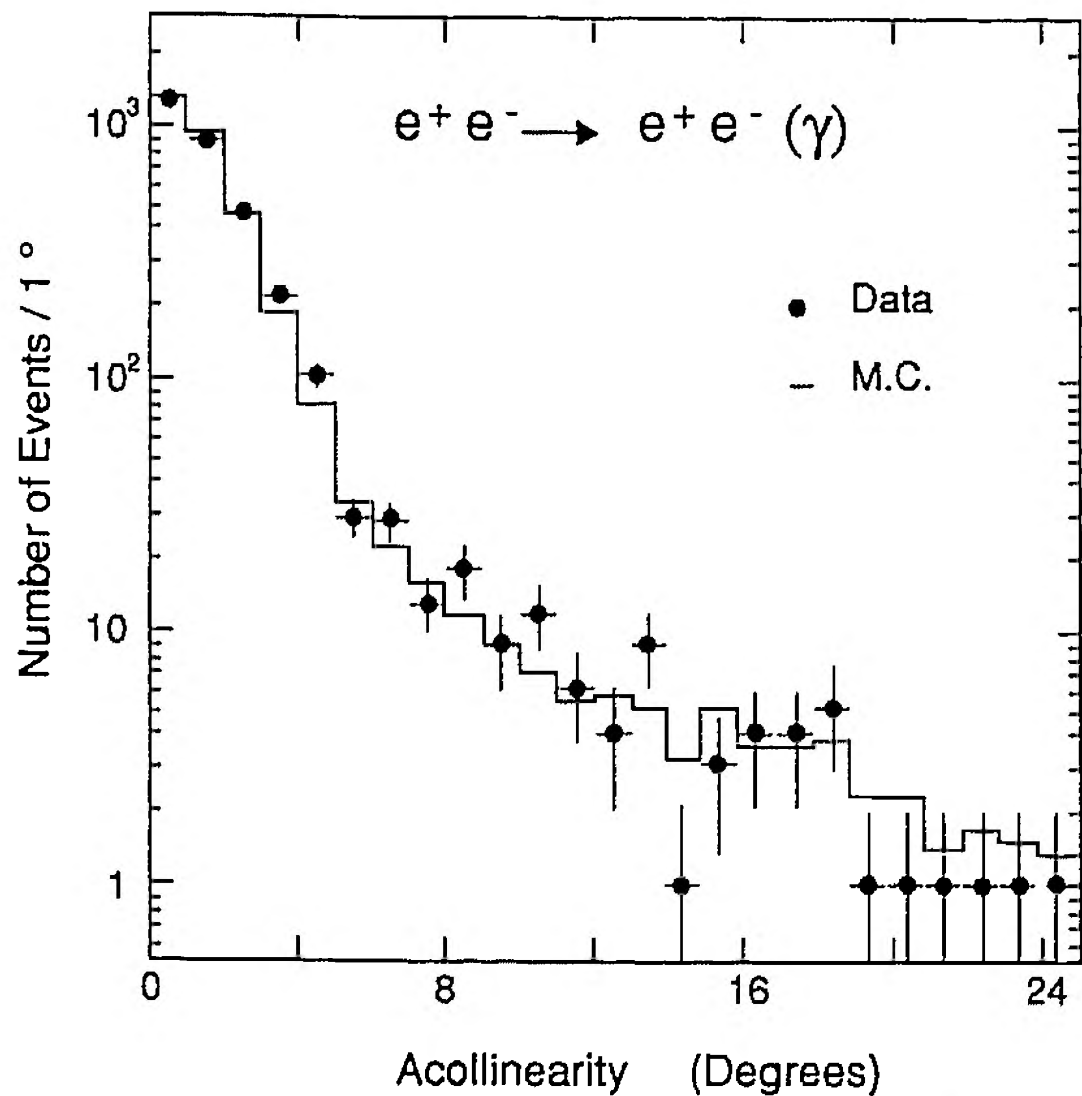
Fig. 12. Acolinearity distribution for e^+e^- \rightarrow e^+e^-(\gamma) events compared to the Monte Carlo simulation
