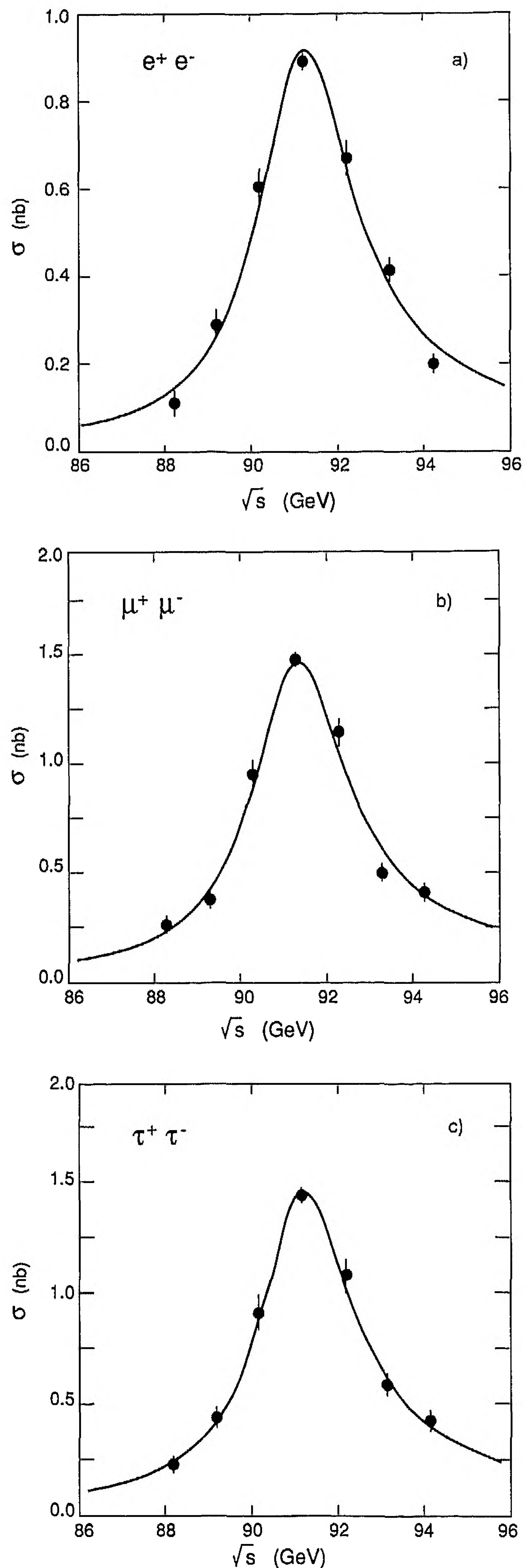
Fig. 18a-c. a The s -channel cross section in the angular range 44^\circ < \theta < 136^\circ and with \zeta < 25^\circ for e^+e^- \rightarrow e^+e^- , b the cross section for e^+e^- \rightarrow \mu^+\mu^- , corrected for geometrical acceptance, and c the cross section for e^+e^- \rightarrow \tau^+\tau^- , corrected for geometrical acceptance, as a function of \sqrt{s} . The solid curves are the results of the four-parameter fit (Table 11) assuming lepton universality
