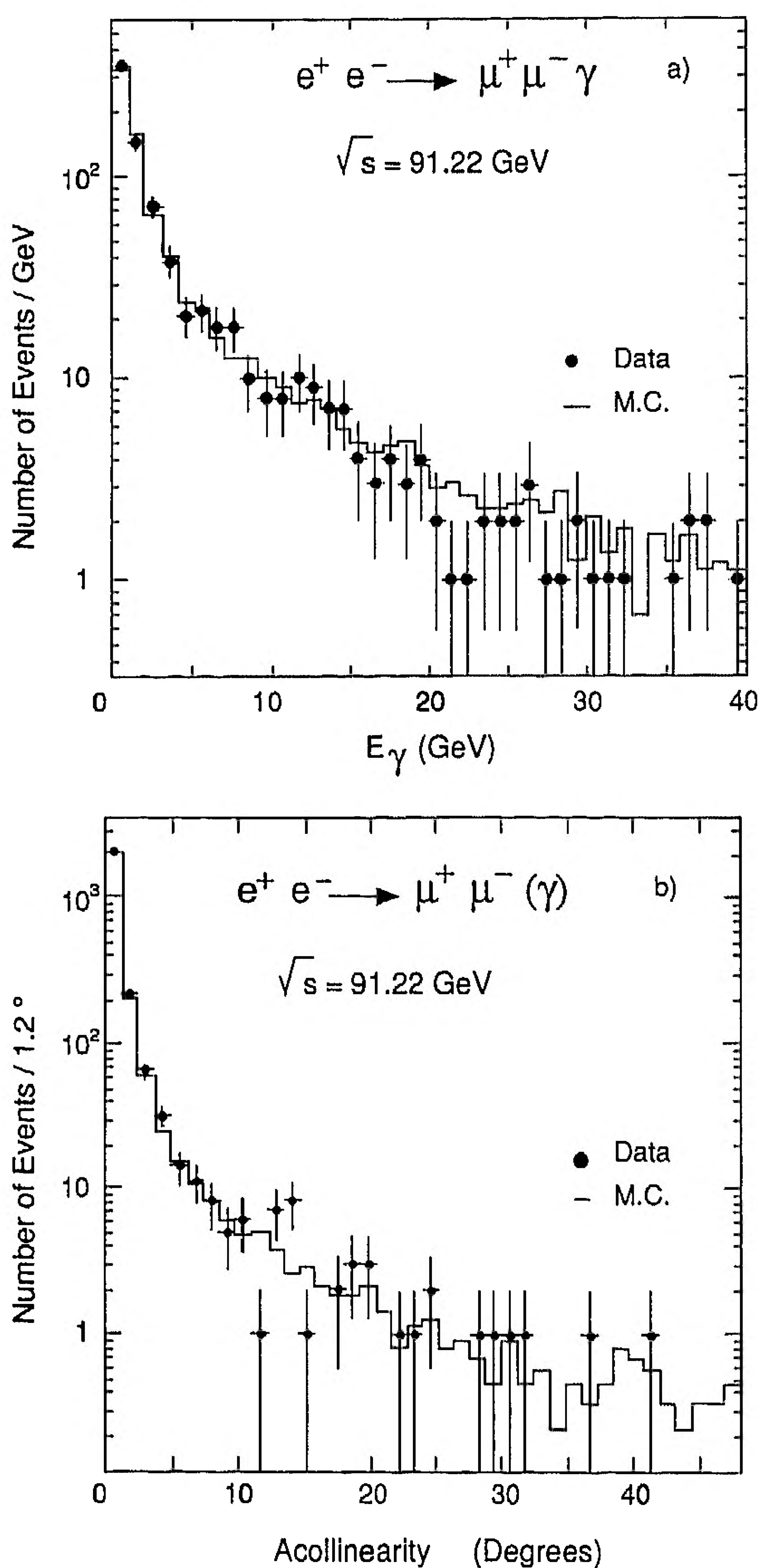
Fig. 7a, b. a The photon energy spectrum for e^+e^- \rightarrow \mu^+\mu^- (\gamma) events and b the acollinearity distribution for e^+e^- \rightarrow \mu^+\mu^- (\gamma) events. Both distributions are compared to the Monte Carlo simulations
