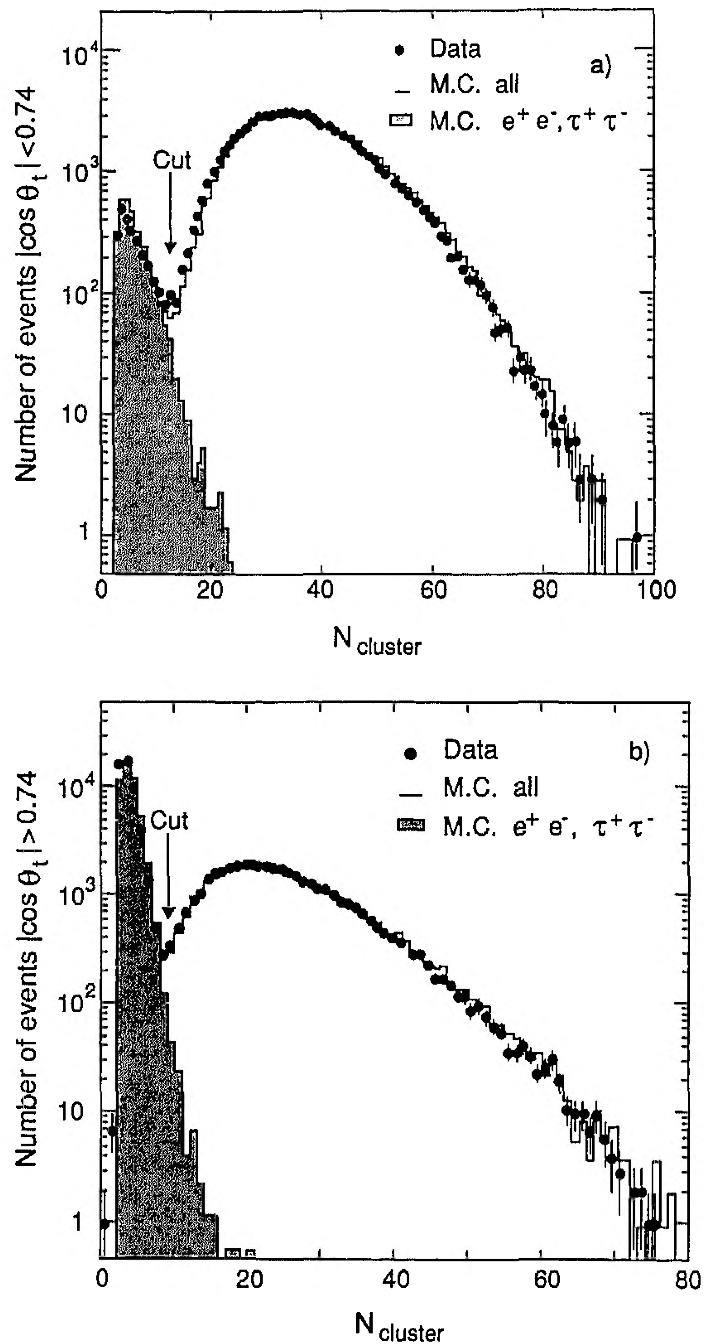
Fig. 5a, b. Number of clusters reconstructed in the calorimeters for hadronic events with a |\cos \theta_t| < 0.74 and b |\cos \theta_t| > 0.74 , are compared with the same distributions for Monte Carlo signal and background events. In these figures all event selection cuts are imposed, except the cut on the variable plotted
