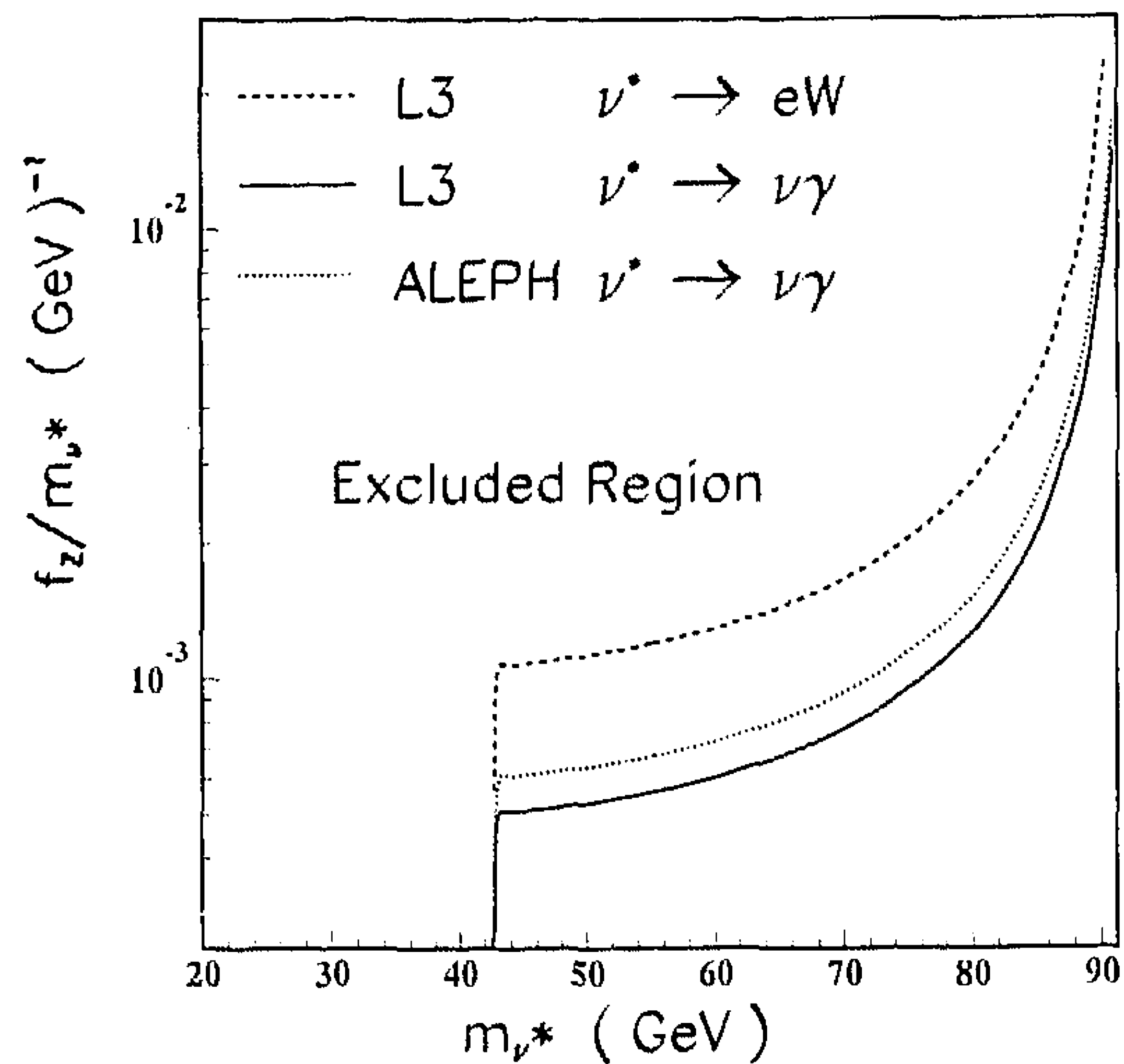
Fig. 3. The upper limit of the coupling constant f_2/m_{\nu^*} at 95% CL as a function of m_{\nu^*} for both \nu^* \rightarrow eW and \nu^* \rightarrow \nu\gamma decays from L3. The upper limit for \nu^* \rightarrow \nu\gamma from ALEPH is also shown. The excluded region is above and left of the curves.
