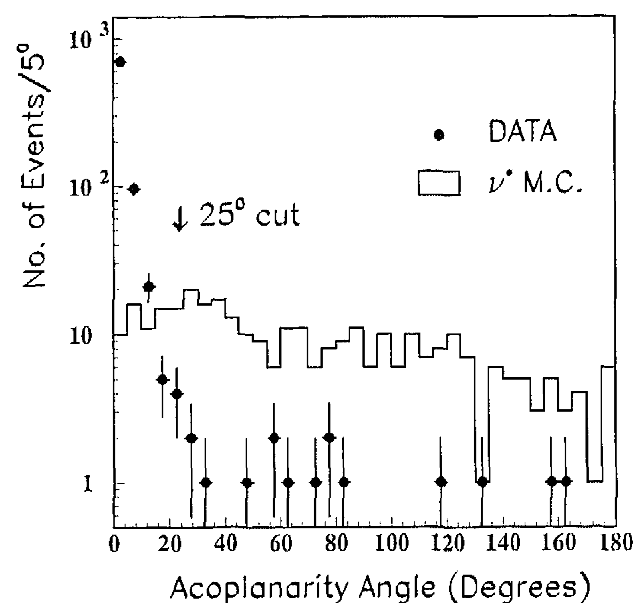
Fig. 1. The acoplanarity angle of the two jets for data and \nu^* Monte Carlo with m_{\nu^*} = 70 \text{ GeV} .
