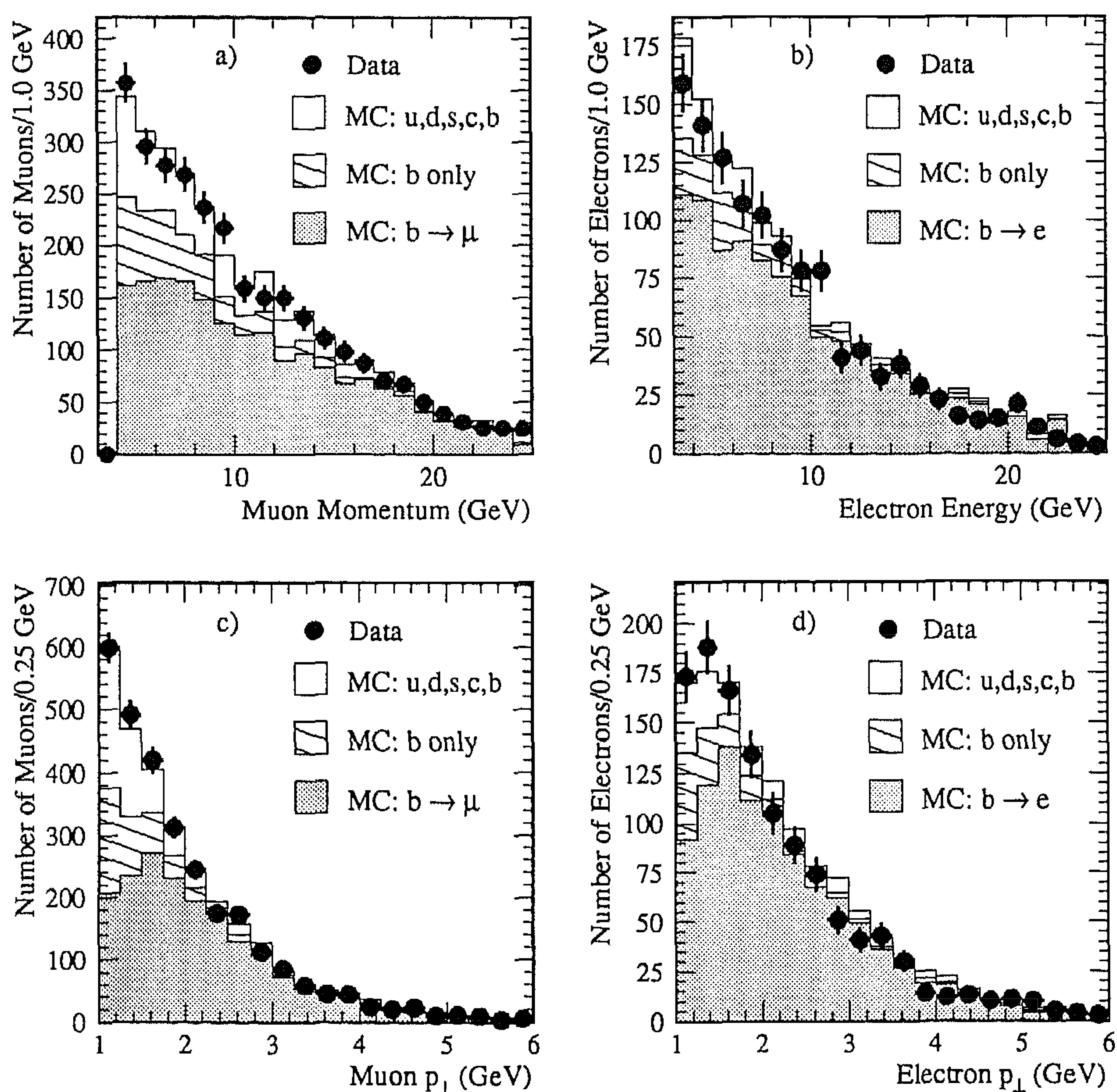
Fig. 1. Measured momentum and transverse momentum spectra for muons (a), (c) and electrons (b), (d) after cuts. The expected contribution from prompt b-decay, b-quarks only, and background is indicated.
