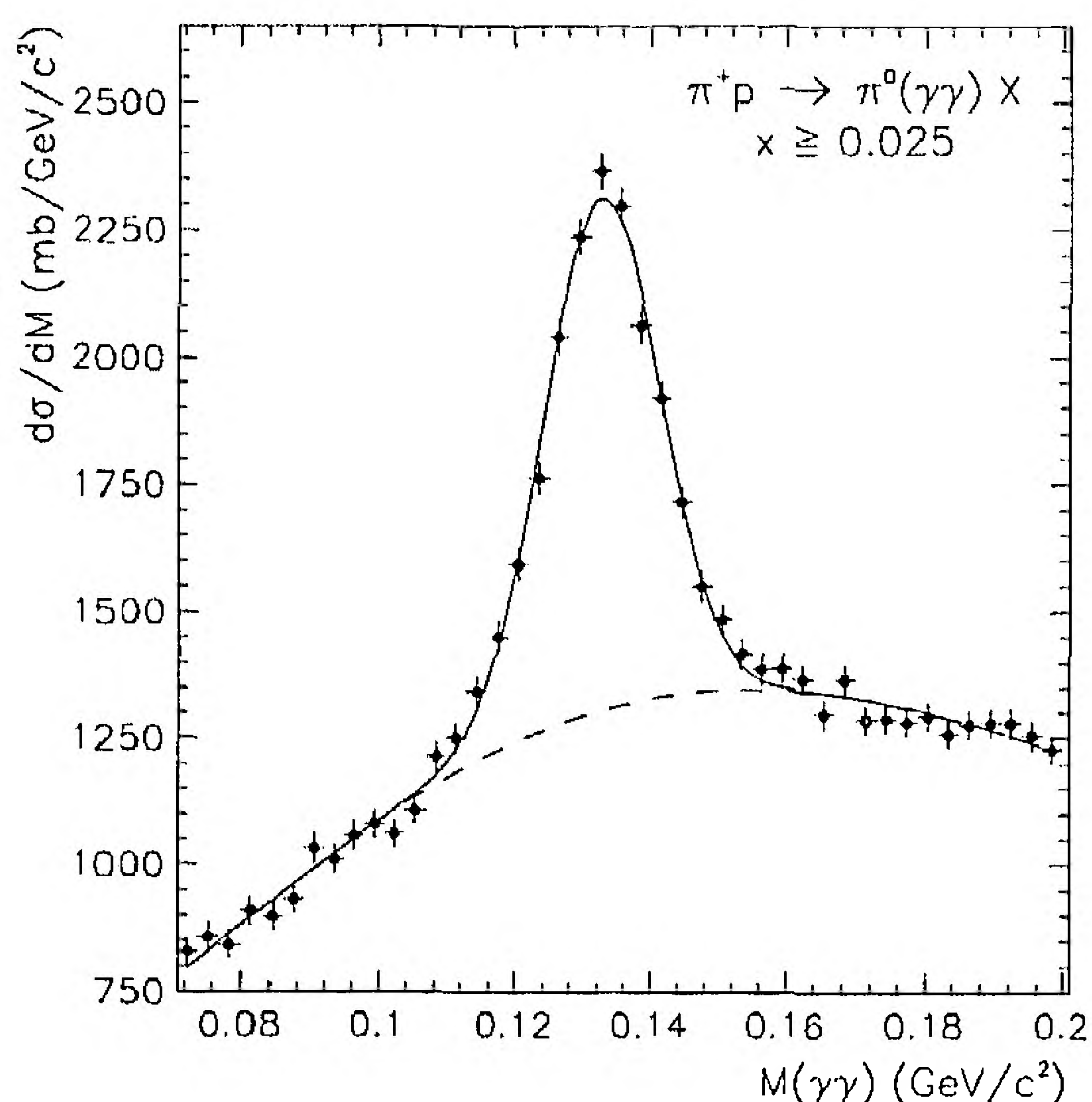
Fig. 1. Weighted \gamma\gamma invariant mass distribution with x(\gamma\gamma) \geq 0.025 for \pi^+p interactions at 250 GeV/c. The curves show the result of the fit described in the text
