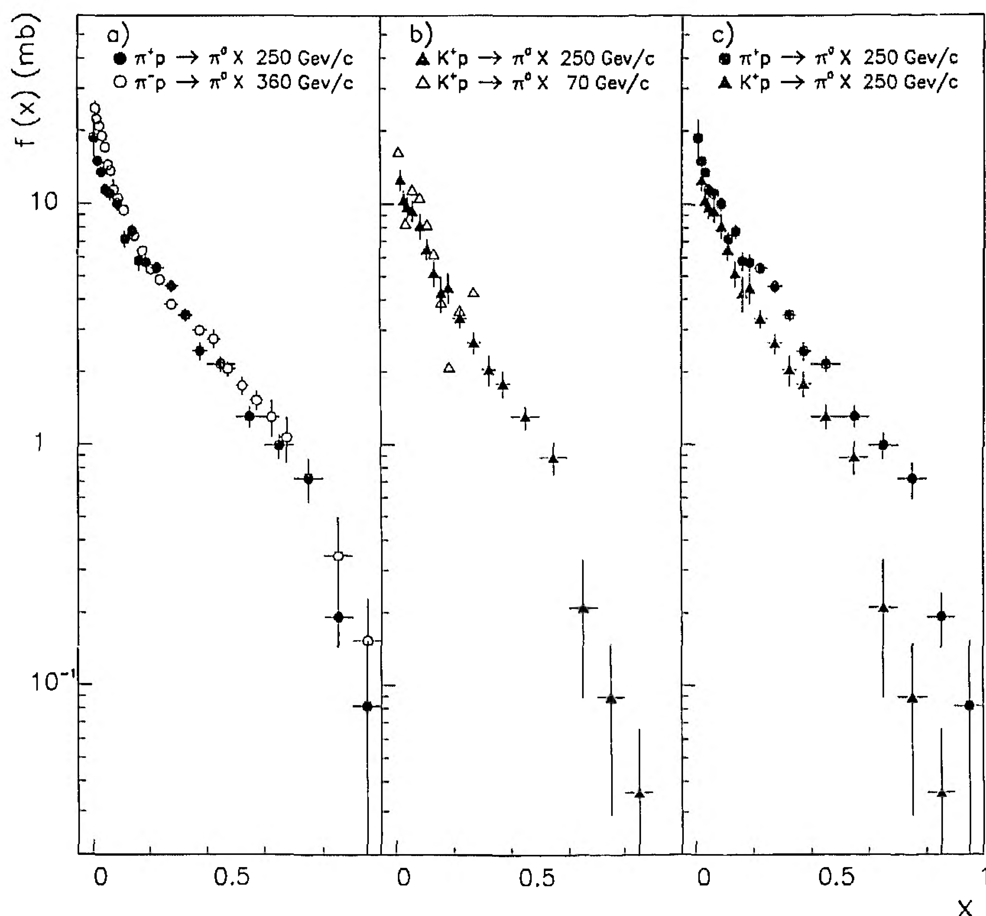
Fig. 5a-c. The invariant f(x) distributions for a \pi^+p at 250 GeV/c and \pi^-p at 360 GeV/c [23]; b K^+p at 70 [16] and 250 GeV/c; c \pi^+p and K^+p at 250 GeV/c
