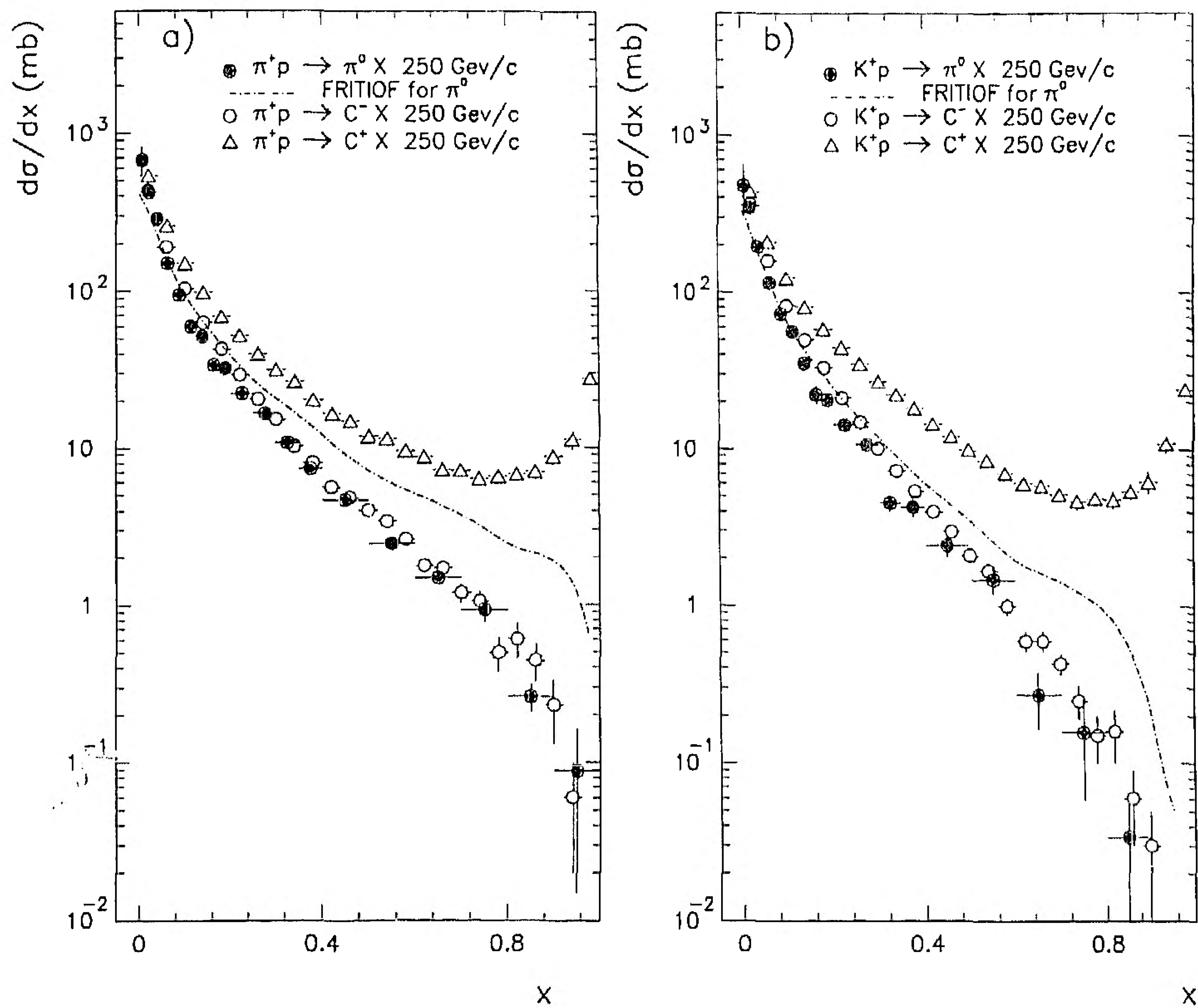
Fig. 4a, b. The d\sigma/dx distribution compared with the prediction of the FRITIOF model (dashed-dotted curve) and the corresponding data for reactions \pi^+p \rightarrow C^+ + X and \pi^+p \rightarrow C^- + X at 250 GeV/c [22] a for \pi^+p interactions at 250 GeV/c, b for K^+p interactions at 250 GeV/c
