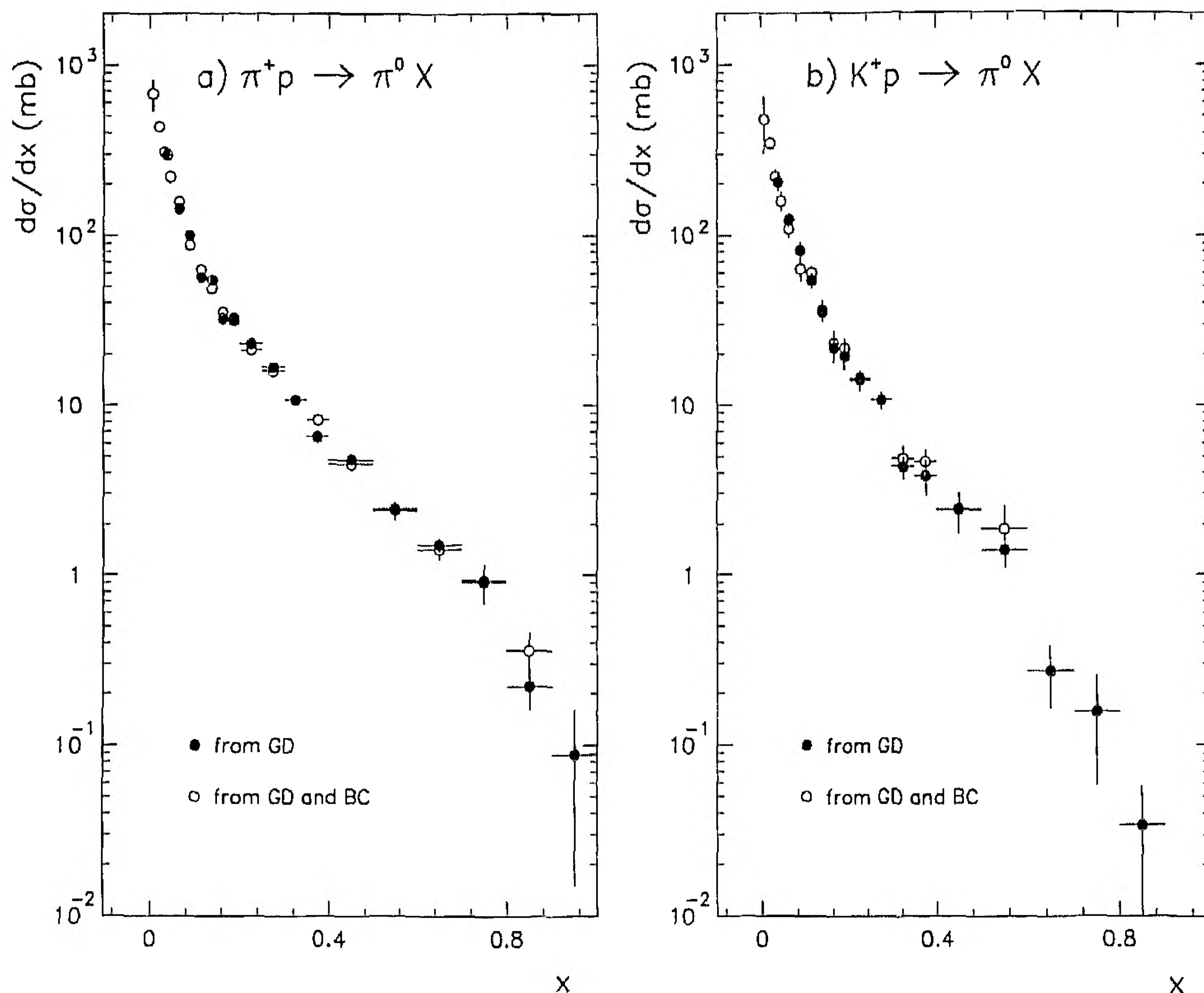
Fig. 3a, b. The d\sigma/dx distribution obtained from IGD and FGD \gamma\gamma invariant mass spectra (full circles), compared with the spectrum based on combined RCBC and GD data (open circles) a for \pi^+p interactions at 250 GeV/c, b for K^+p interactions at 250 GeV/c
