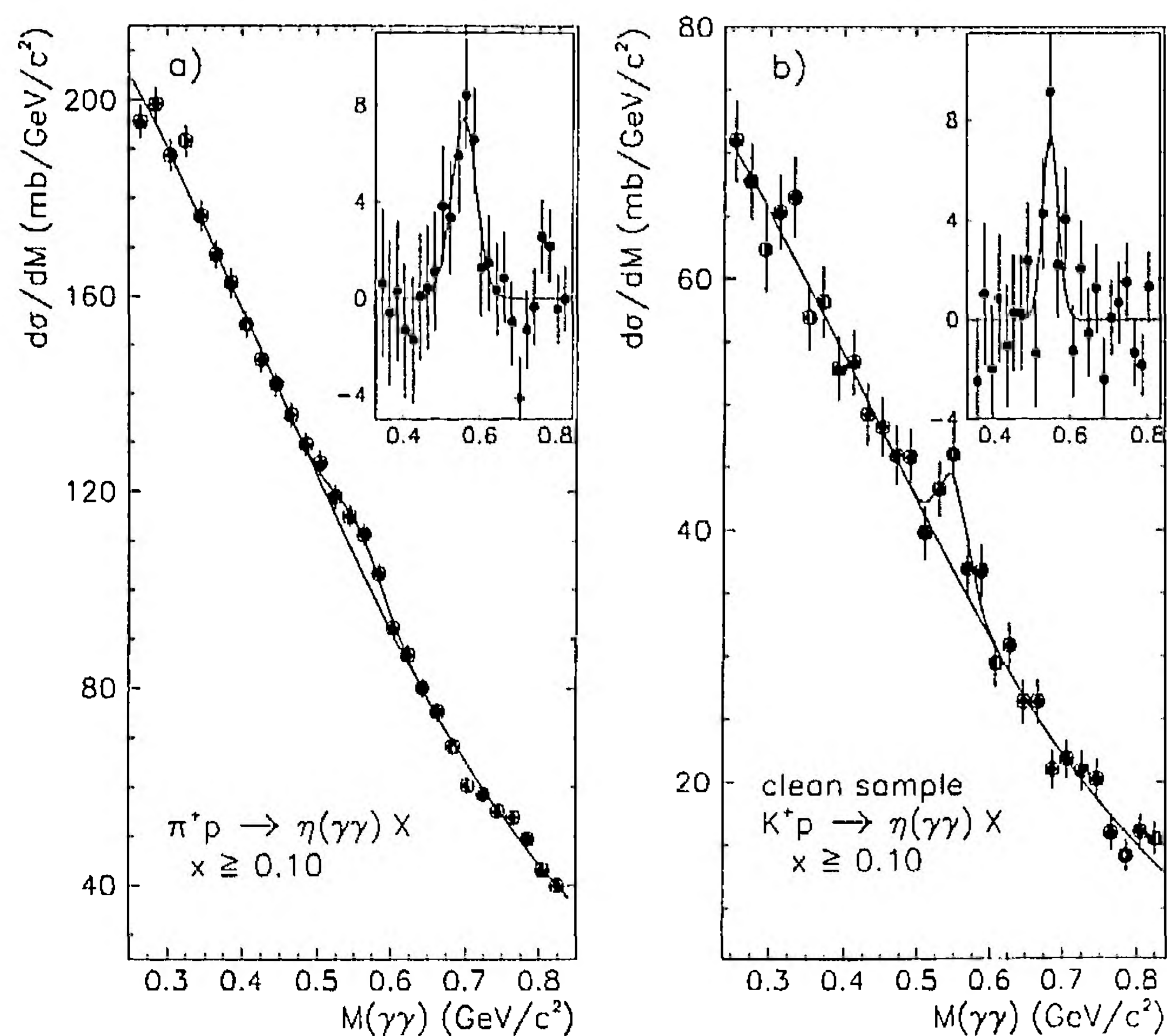
Fig. 7. a Weighted \gamma\gamma invariant mass distribution in the region x(\gamma\gamma) \geq 0.1 for \pi^+ p interactions at 250 GeV/c. The curves are the result of the fit described in the text. The insert shows the signal after subtraction of the background; b the same as in a, but for K^+ p interactions at 250 GeV/c and after removal of photons also contributing to the \pi^0 -signal
