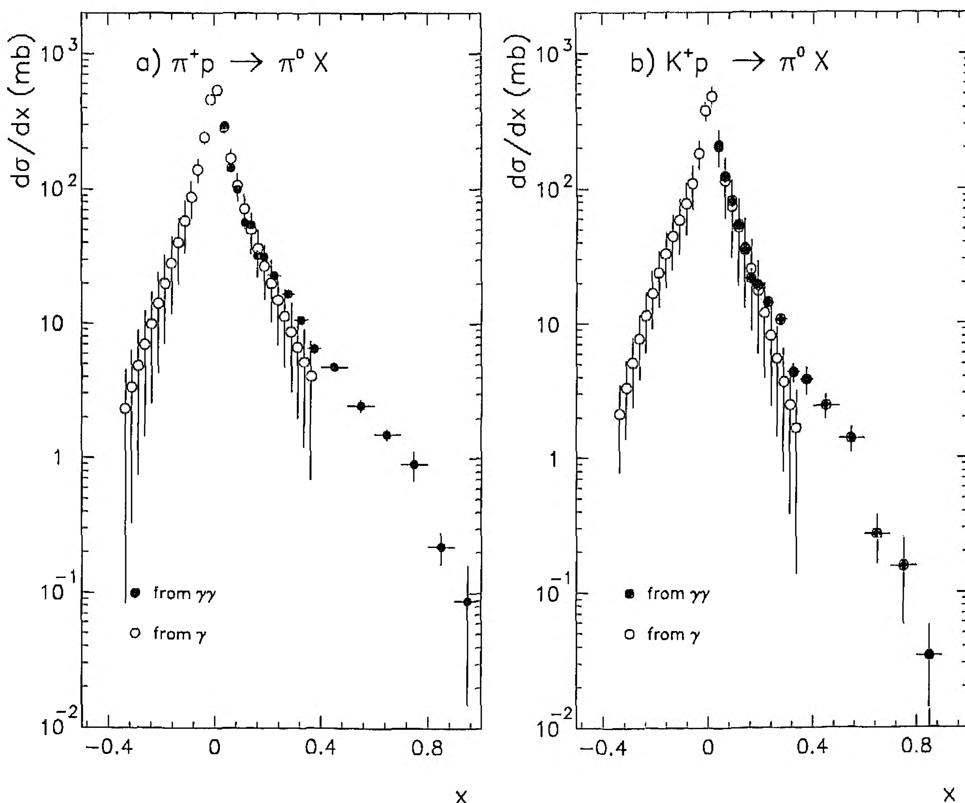
Fig. 2a, b. The d\sigma/dx distribution obtained from IGD and FGD \gamma\gamma invariant mass spectra in separate x -intervals (full circles), compared to the result of a fit to the RCBC \gamma spectrum (open circles) a) for \pi^+p interactions at 250 GeV/c, b) for K^+p interactions at 250 GeV/c
