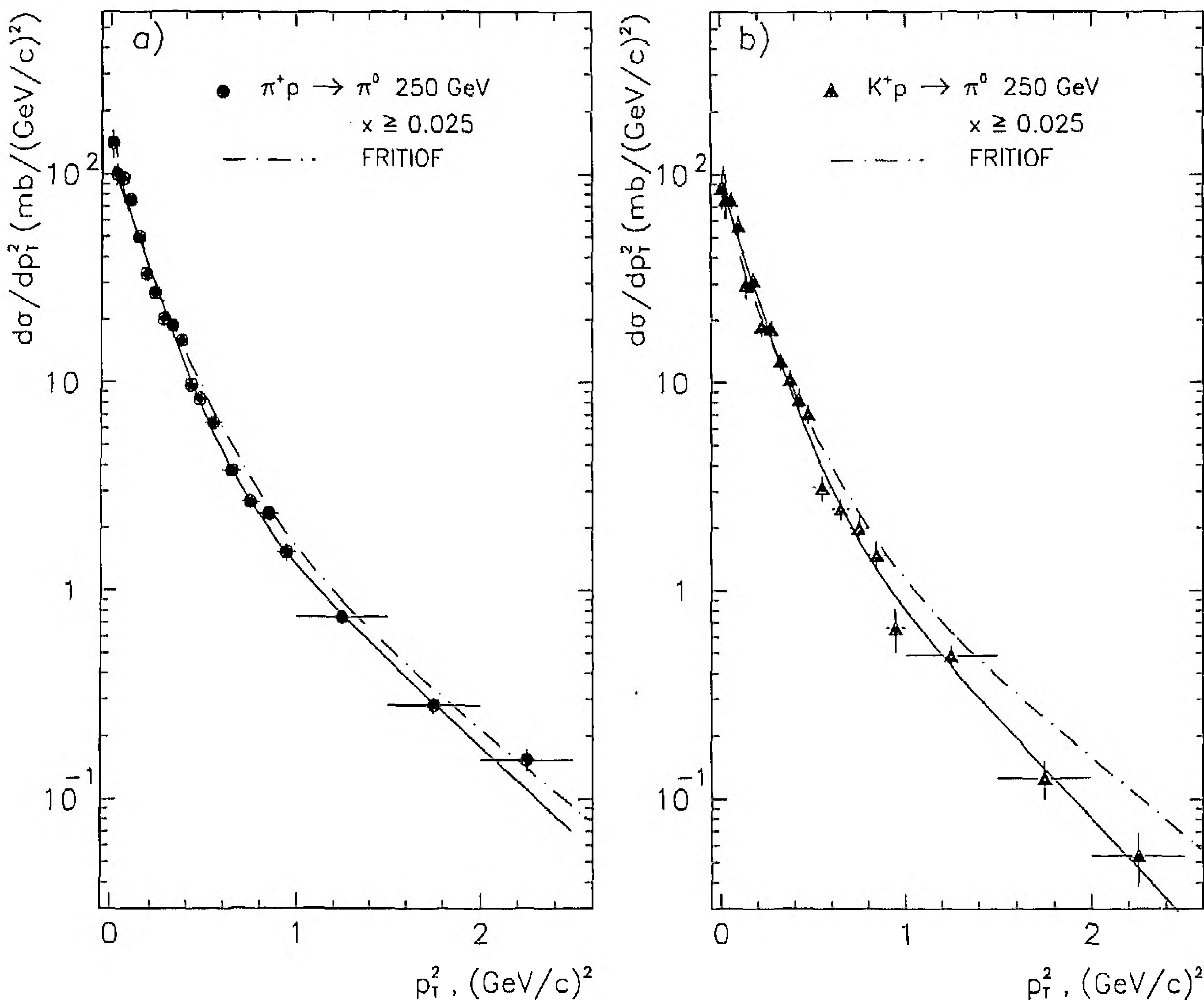
Fig. 6a, b. The d\sigma/dp_T^2 distribution for reaction (1) a and (2) b with x \geq 0.025 at 250 GeV/c. Solid curves are fits to the sum of two exponentials described in the text. Dashed-dotted curves are predictions of the FRITIOF model
