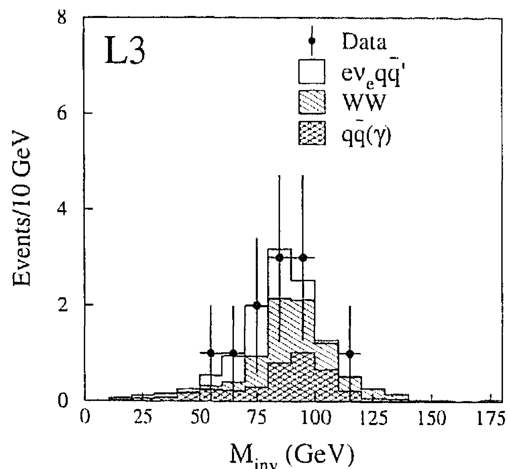
Fig. 7. The jet-jet invariant mass spectrum, M_{inv} of the selected hadronic candidates for the combined data sample. The hatched histogram represents the background, the open histogram shows the fitted signal from e^+\nu_e q\bar{q}' final states.
