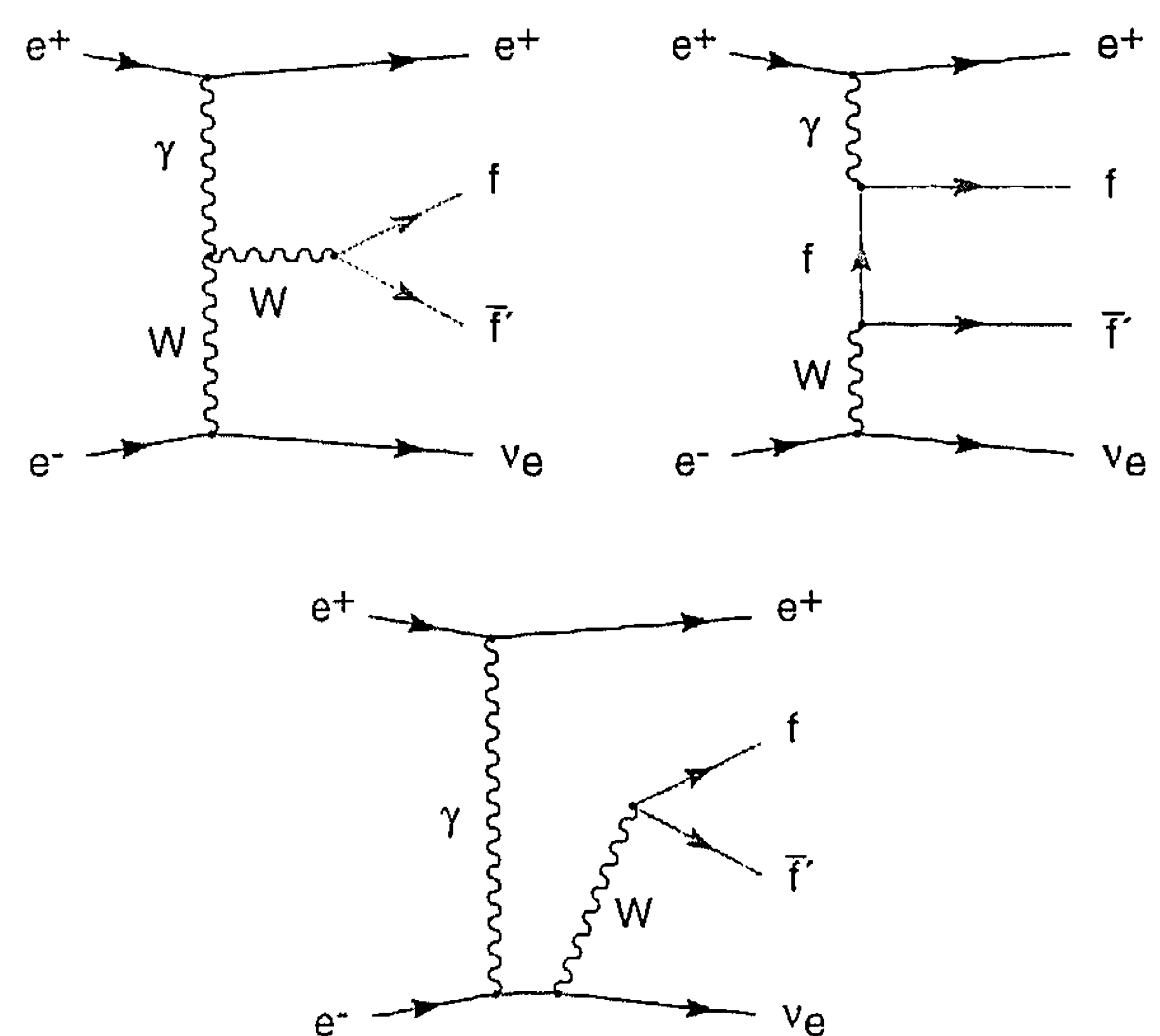
Fig. 1. The dominant Feynman diagrams for the process (1).
