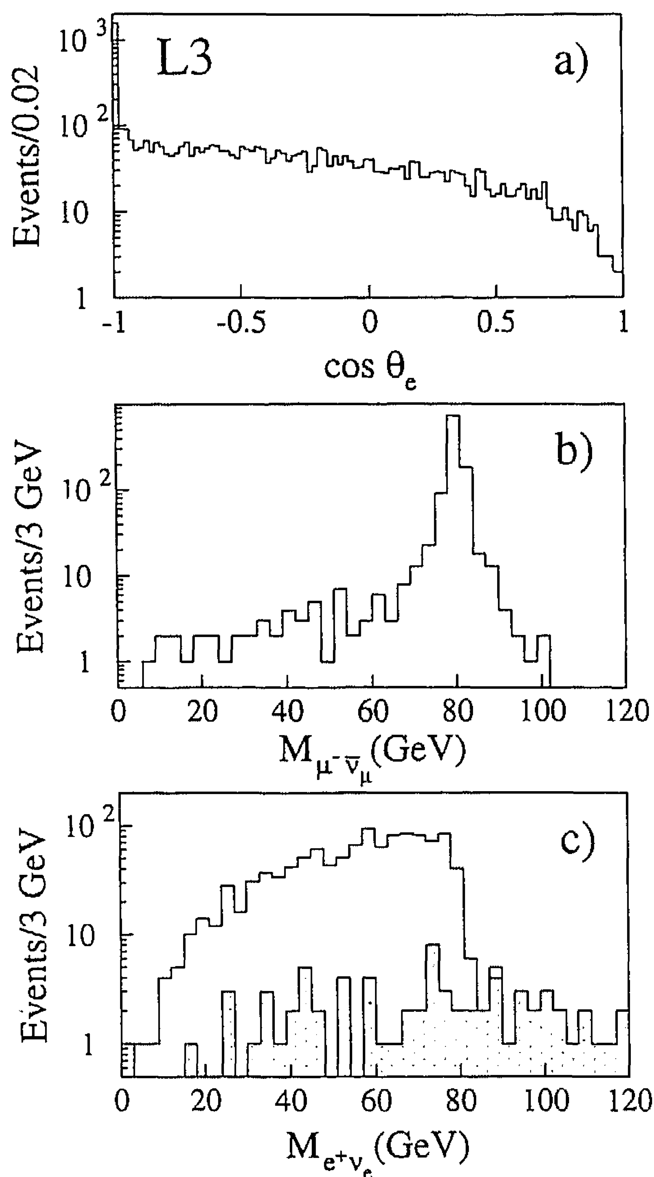
Fig. 2. (a) The positron polar angle spectrum for all e^+\nu_e\mu^-\bar{\nu}_\mu final states generated by GRC4F at \sqrt{s} = 161 GeV. The invariant mass spectrum of the \mu^-\bar{\nu}_\mu (b) and e^+\nu_e (c) pairs for the events satisfying phase space conditions (2). The hatched histogram in (c) represents events which meet the requirement |M_{\mu\nu\mu} - M_W| > 10 GeV.
