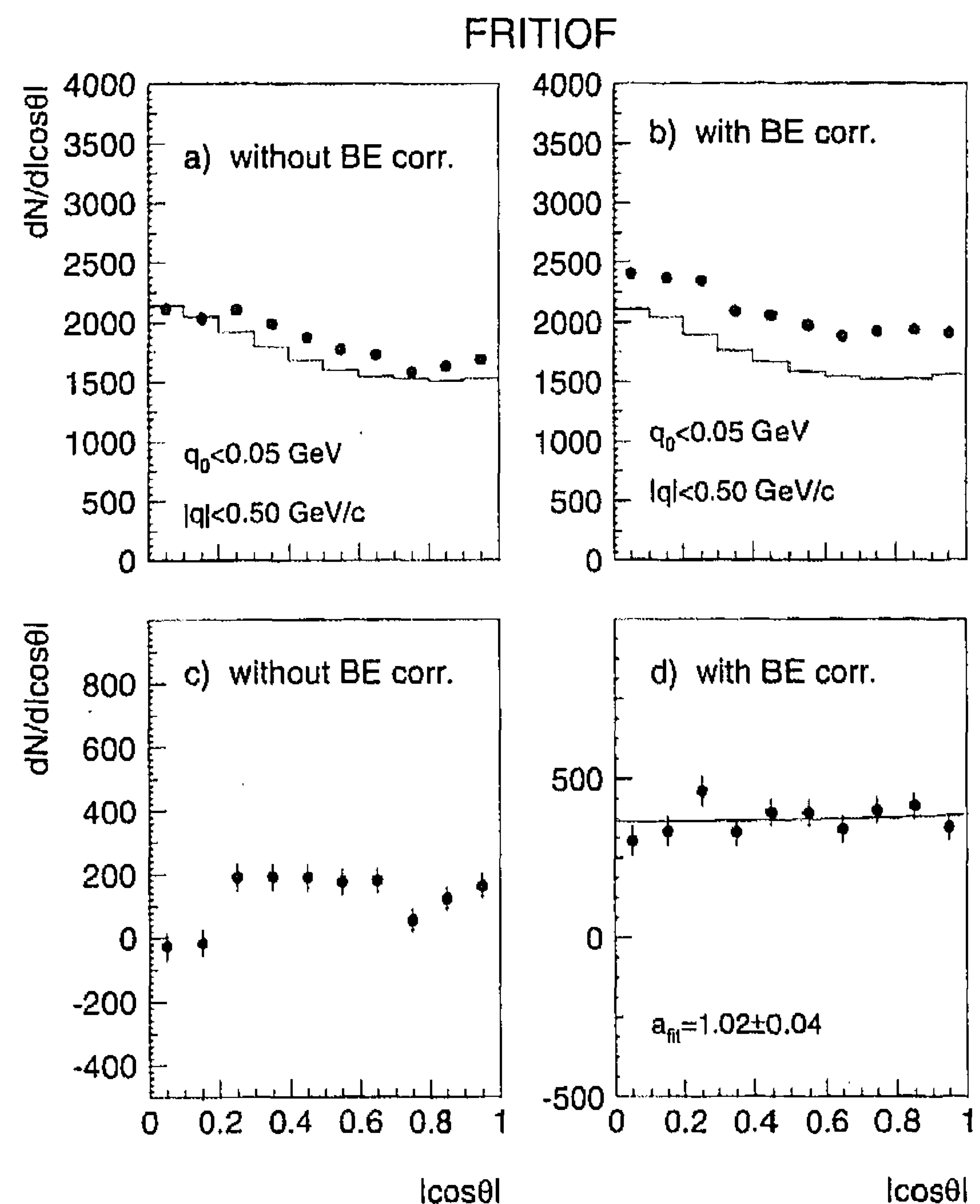
Fig. 4. The angular distribution of the vector \mathbf{q} at q_{cut} = 0.5 GeV/c and (q_0)_{cut} = 0.05 GeV for FRITIOF a) without and b) with Bose-Einstein correlations (points: generated distribution; histograms: generated reference distribution). c,d) The results of the subtraction of the distributions presented in a,b (curve: result of the fit by (3))
