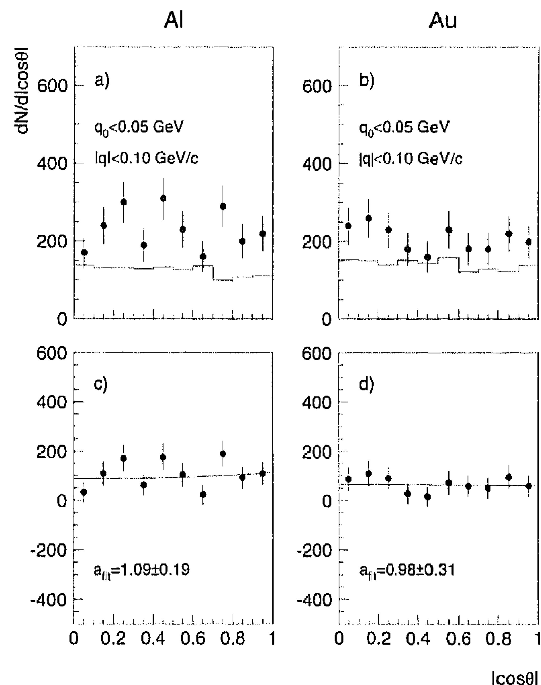
Fig. 8. (a,b) The angular distribution of the vector \mathbf{q} for pion pairs in meson-nucleus interactions with q_0 < 0.05 GeV, |\mathbf{q}| < 0.10 GeV/c. Points: experimentally observed distribution; histograms: reference distribution. (c,d) The result of the subtraction of the distributions presented in a,b (curves: the result of the fits by expression (3))
