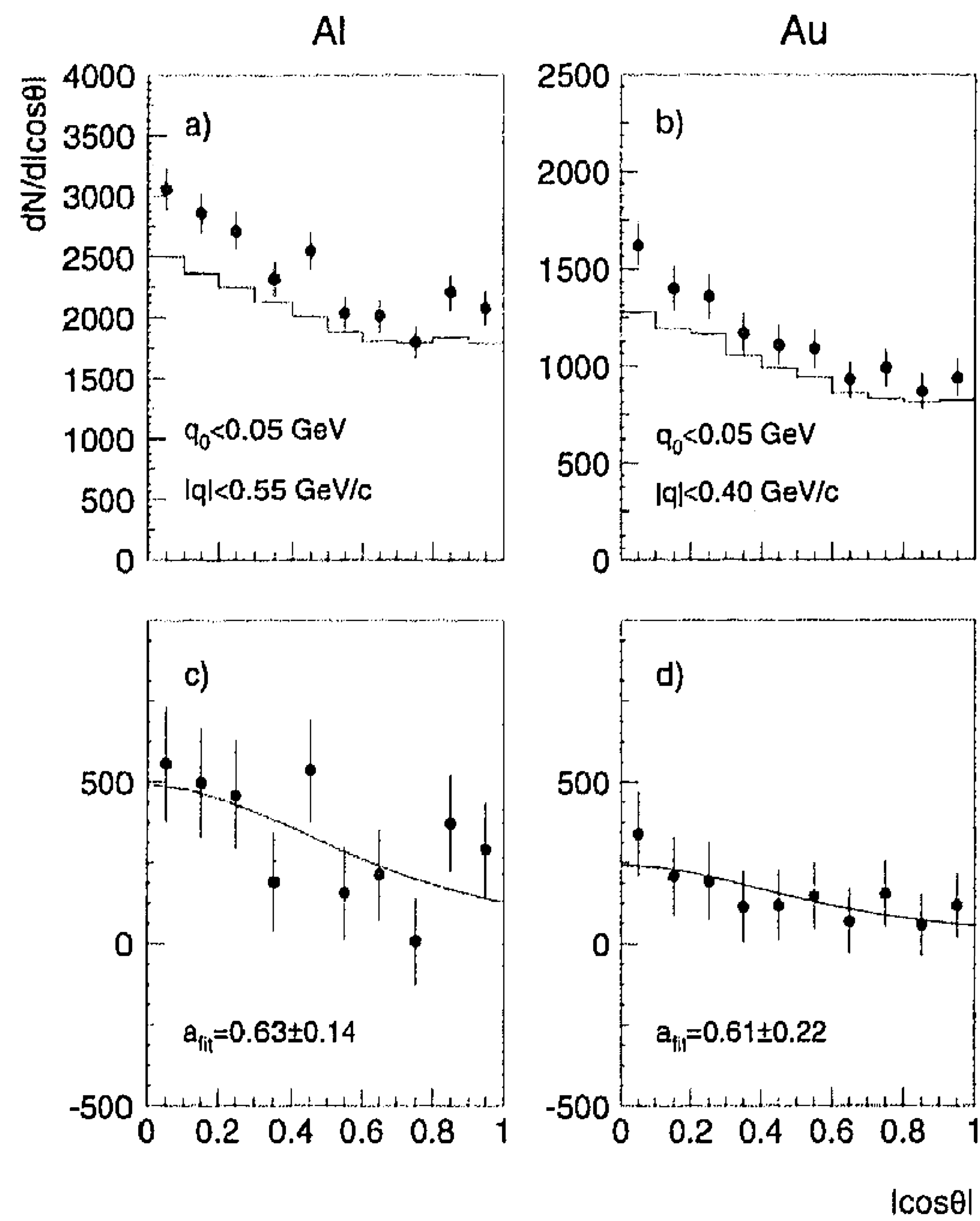
Fig. 9. The same as in Fig.8, but for q_0 < 0.05 GeV and |q| < 0.55 GeV/c (Al) and |q| < 0.40 GeV/c (Au)
