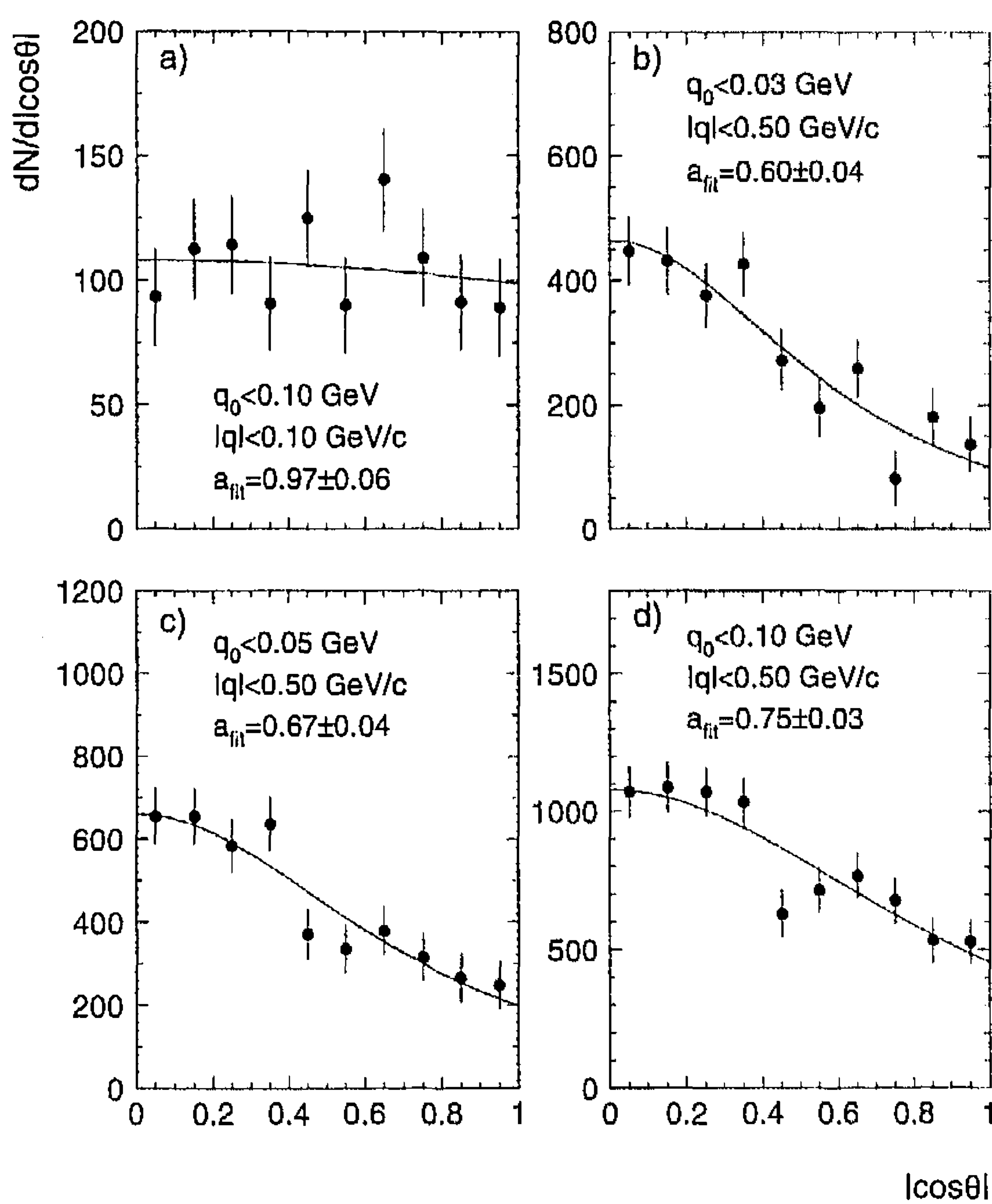
Fig. 3. The result of the subtraction of the distributions presented in Fig. 2 (curves: result of the fits by (3))
