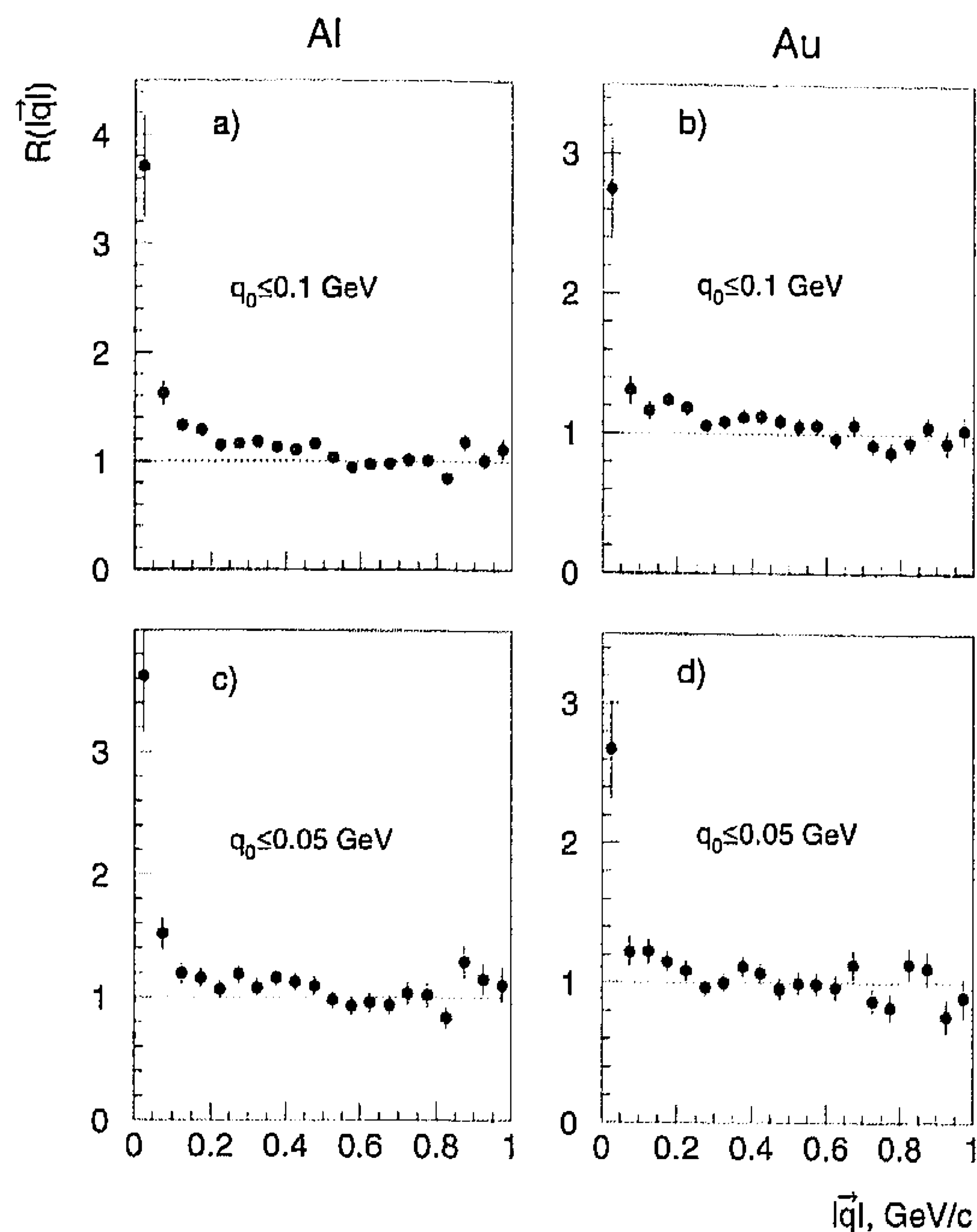
Fig. 7. The correlation function for pairs of negative pions with q_0 < (q_0)_{cut} in meson-nucleus interactions
