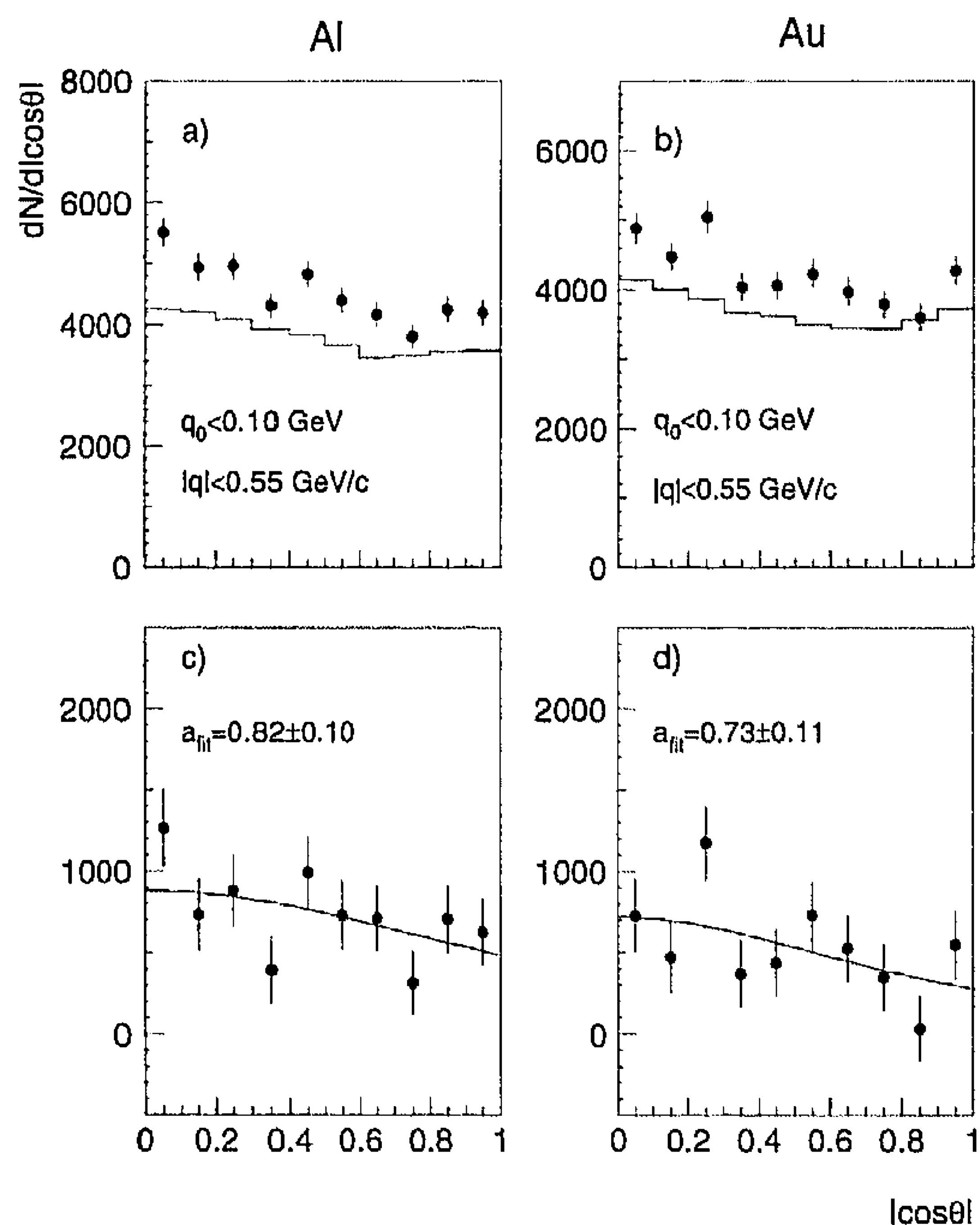
Fig. 10. The same as in Fig.8, but for q_0 < 0.10 GeV and |q| < 0.55 GeV/c
