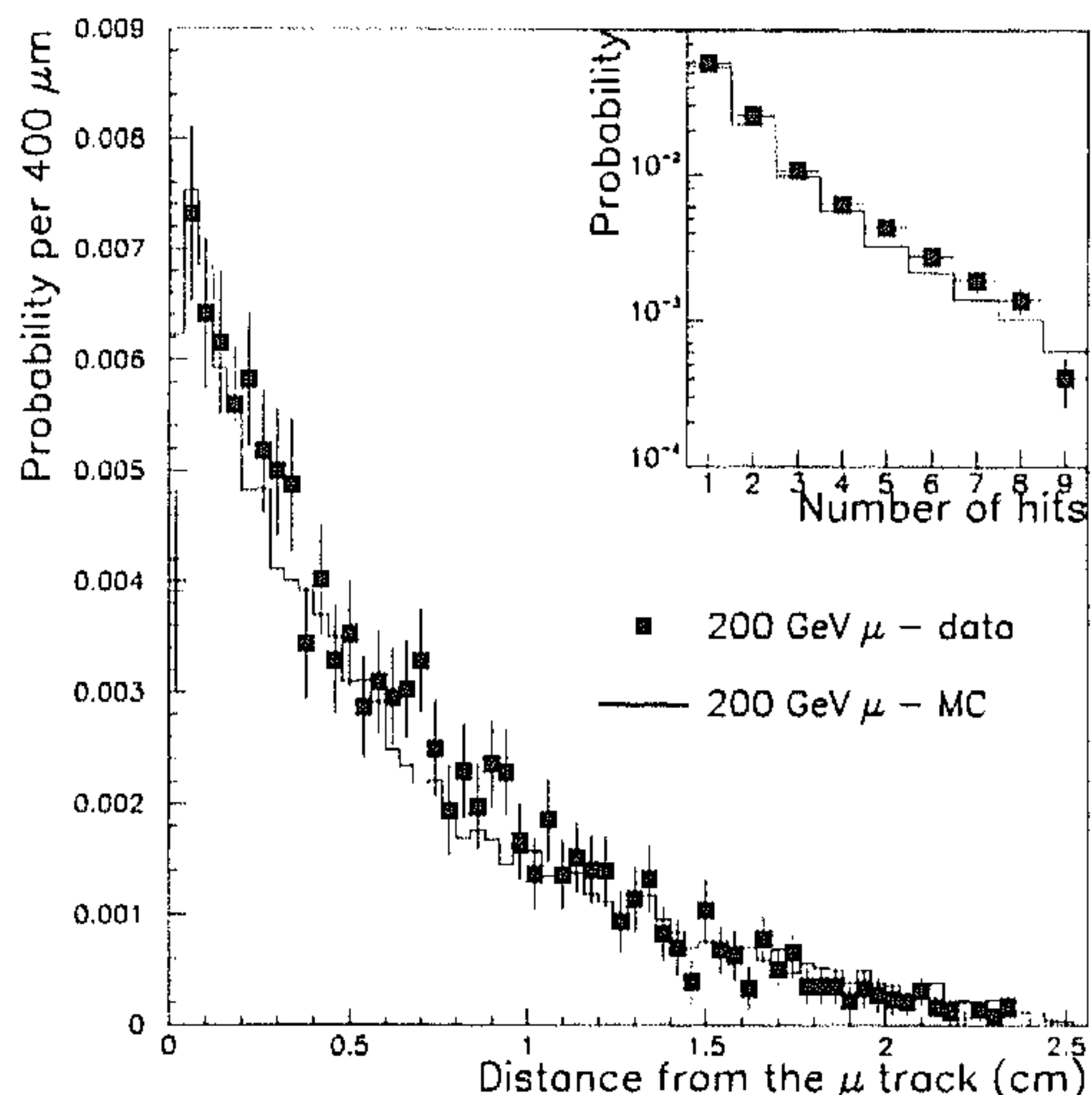
Fig. 3. Distribution of the distance of additional hits in the SiBT due to showering induced by a muon in the iron, at 4.7 cm from the absorber. The inset shows the probability distribution of the number of additional hits.
