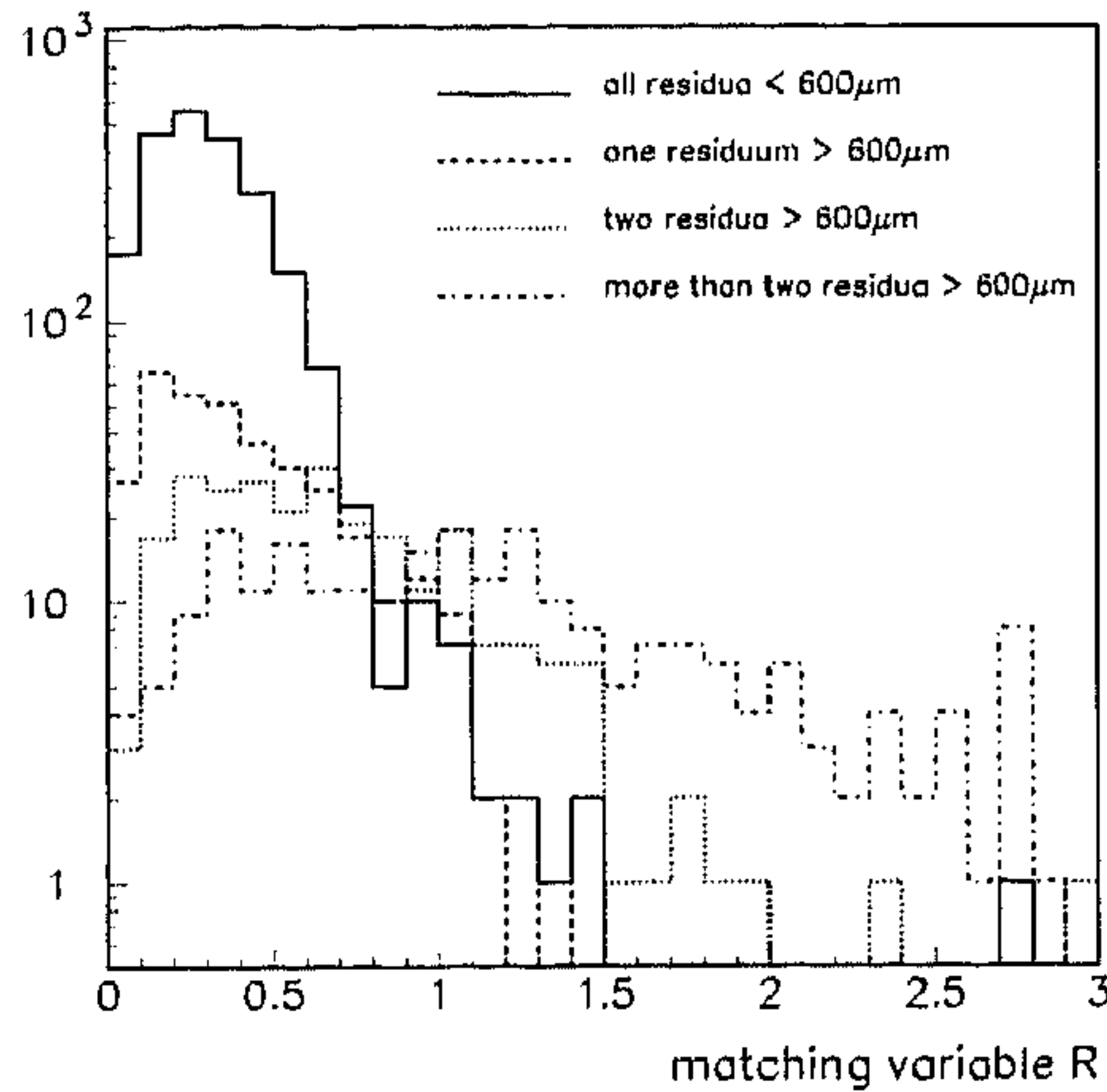
Fig. 20. Muons of 200 GeV measured in the WLDC and compared with an external track measurement. Distribution of the matching variable R measured for different even classes. For “good matching” we require R < 1 . Since here the reference track had to be extrapolated over a long path, a large R reflects mainly angular mismatches.
