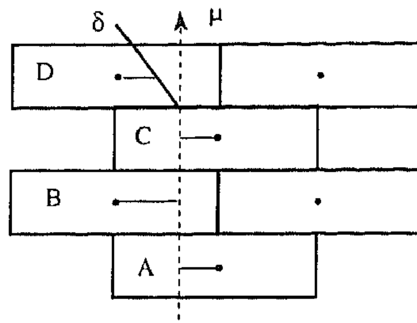
Fig. 14. The presence of a \delta -electron in one layer leads to a wrong mean timer measurement.
