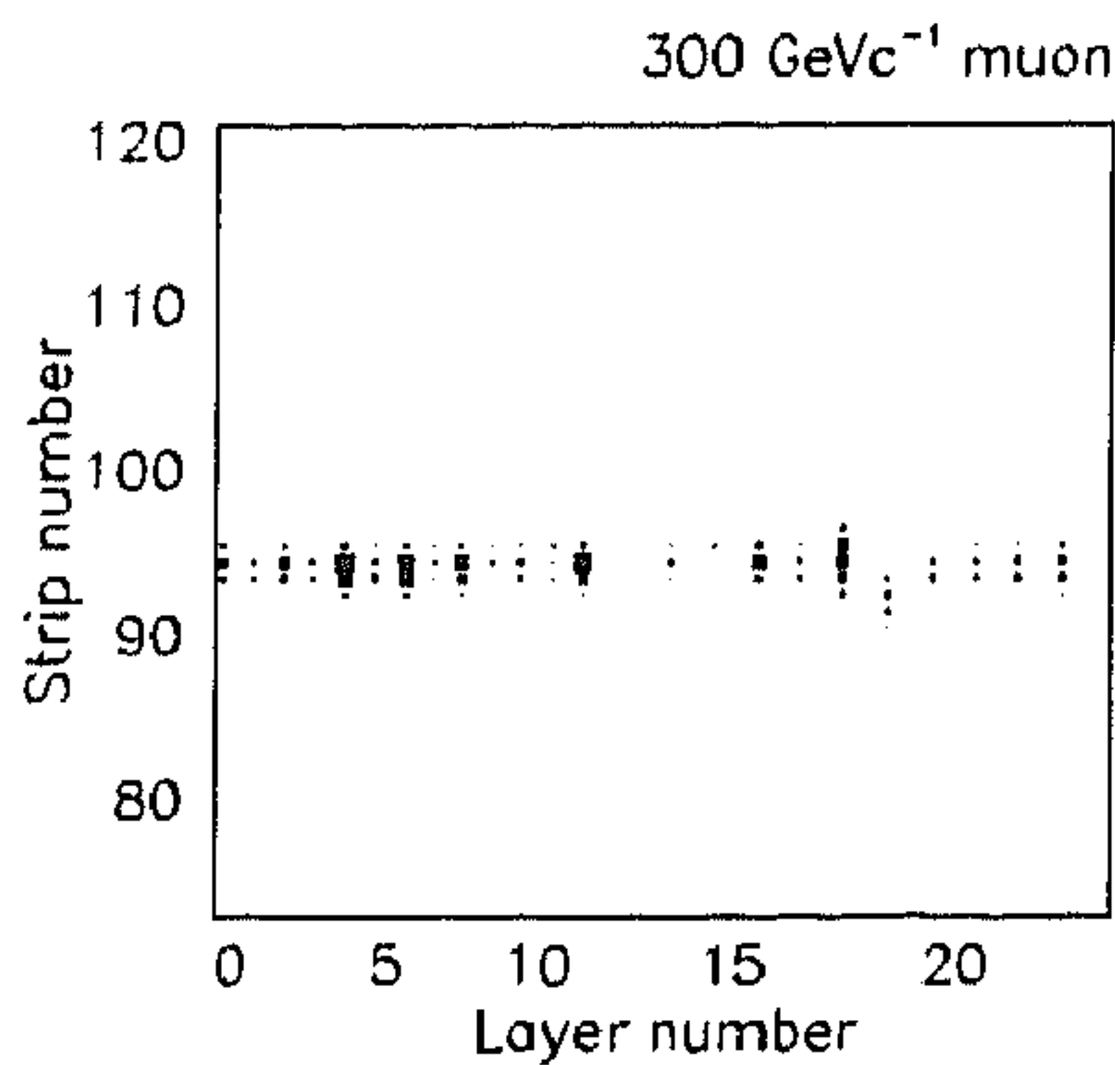
Fig. 4. A typical muon track through TRACAL. The box size is proportional to the charge collected by the indicated strip.
