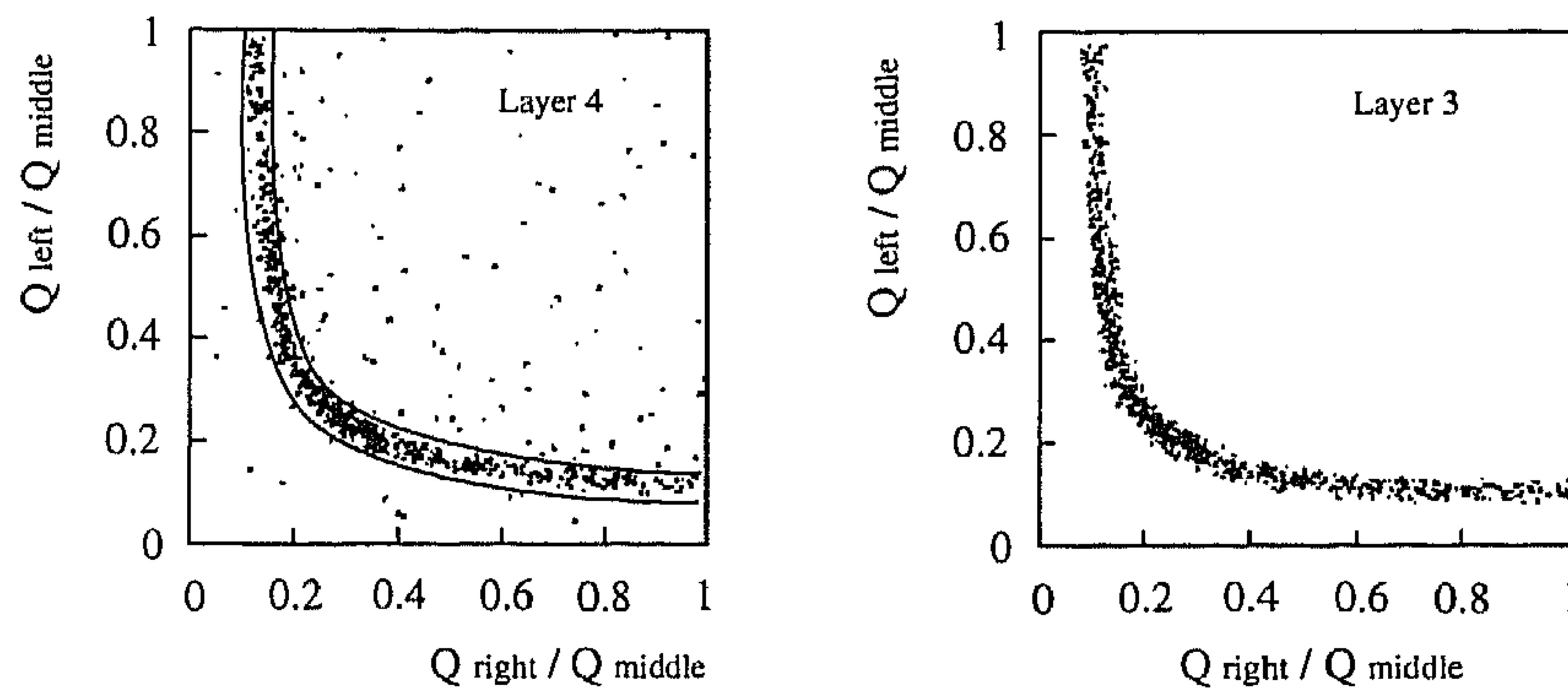
Fig. 7. Scatter plot of the ratio Q_{\text{left}}/Q_{\text{middle}} versus Q_{\text{right}}/Q_{\text{middle}} in the CSC, for events with a single track reconstructed in three layers (labelled 1–3). As shown for layer 3 (right), the charges in these layers all lie within a narrow band. This band is also indicated in the distribution for the fourth layer (solid lines, left). Events above the expected range, in the fourth layer, are identified as a cosmic ray accompanied by \delta -electron(s). The position sensing cathode strips have a readout pitch of 5 mm.
