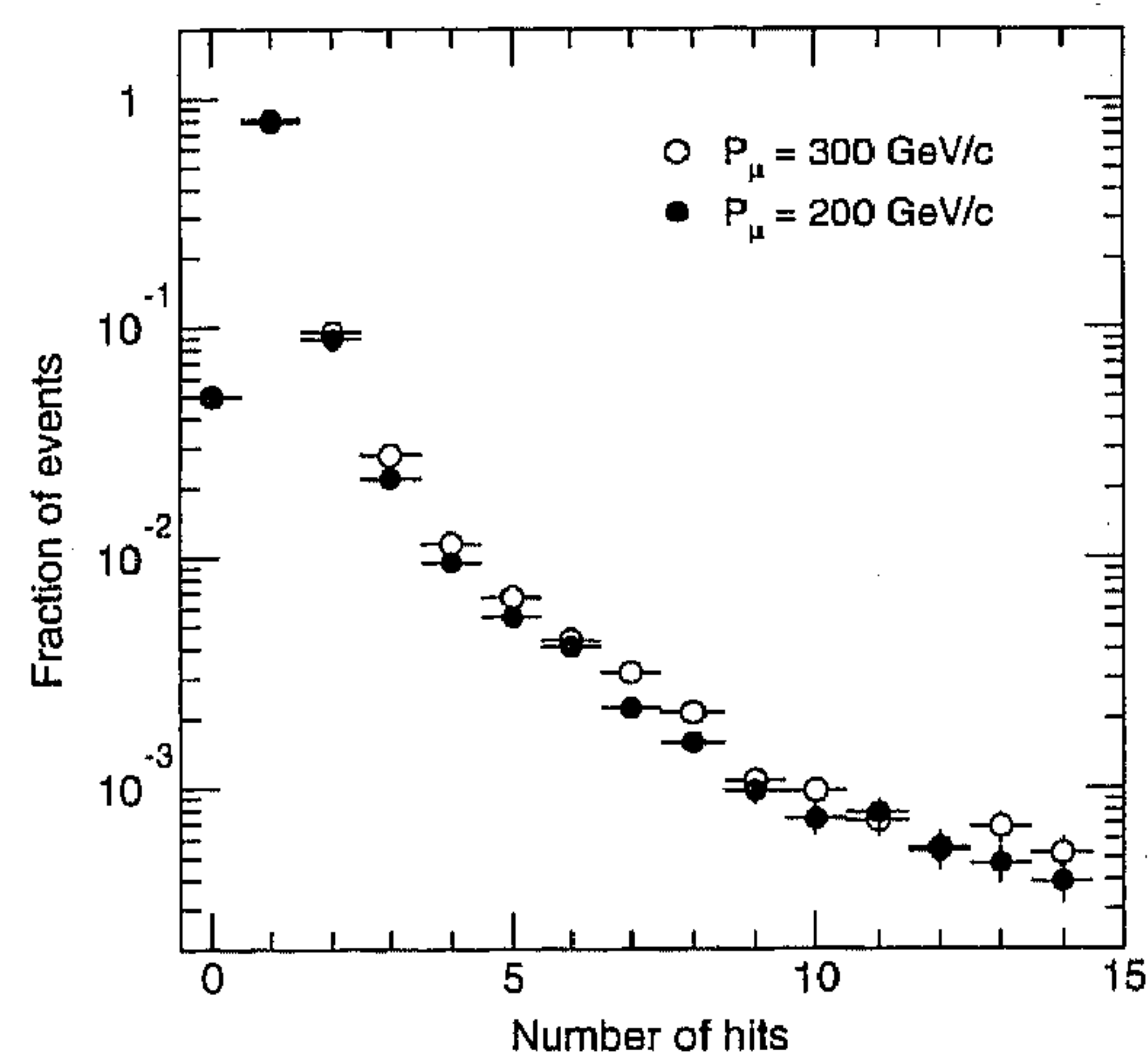
Fig. 8. Distribution of number of hits per CSC layer for 200 GeV/c and 300 GeV/c incident muons.
