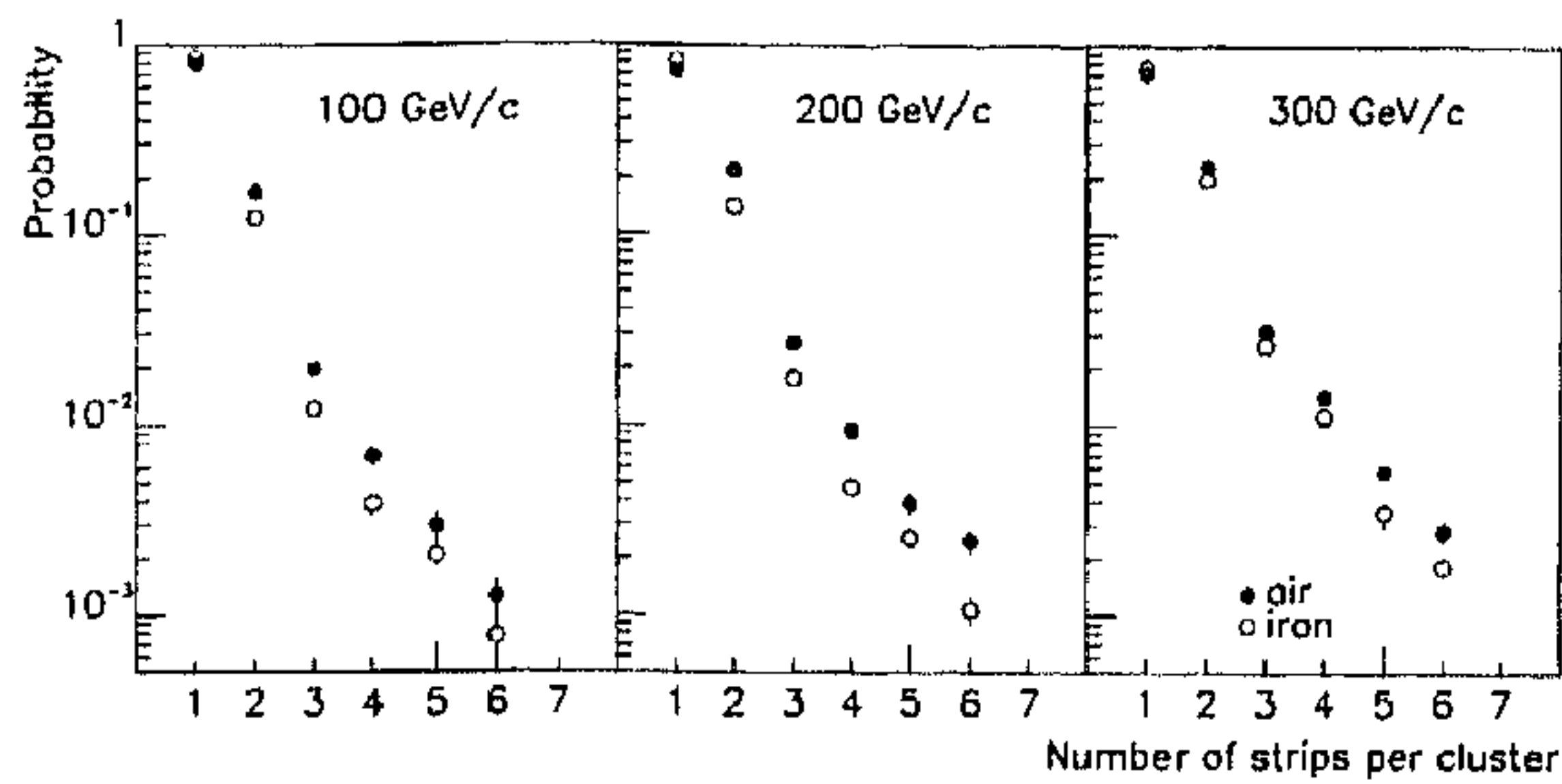
Fig. 17. Cluster size distribution for different muon energies. Open dots: RPC placed immediately behind the iron absorber; full dots: RPC placed 70 cm downstream from the absorber. The strip width is 3 cm.
