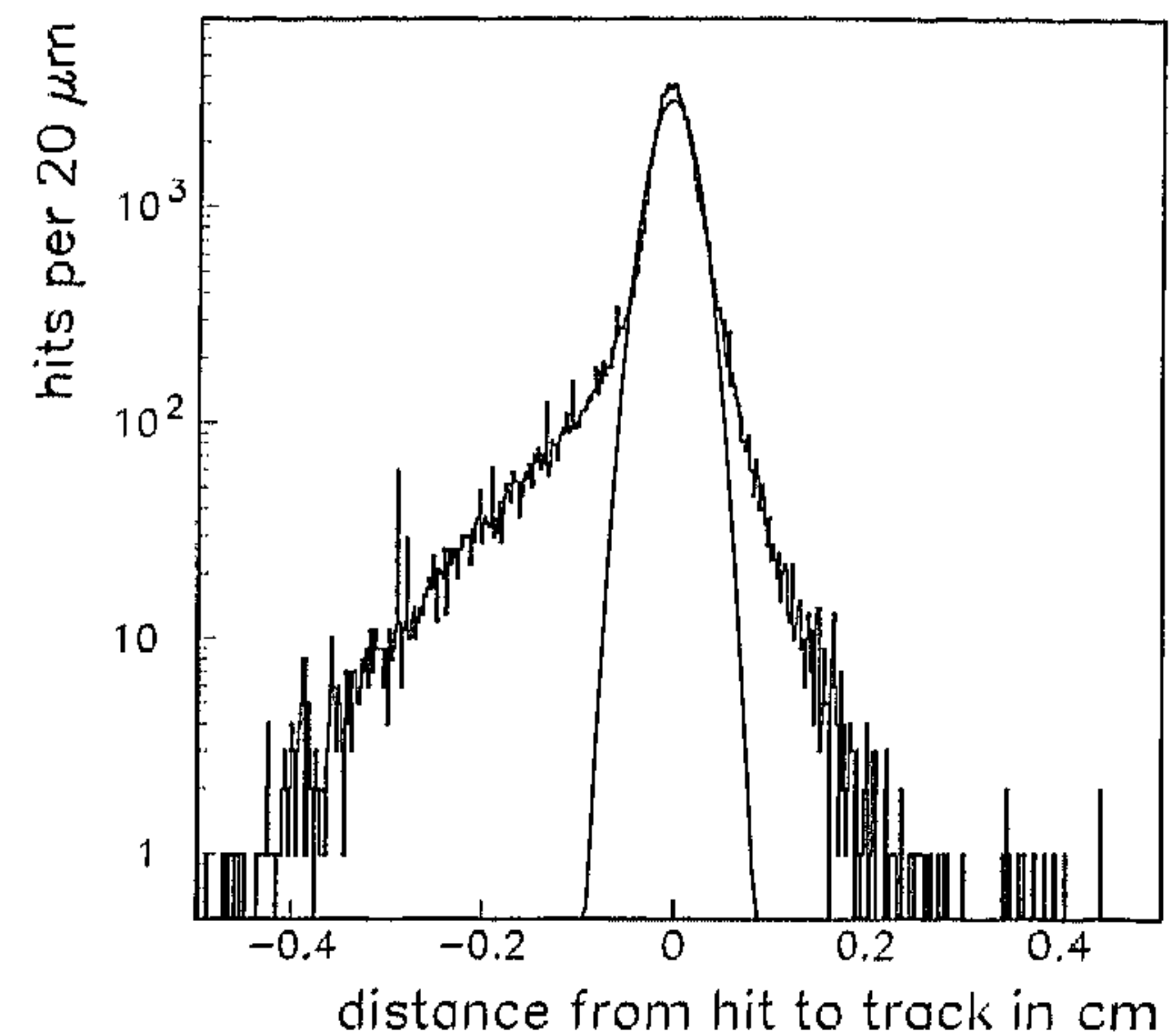
Fig. 10. WLDC data (200 GeV muons): Signed residua of a reconstructed muon track, with logarithmic scale to show the asymmetry. The anode is on the left side. A fitted Gaussian is also shown.
