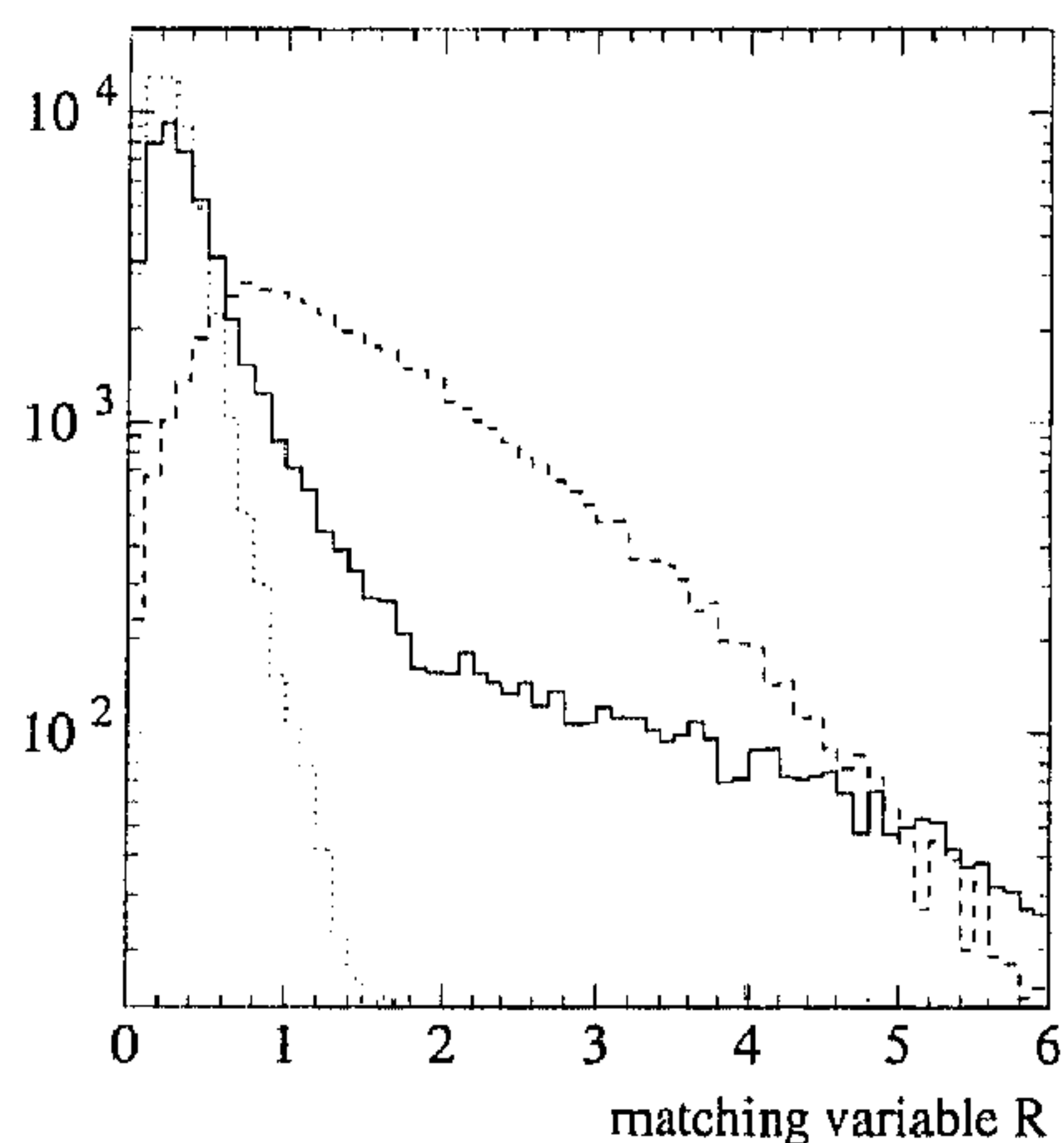
Fig. 22. Distribution of the matching variable R for those simulated events having at least one em secondary, using all hits (dashed line) and after removal of hits outside 350 \mu\text{m} (solid line). The fraction of tracks with R above 1 is reduced from 63.9% to 15.2%. As a reference, the distribution for undisturbed muons (no em secondaries; dotted line) features 0.6% of the events with R above 1. The three curves are normalized to the same area
