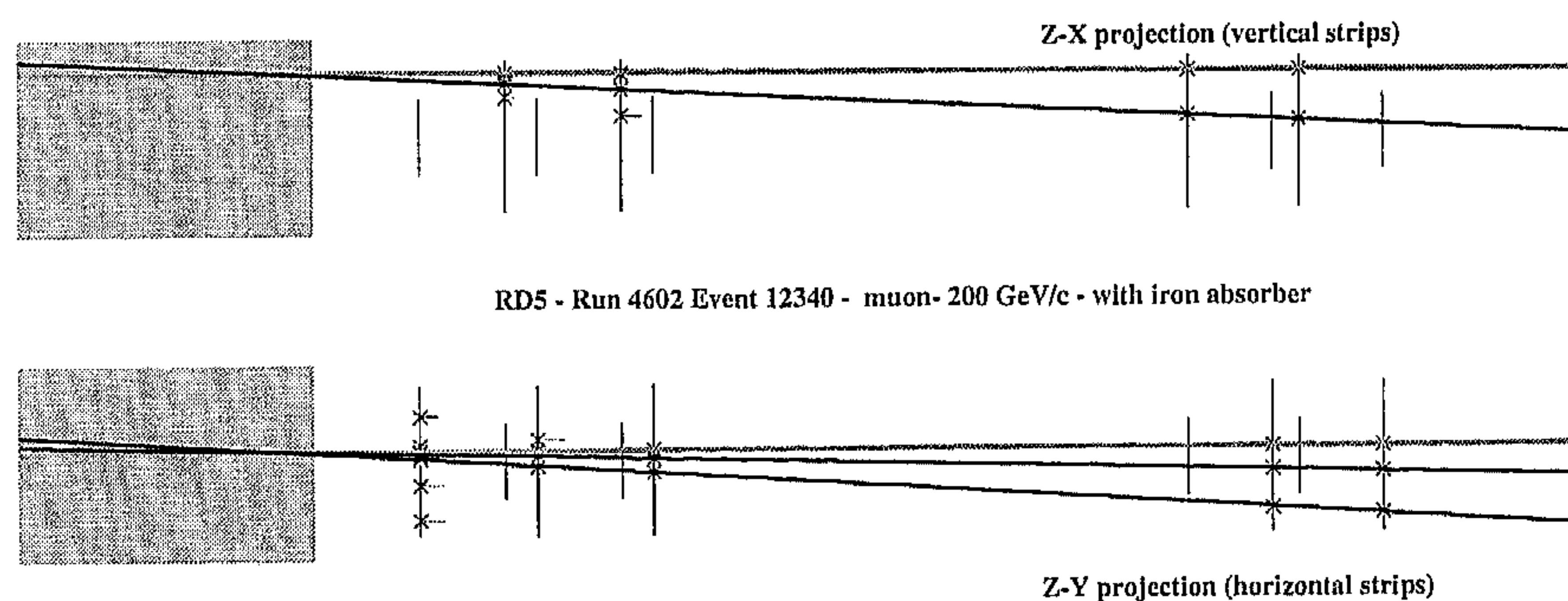
Fig. 1. Display of one event in the SiBT, in which a 200 GeV/c muon (dotted track) has generated two electrons in the iron block, of which one is reconstructed in both projections.
