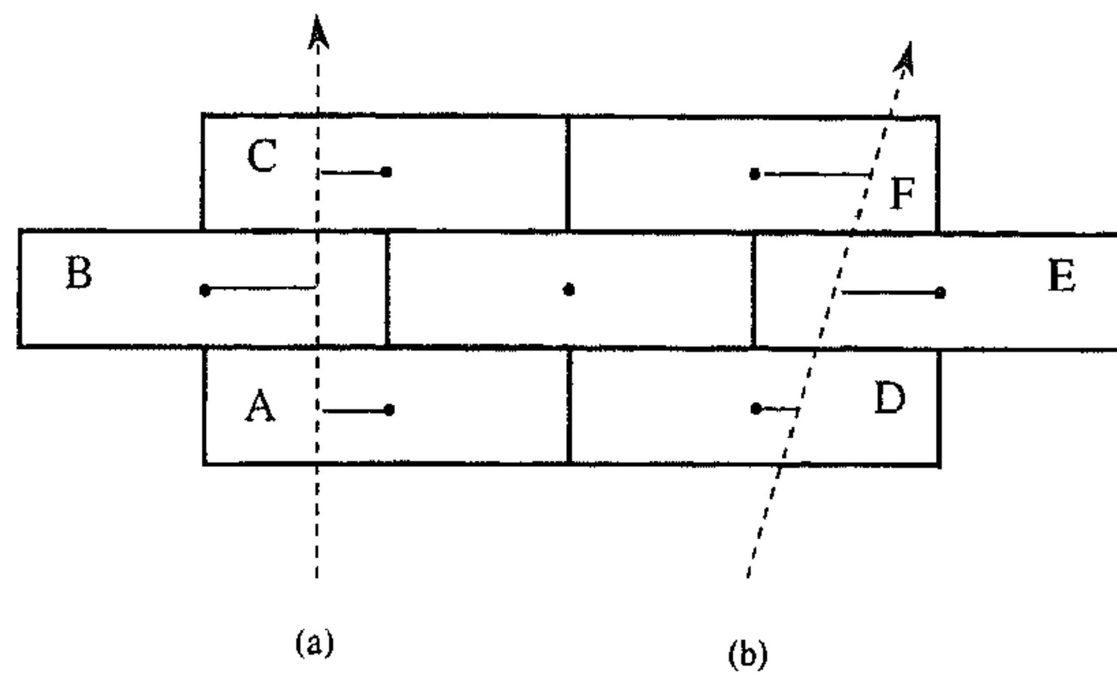
Fig. 12. Principle of mean-timer operation.
