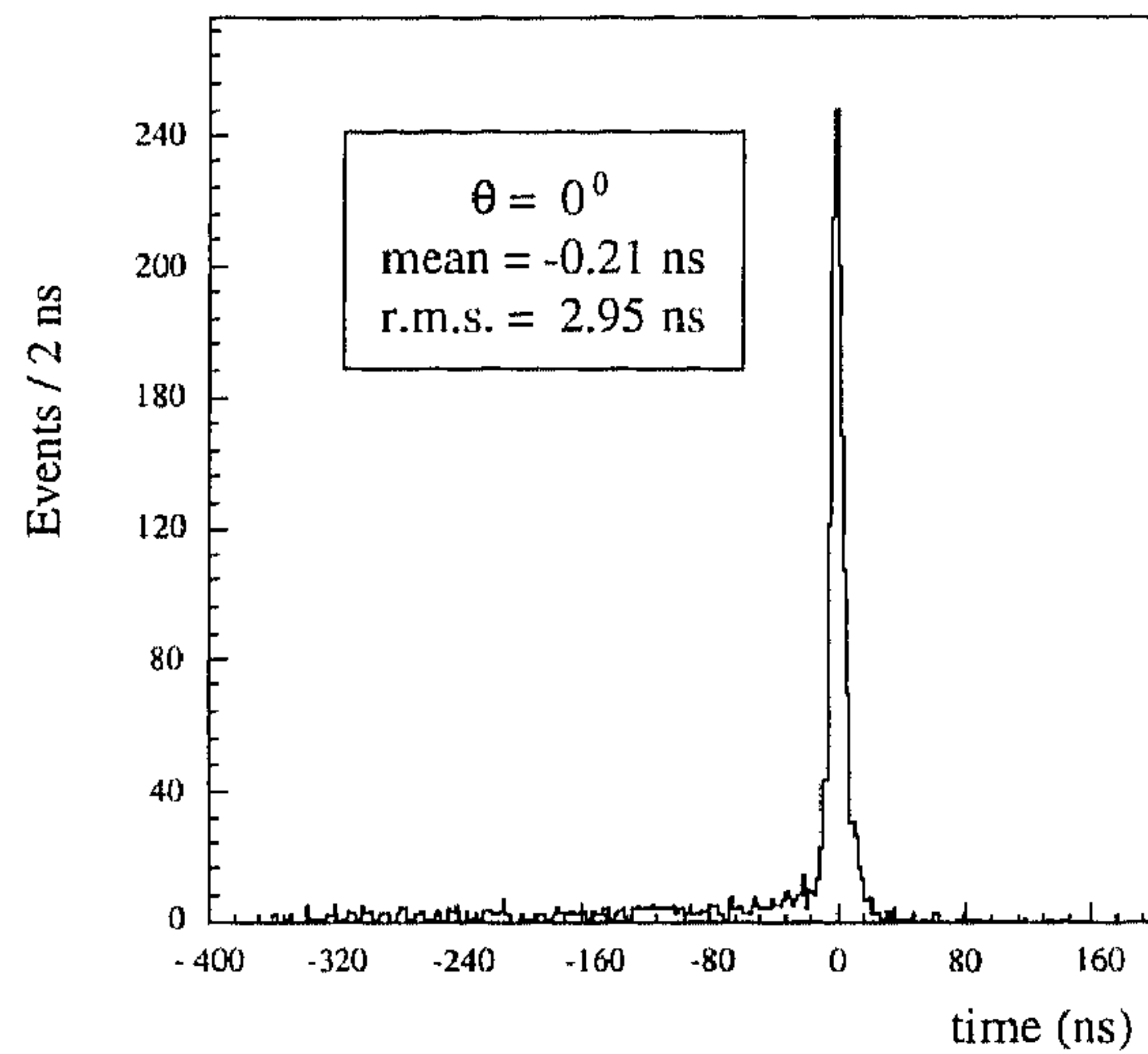
Fig. 13. Time distribution of the mean-timer sum for a DTBX exposed to 200 \text{ GeV}/c muons under normal incidence on the chamber.
