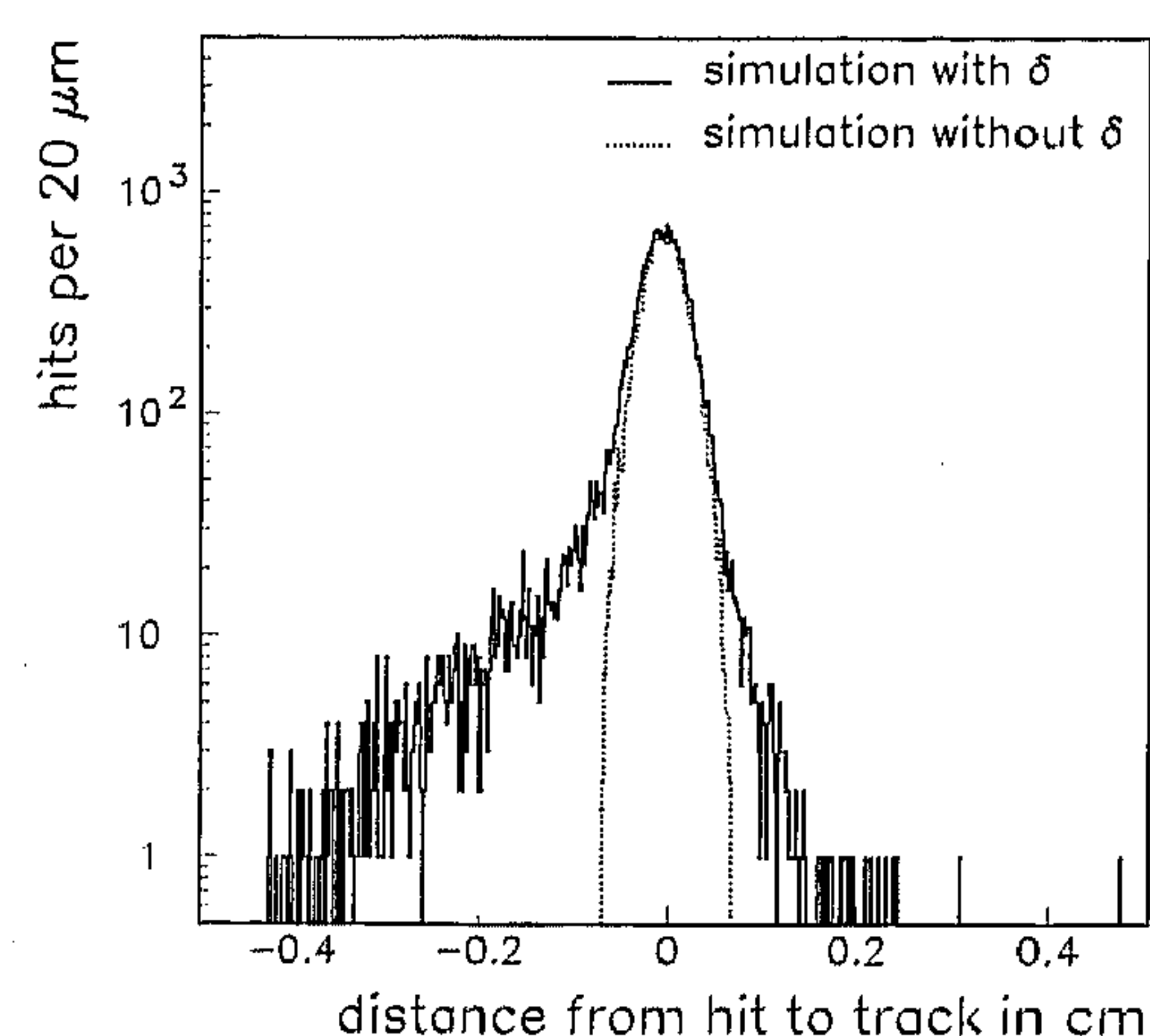
Fig. 11. WLDC simulation (200 GeV muons): Signed residua of reconstructed tracks, with logarithmic scale to show the asymmetry. The solid line is the simulation including \delta -electrons, the dotted line is the simulation without generation of secondaries.
