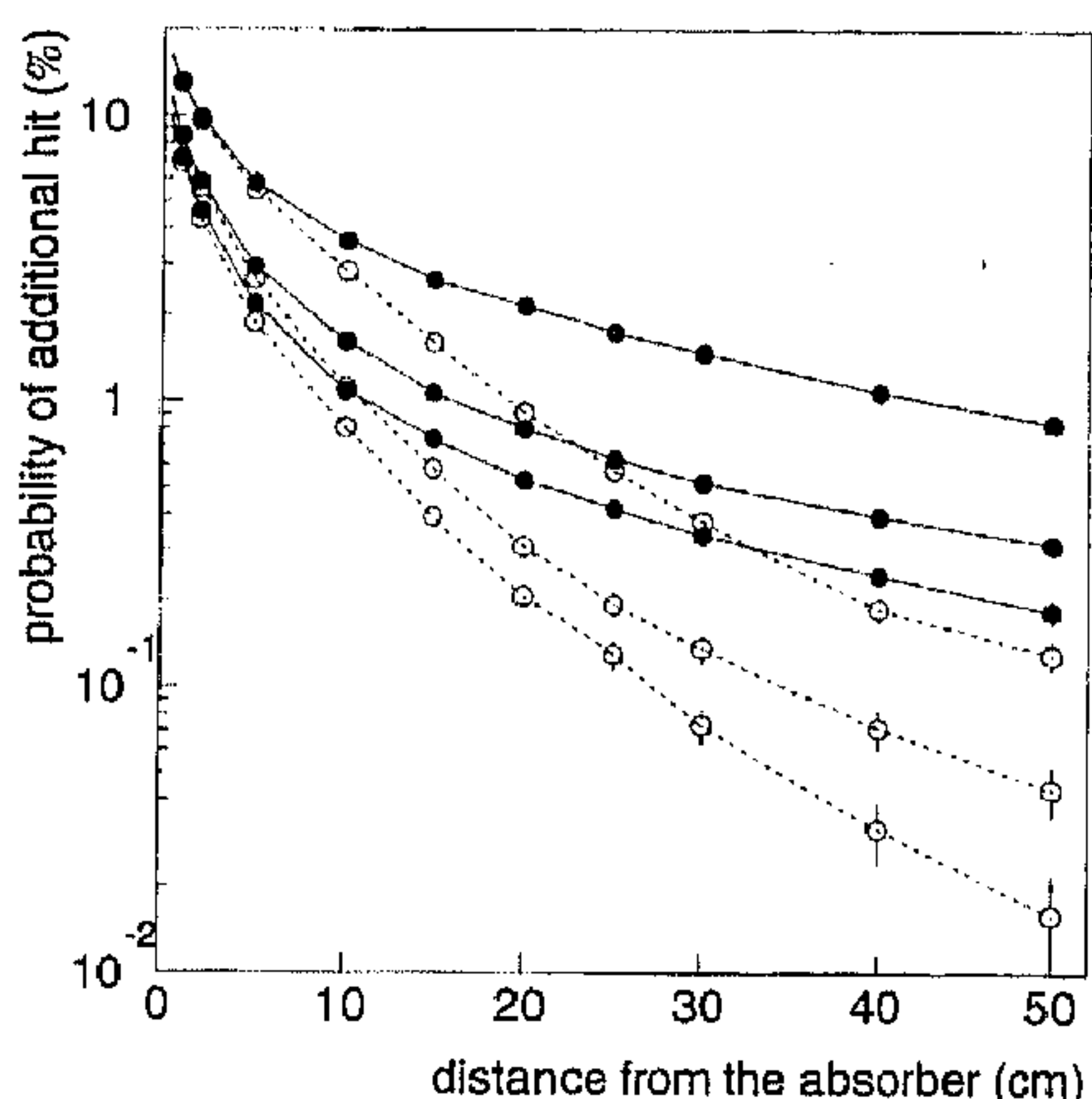
Fig. 19. Probability of having a spoiled muon hit versus the distance from the absorber for a two hit resolution of 5 mm. The muon momentum is 300, 100 and 50 GeV/c (top to bottom). Solid lines are for magnetized iron; dashed lines for 0.6 T downstream the absorber.
