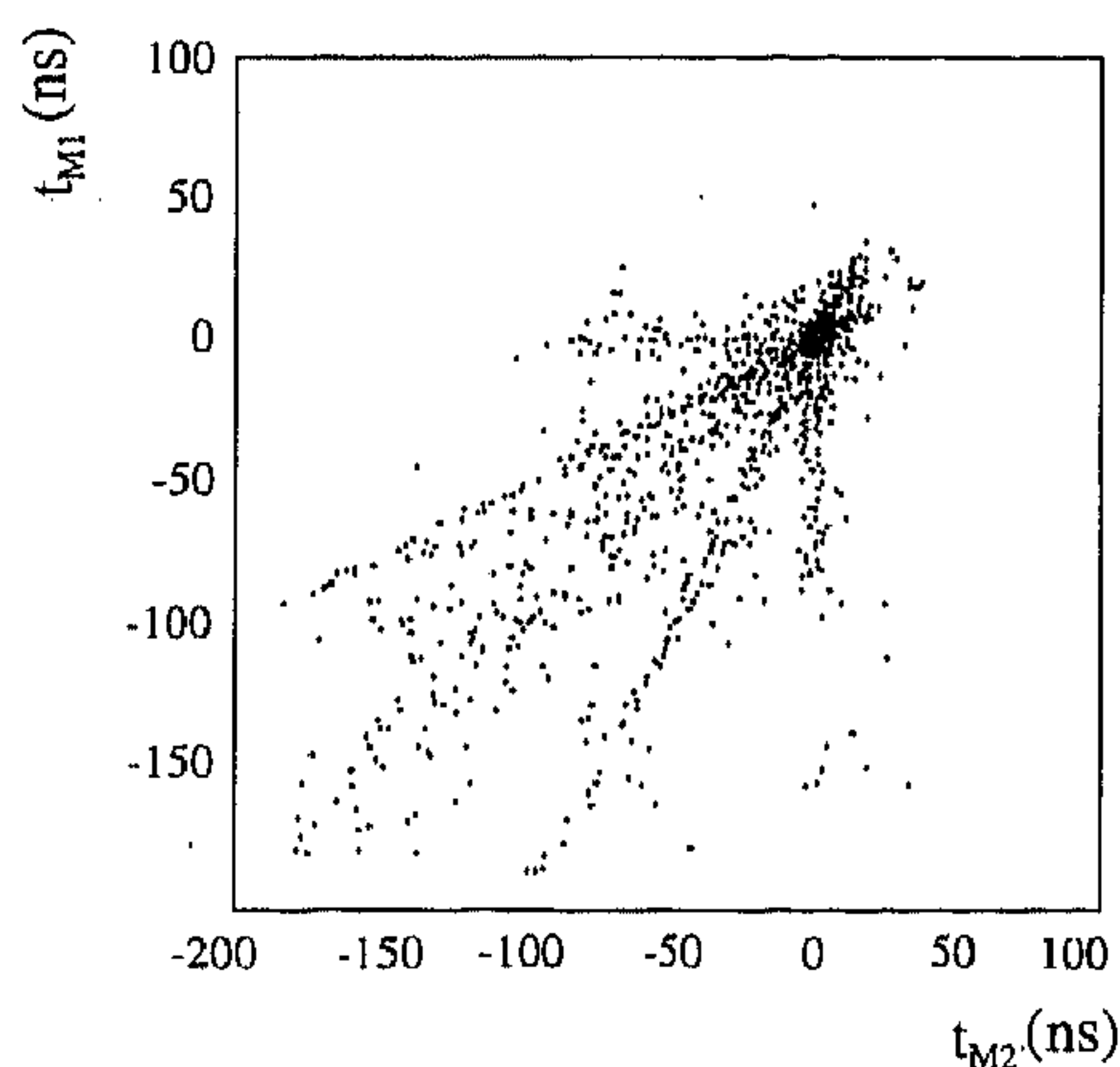
Fig. 15. Correlation between the two mean timer measurements obtained from the 4-layer DTBX. Points at the origin represent undisturbed muon tracks. The four lines are an indication for tracks disturbed in only one of the four layers.
