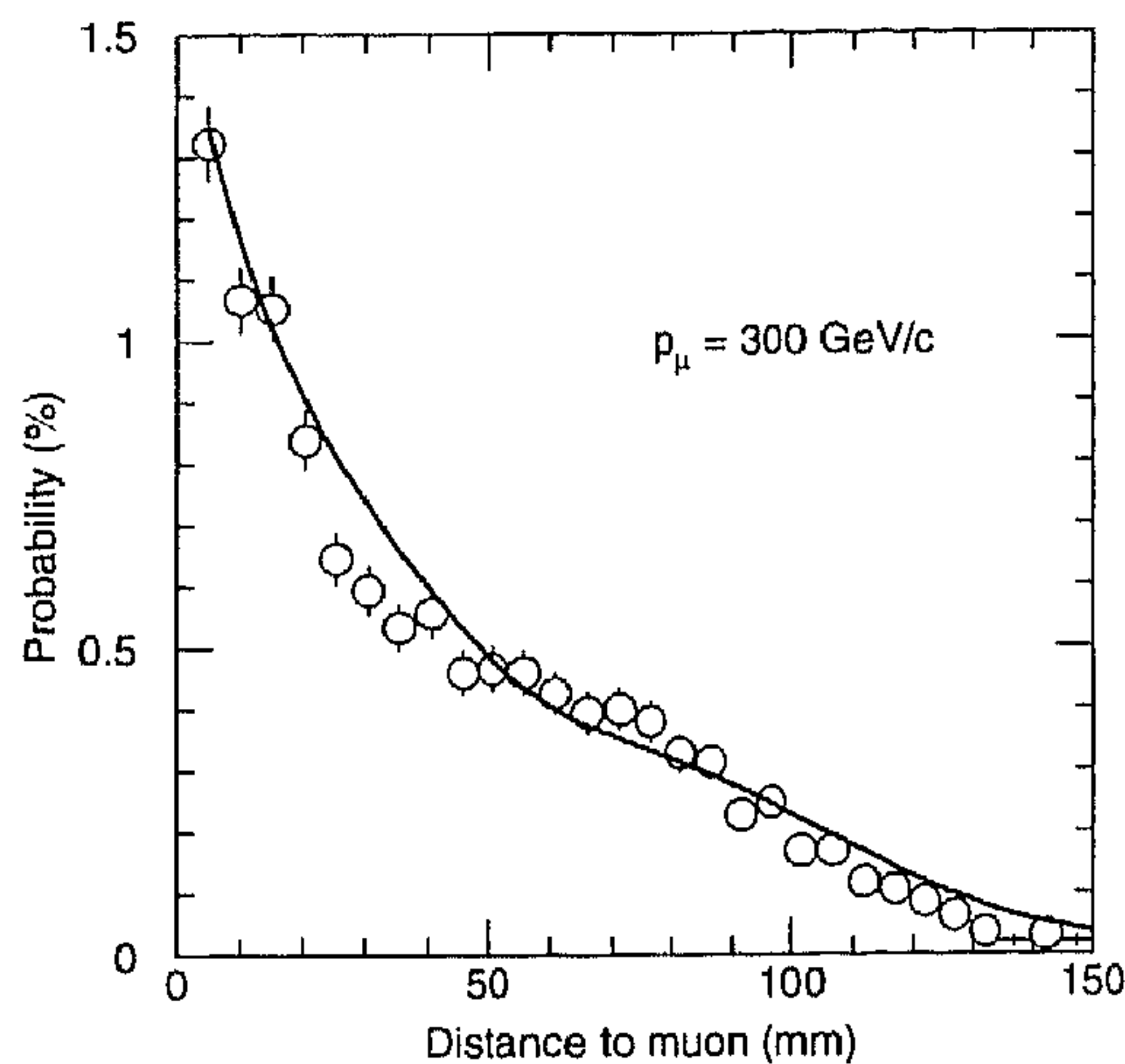
Fig. 9. Comparison of GEANT Monte Carlo simulation (line) and measured (points) probability of secondary tracks vs. the distance from the muon for 300 GeV/c incident muons. "Tracks" taken here as charge clusters in all 4 CSC layers.
