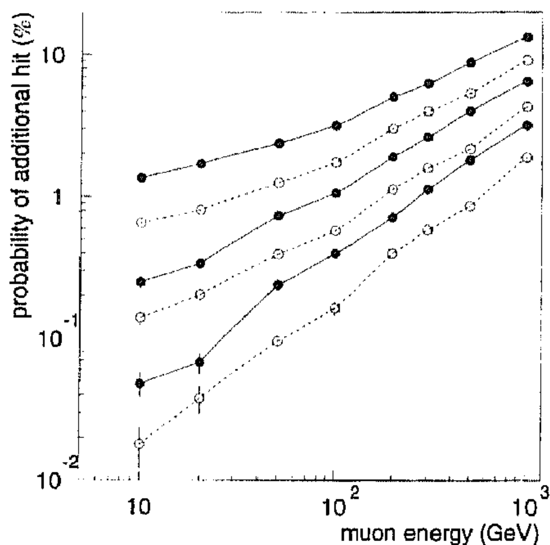
Fig. 18. Simulation: probability of having a muon hit spoiled by the presence of at least one additional electron hit within a two hit resolution of 15, 5 and 2 mm (top to bottom). The detector is at 15 cm from the absorber. Solid lines are for magnetized iron; dashed lines for 0.6 T downstream of the absorber.
