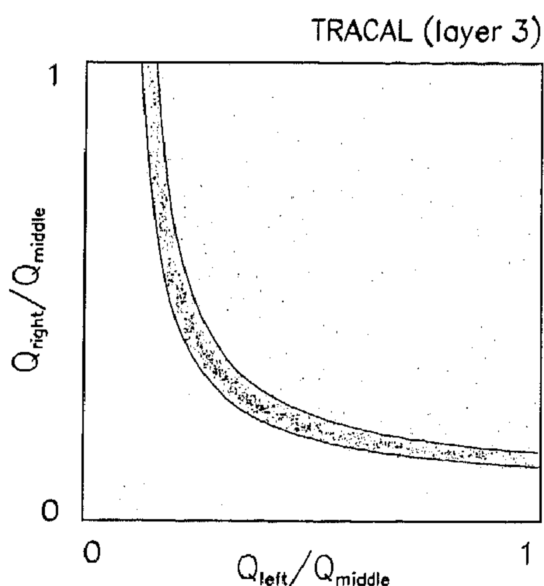
Fig. 5. The ratio Q_{\text{right}}/Q_{\text{middle}} plotted against Q_{\text{left}}/Q_{\text{middle}} for a single-layer HSC in TRACAL. The entries above the expected range (solid lines) are clearly visible.
