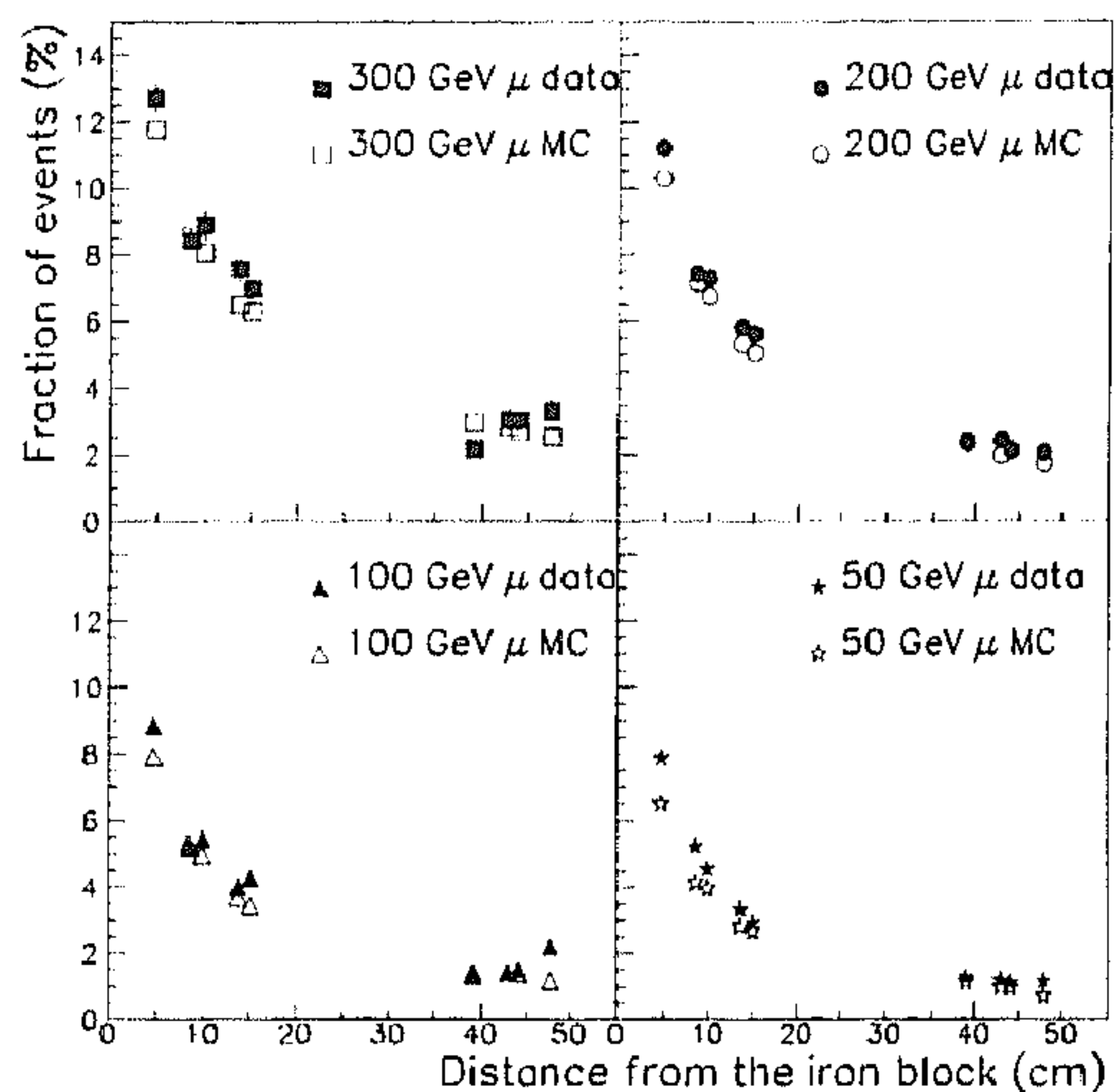
Fig. 2. Fraction (%) of events in SiBT with at least 1 additional hit \geq 100 \mu\text{m} apart from the muon track in the silicon planes, versus the distance of the detector plane from the iron absorber, for different beam energies.
