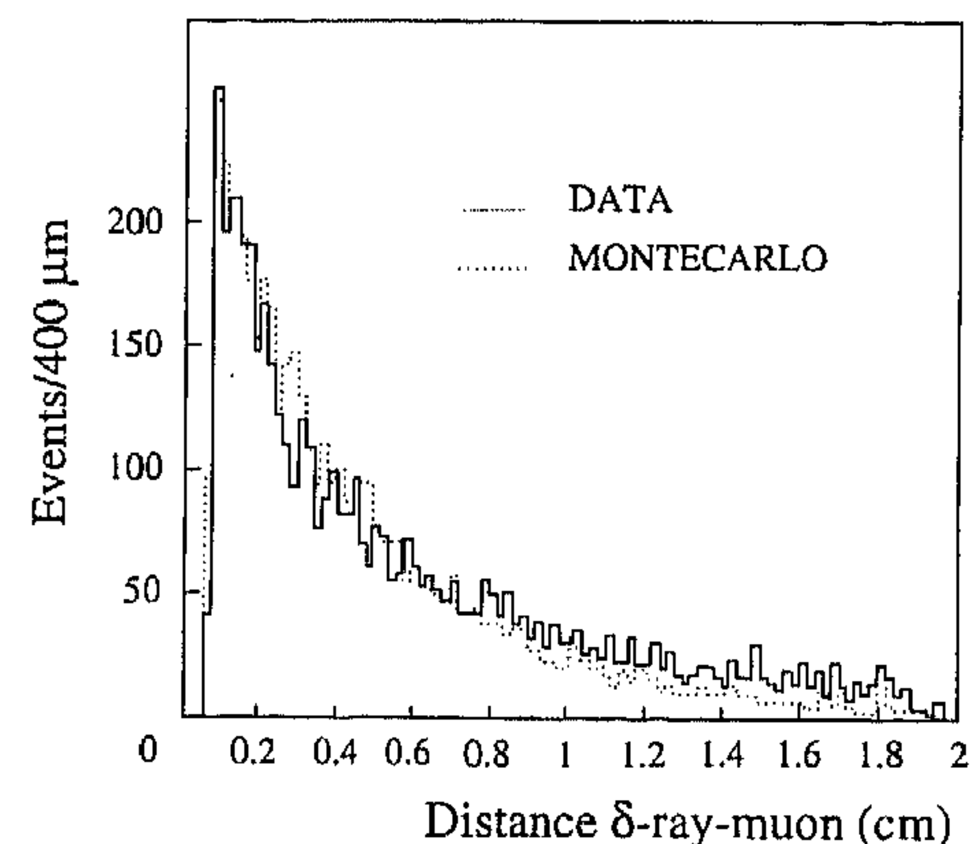
Fig. 16. Distribution of the distance between the "spoiled" hit and the muon track, as obtained from mean timing measurement in the DTBX and from simulation.
