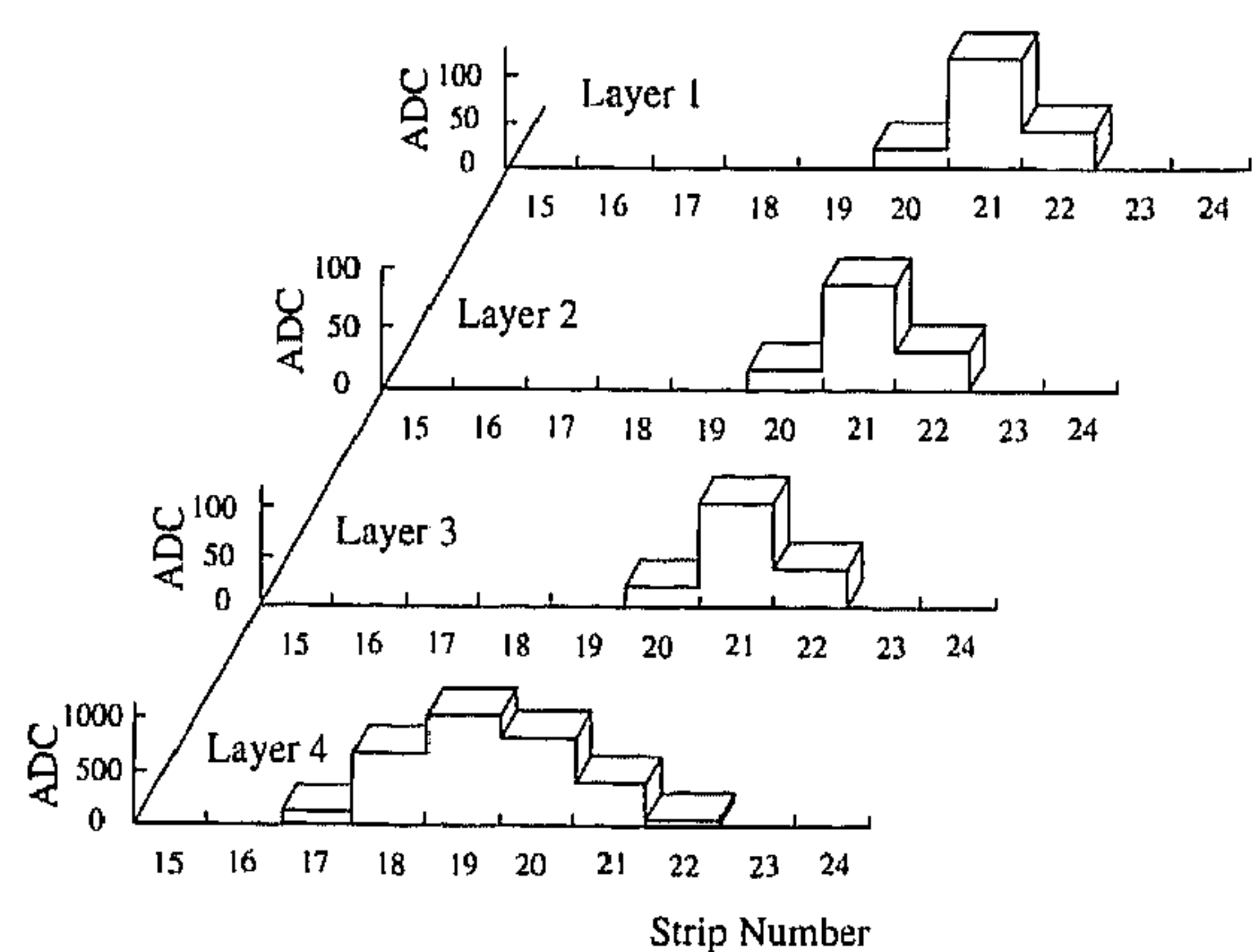
Fig. 6. Display of a typical event in the CSC, with a single track reconstructed in the three upper layers. The charge distribution in the fourth layer (bottom) identifies it as an event with \delta -electron production, since it is clearly wider and shifted w.r.t. the primary particle track.
