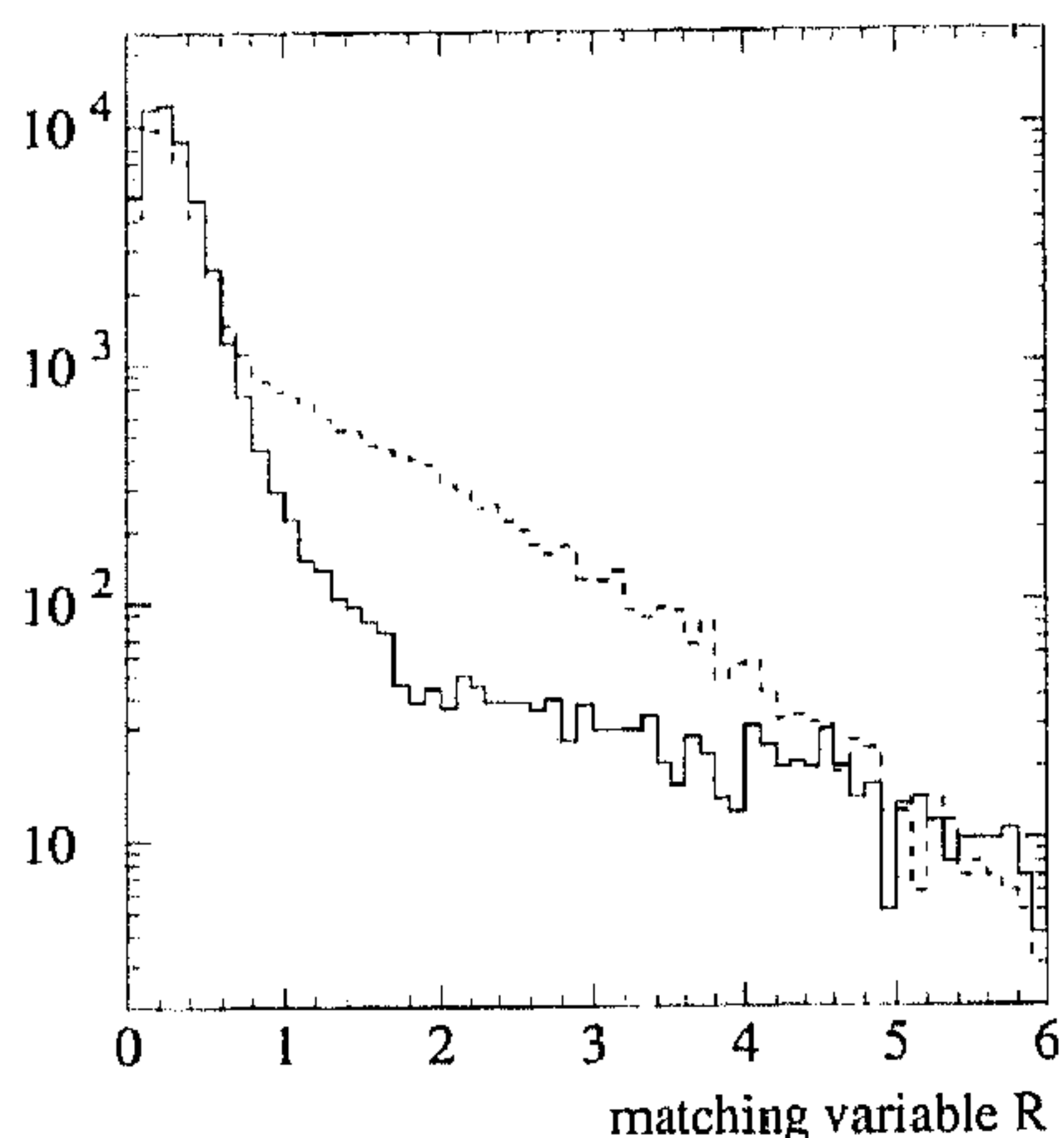
Fig. 21. Distribution of the matching variable R using all hits (dashed line) and after removal of hit(s) outside 350 \mu\text{m} and refitting the track (solid line) for simulated events in an 8-layer WLDC. The fraction of tracks having R above 1 is reduced from 17.2% to 4.1%. Here R is calculated w.r.t. the (known) true muon track.
