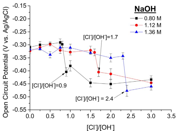
Fig. 4. Measured open circuit potential values (V vs. Ag/AgCl) for steel immersed in chloride-contaminated NaOH solutions. OCP values are plotted against the ratio [\text{Cl}^-]/[\text{OH}^-] .
