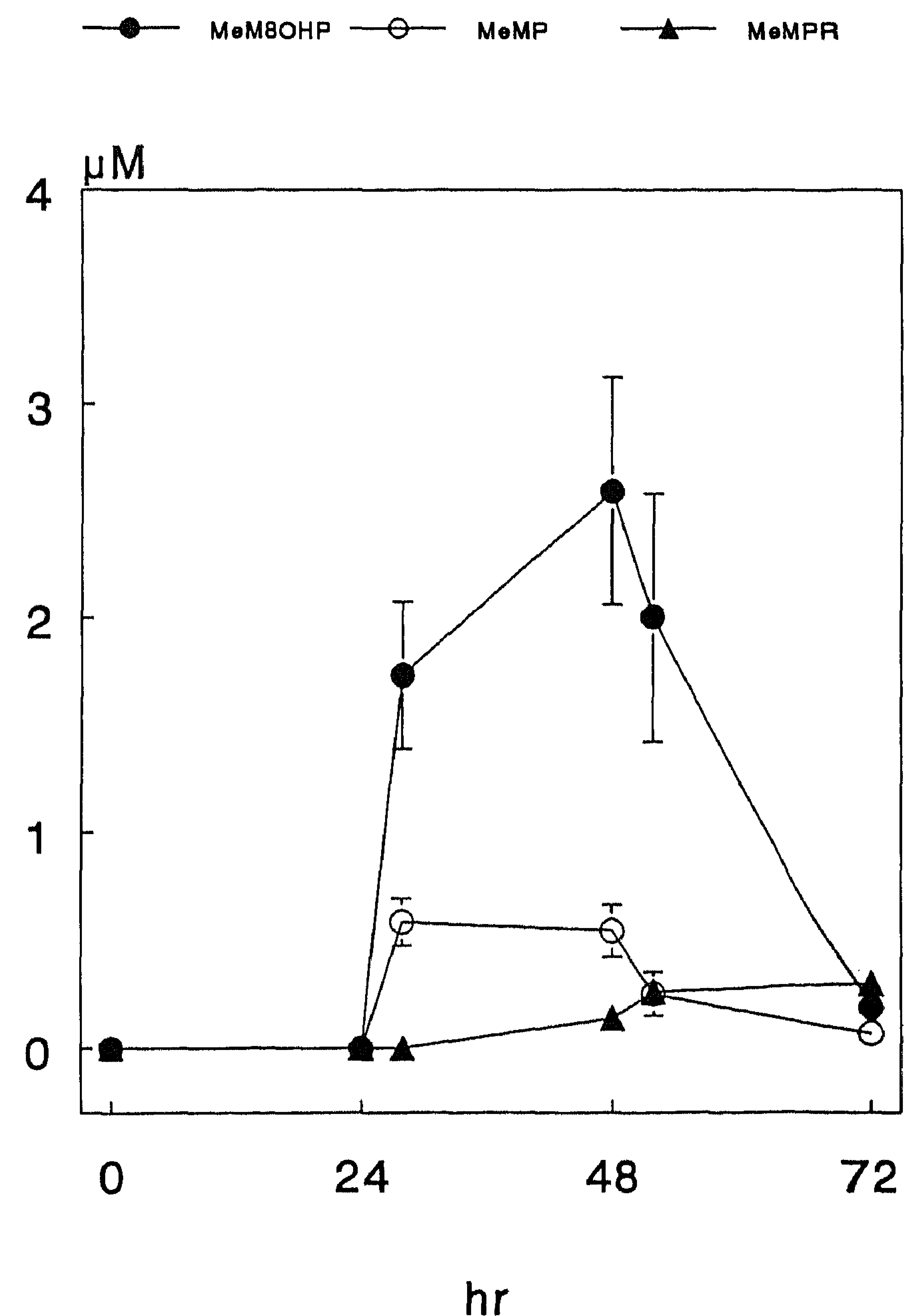
FIG. 1. Methylated metabolites of 6MP in plasma of the intravenous 6MP group. Patients were treated with an MTX infusion from 0–24 hr and a 6MP infusion from 24–48 hr. The means of all courses and all patients are indicated by the markers, the error bars indicate the SEM.
