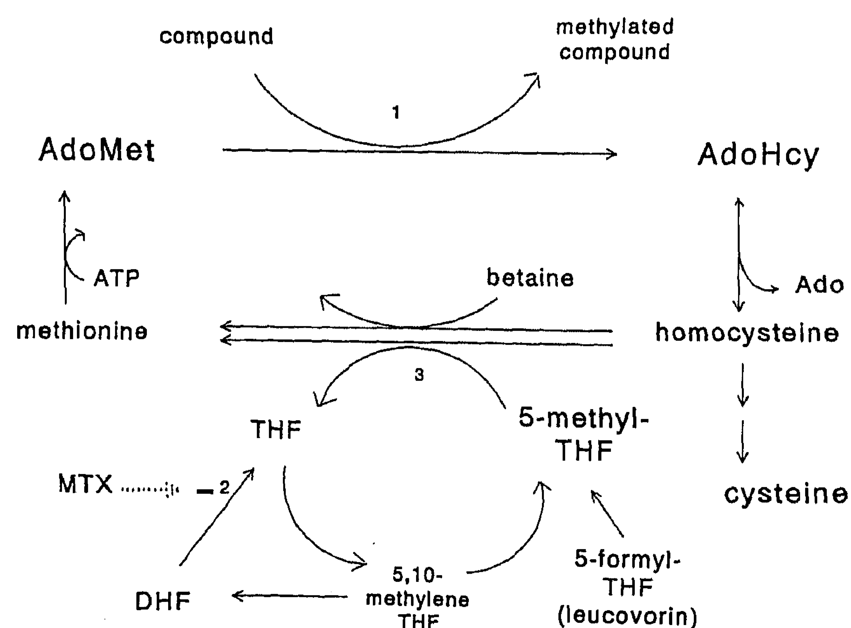
SCHEME 2. The transmethylation pathway. 1, thiopurine-methyltransferase and other AdoMet-dependent methyltransferases; 2, dihydrofolate reductase; 3, 5-methyltetrahydrofolate homocysteine methyltransferase; DHF/THF, di/tetra hydrofolate.
