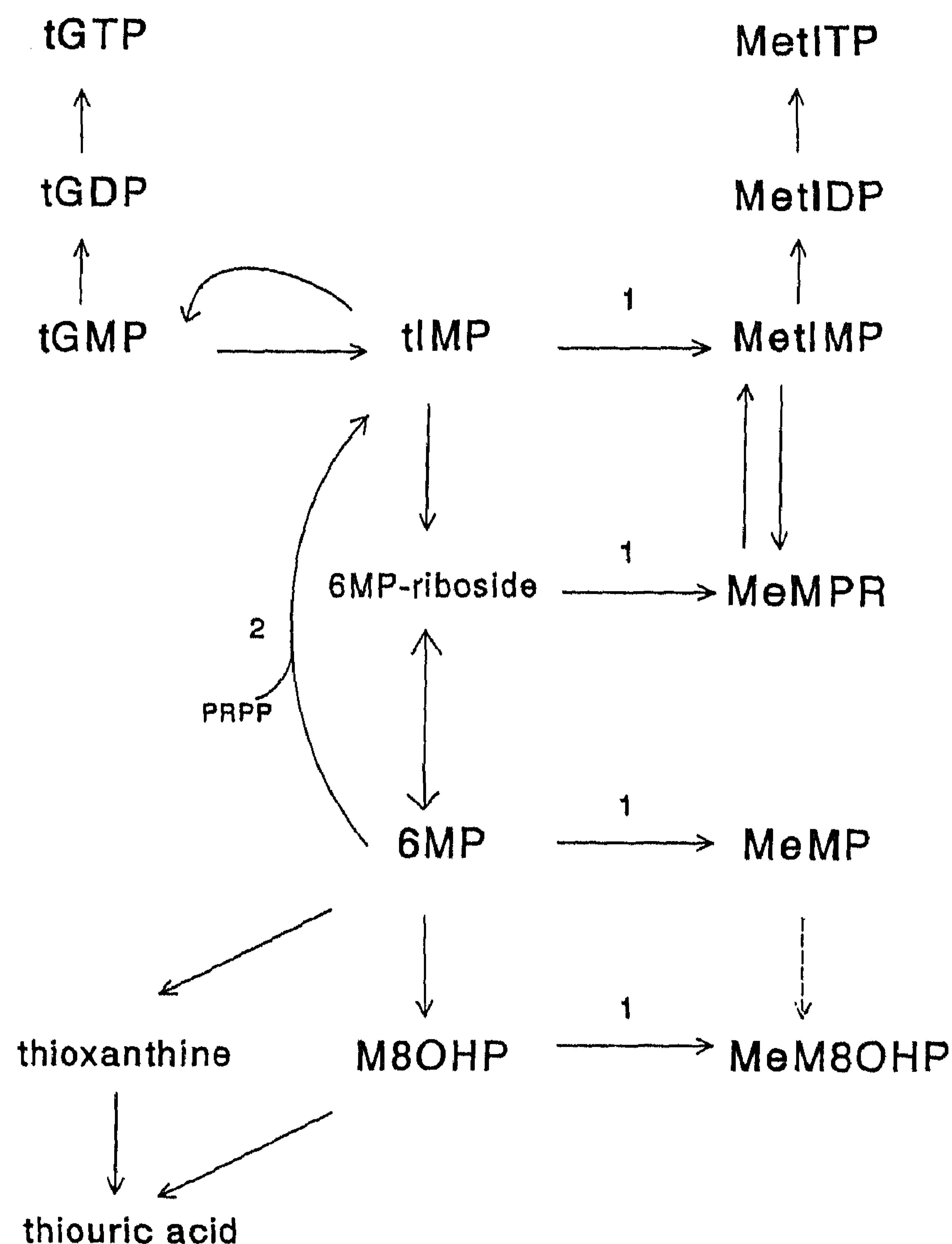
SCHEME 1. The metabolism of 6MP. 1, thiopurinemethyltransferase; 2, hypoxanthineguanine phosphoribosyltransferase (EC 2.4.2.8); M8OHP, 6-mercapto-8-hydroxypurine; PRPP, 5-phosphoribosyl-1-pyrophosphate.
