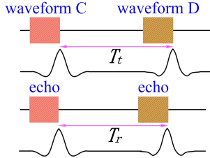
Fig. 12. Doppler speed measurement principle when the sonar system and the target move in opposite directions.
