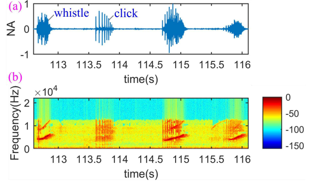
Fig. 1. Clicks and whistles produced by the false killer whale.
