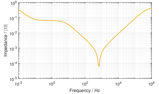
Fig. 3: Impedance Spectrum for Hybrid Model, Neglecting R_1 & L_1
