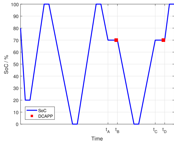
Fig. 5: Test Procedure SoC Profile & DCAPP Locations
