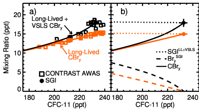
Figure 6. Stratospheric tracer relations between bromine and CFC-11 in winter 2014. In both panels, orange is the sum of bromine supplied by only long-lived compounds ( \text{CH}_3\text{Br} and halons), and black is the sum of bromine supplied by long-lived compounds and VLS. The circle points and error bars are the mean and standard deviation of \text{CBr}_y and CFC-11 at the base of the stratosphere (i.e., CFC-11 = 233 ppt). (a) The solid lines are the calculated relation between \text{CBr}_y and CFC-11 from CONTRAST and ATTREX observations (Table 2). The squares represent the sum of CONTRAST measurements of bromocarbons collected during RF06 and RF15. (b) \text{Br}_y^{\text{SGI}} (dashed lines) calculated from the difference between \text{CBr}_y (solid lines) and \text{SGI}^{\text{LL+VLS}} (dotted lines) using equation (4).
