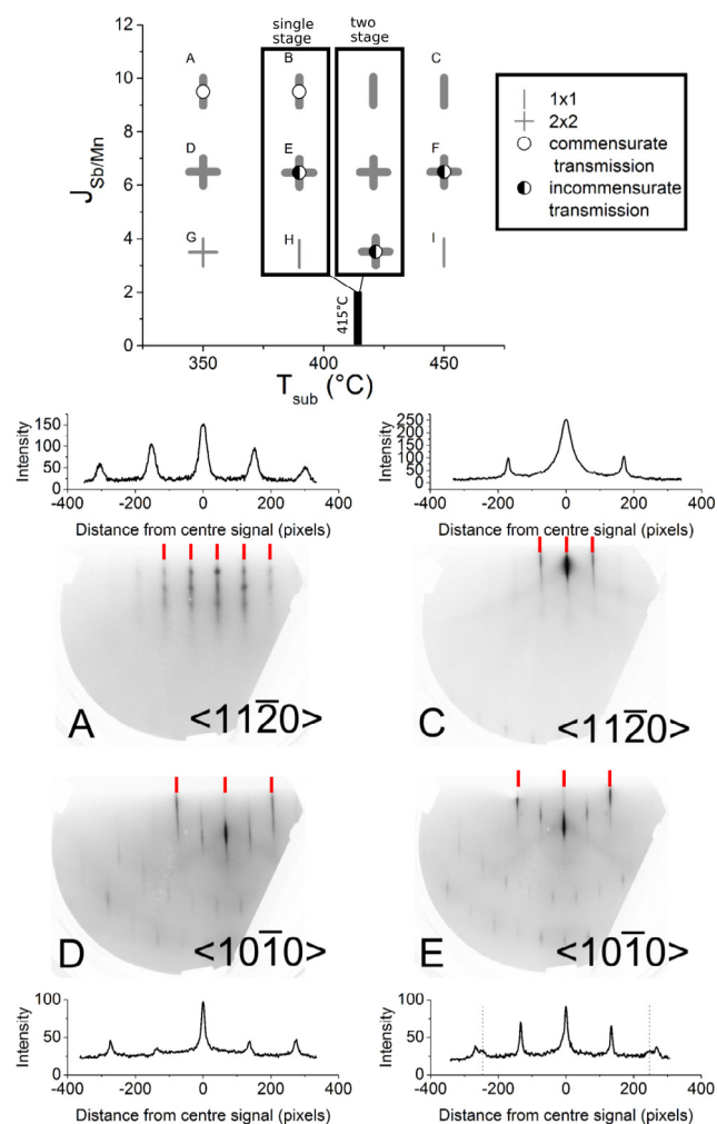
Fig. 1. RHEED pattern summary (upper panel) and examples (lower panels) for MnSb growth on \text{InGaAs}(111)\text{A} as a function of substrate temperature T_{\text{sub}} and Sb/Mn flux ratio J_{\text{Sb}/\text{Mn}} . Patterns A, C, D and E exemplify the main features observed in the two principal surface azimuths, and line profiles across each pattern are also shown. Red lines indicate the integer streak positions for each pattern. (For interpretation of the references to colour in this figure legend, the reader is referred to the web version of this article.)
