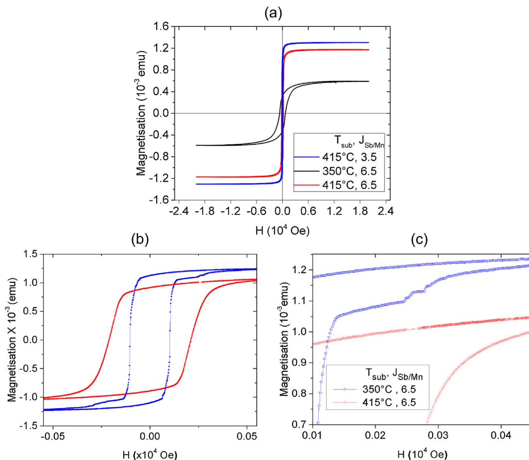
Fig. 8. (a) M Vs H measurements obtained using a VSM at 10 K for MnSb/InGaAs(111)A grown using favourable ( J_{Sb/Mn} = 6.5 ) and non-favourable ( J_{Sb/Mn} = 3.5 ) growth conditions, with the magnetic field aligned in-plane. (b) and (c) are enlarged versions of the M Vs H loops for J_{Sb/Mn} = 6.5 samples
