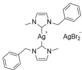
Fig 1. Chemical Structure of Ag8
