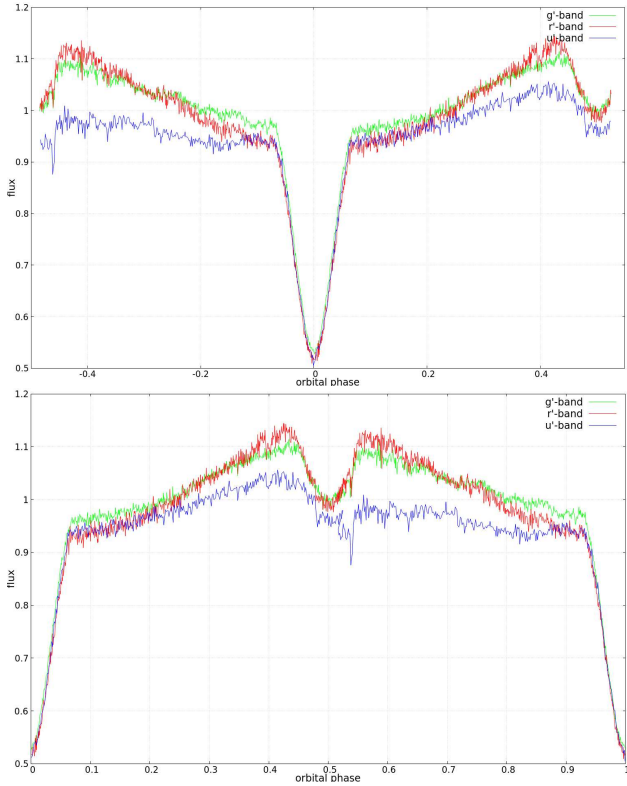
Figure 6. Top: Original ULTRACAM light curves; bottom: Light curves adapted for MORO. The second minimum lays now at \Phi = 0.5 , the blue light curve is obviously not usable for further analysis.
