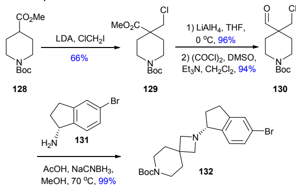
Scheme 35 Reductive amination and chlorine displacement to form the azetidone of the 4-spiropiperidine.
