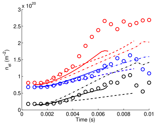
Figure 2. Time evolution of the measured (circles) and simulated (lines - plain = \Delta\phi_{MGI} = 2 ; dashed = \Delta\phi_{MGI} = 0.5 ; dash-dotted = \Delta\phi_{MGI} = 100 ) line integrated density for the three interferometry lines of sight
