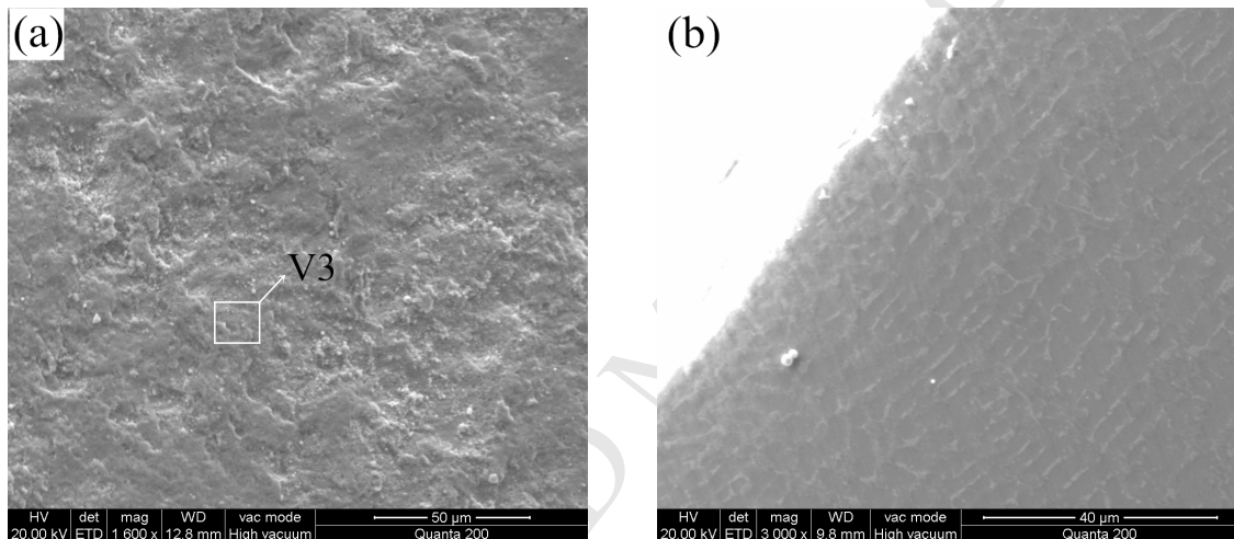
Fig. 22 (a) Worn surfaces of valve 4 seating face and EDS test area V3; (b) cross-section of valve 4 seating face.
