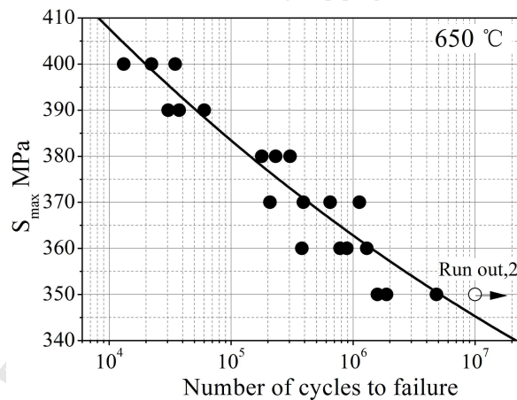
Fig. 13. S–N curves of 23-8N steel at 650 °C.
