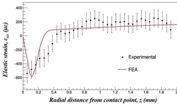
Fig. 10. Subsurface axial ( \epsilon_{xx} ) strain averaged through the sample, as a function of distance from the contact site, compared to the same component of average FEA strain.
