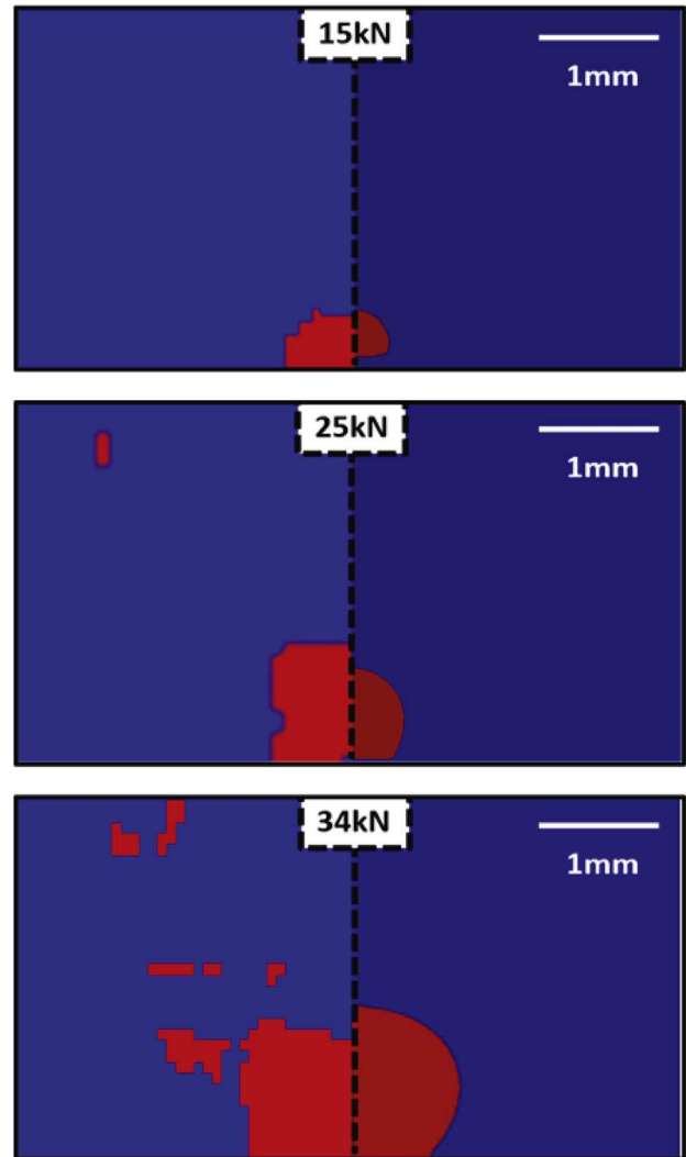
Fig. 11. (Top) Radiograph indicating the region of interest, beneath the contact. (Bottom) Comparison of \sigma broadening parameter and the active yield region at the contact site, with applied loads of 15 kN, 25 kN and 34 kN load.
