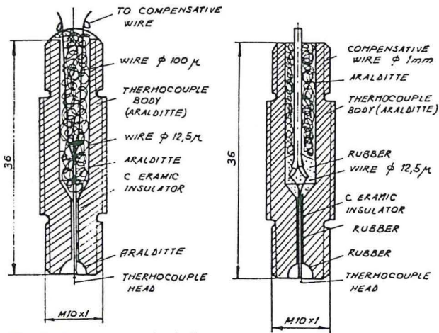
Fig. 1 Thermocouple design
