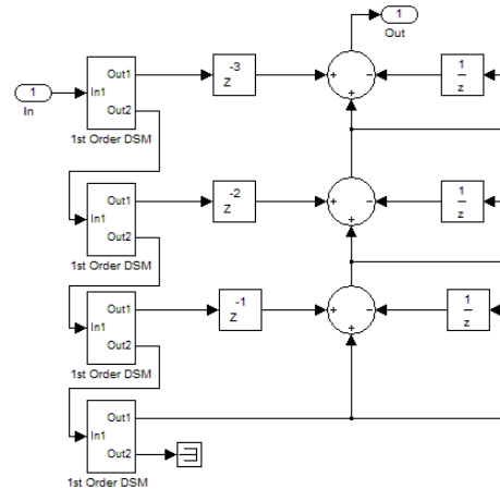
Figure 2. Simulink Model of MASH 1-1-1-1 DDSM
