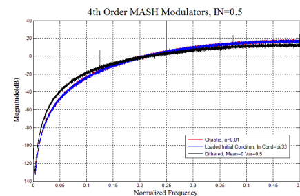
Figure 13. Output Spectrum of MASH 1-1-1-1 Modulators
