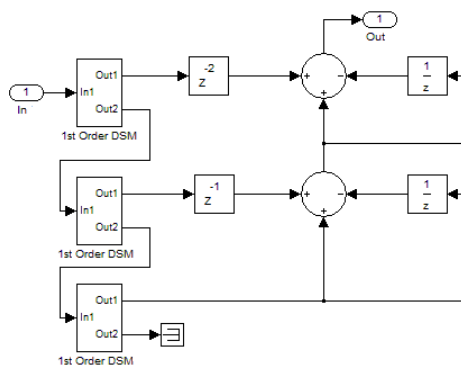
Figure 1. Simulink Model of MASH 1-1-1 DDSM
