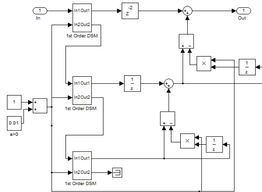
Figure 6. Simulink Model of MASH 1-1-1 Chaotic Modulator
