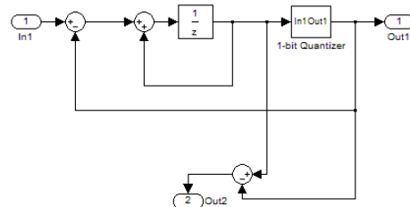
Figure 3. Simulink Model of 1 st Order DDSM used in MASH 1-1-1 and MASH 1-1-1-1 stages
