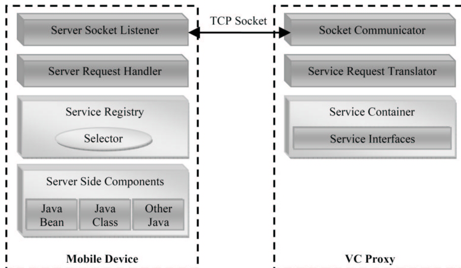
Figure 1: Architectural Overview of MPA/LSC and VC Proxy
