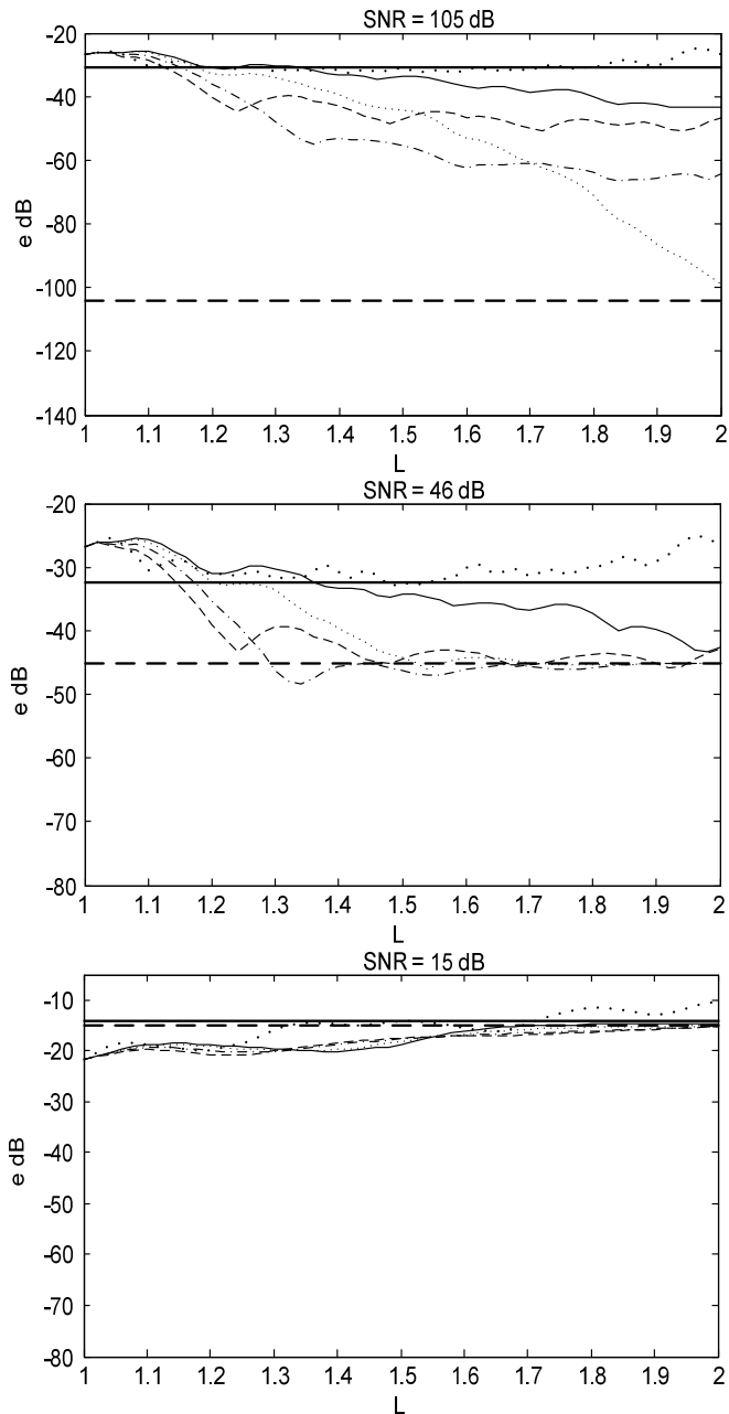
Figure 4, Maximum reconstruction error for various filter normalized bandwidths for noisy cases.
