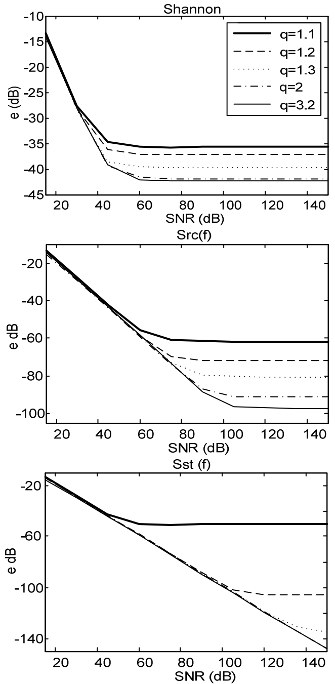
Figure 5, Maximum reconstruction error for selected methods with changing SNR and oversampling ratios.
