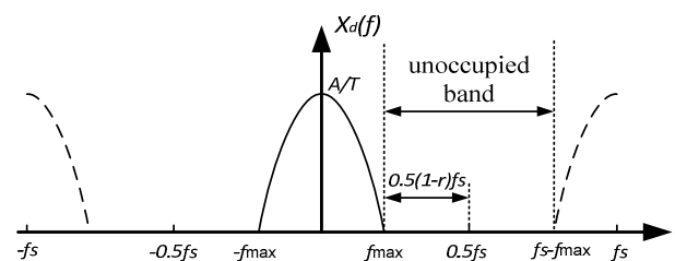
Figure 1, Spectrum of a typical sampled waveform
