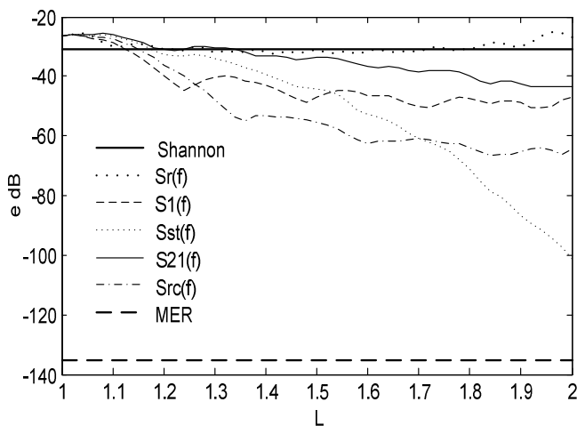
Figure 2, Maximum reconstruction error versus normalized filter bandwidth for noise free case.
