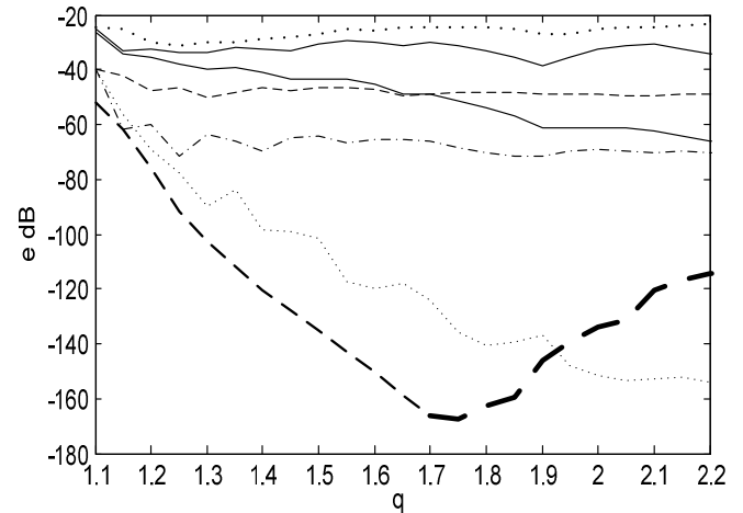
Figure 3, Maximum reconstruction error versus oversampling ratio for noise free cases.
