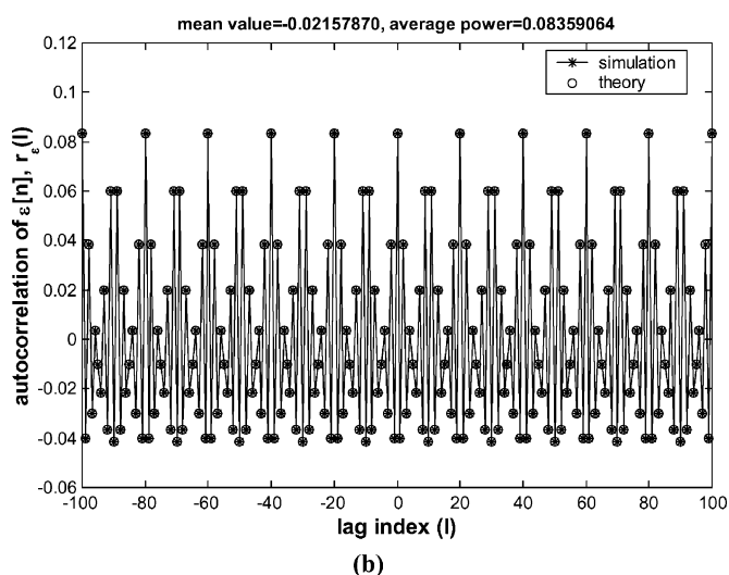
Fig. 4. Autocorrelation function for the binary quantizer error in the first-order modulator with 0.1 dc input. (a) v_0 = 0.60684258354180 . (b) v_0 = -0.60684258354180 .
