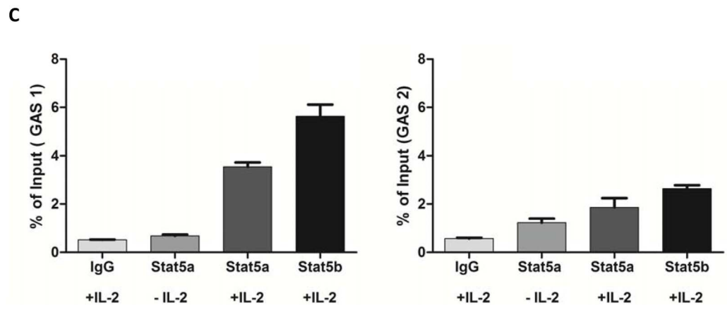
Figure 4. Study of the binding site, location and validation of the cloned fragment obtained by ChIP. A. Sequence of the cloned fragment and the corresponding typical and atypical GAS sequences present. There is a TTN 5 AA (blue font) sequence and one typical GAS TTCN 3 GAA (red font) sequence present within the cloned fragment. B. The relative location of the cloned fragment, GAS1 and GAS2 with respect to the FRA2 transcription start site (TSS) and intron/exon is shown schematically and its coordinates on the UCSC genome browser. Figure 4C: IL-2 induces in-vivo binding of STAT5 to GAS1 within the third intron of the FRA2 gene in preactivated CD4 T cells. STAT5-ChIP samples from ±IL-2-treated preactivated CD4 T cells were analysed by real-time PCR for specific binding to the two GAS motifs identified above. ChIP assay was performed using the LowCell# ChIP kit and ±IL-2-treated preactivated CD4 T cells. Enrichment of GAS 1 was higher when compared to GAS 2 and more so with the STAT5b antibody. doi:10.1371/journal.pone.0090370.g004
