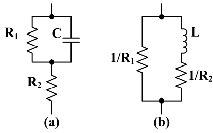
Fig. 5. Model for a) Capacitor, b) Inductance.
