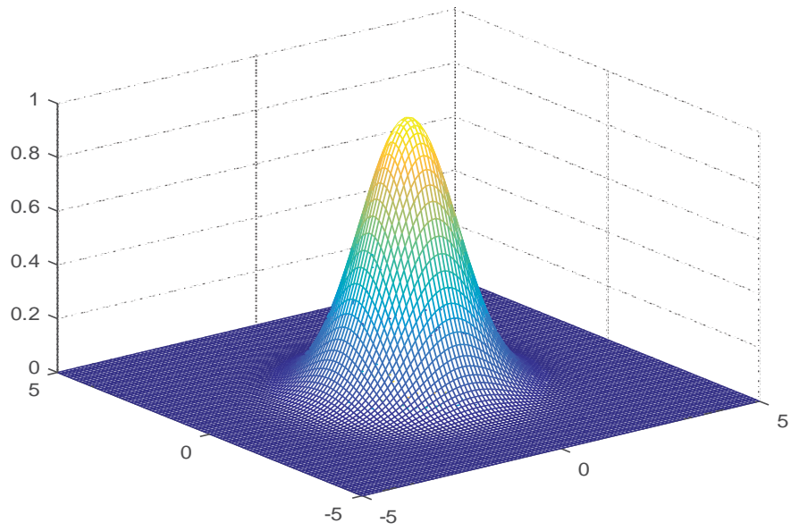
Figure 1.1: Gaussian DECO. \rho_t = 0.05 .
