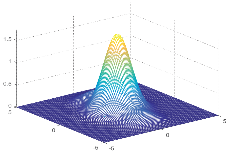
Figure 1.2: MME-DECO. \rho_t = 0.05 , \gamma_{14} = 0 , \gamma_{16} = 0.0005 , \gamma_{24} = 0.065 , \gamma_{16} = 0.0002 .
