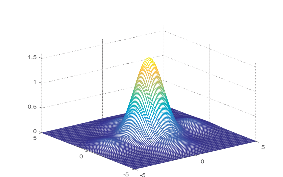
Figure 1.3: MME-DECO. \rho_t = 0.05 , \gamma_{14} = 0 , \gamma_{16} = 0.005 , \gamma_{24} = 0.05 , \gamma_{16} = 0.002 .
