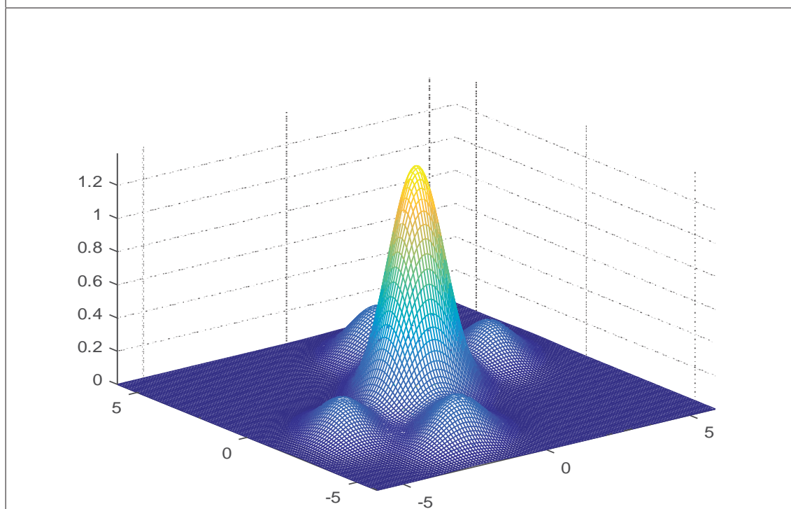
Figure 1.4: MME-DECO. \rho_t = 0.4 , \gamma_{14} = 0 , \gamma_{16} = 0.005 , \gamma_{18} = 0.003 , \gamma_{24} = 0.05 , \gamma_{26} = 0.002 , \gamma_{28} = 0.0005
