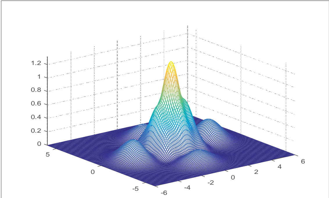
Figure 1.5: MGC-DECO. \rho_t = 0.1, \gamma_{14} = 0.25, \gamma_{16} = 0.025, \gamma_{24} = 0.15, \gamma_{16} = 0.015.
