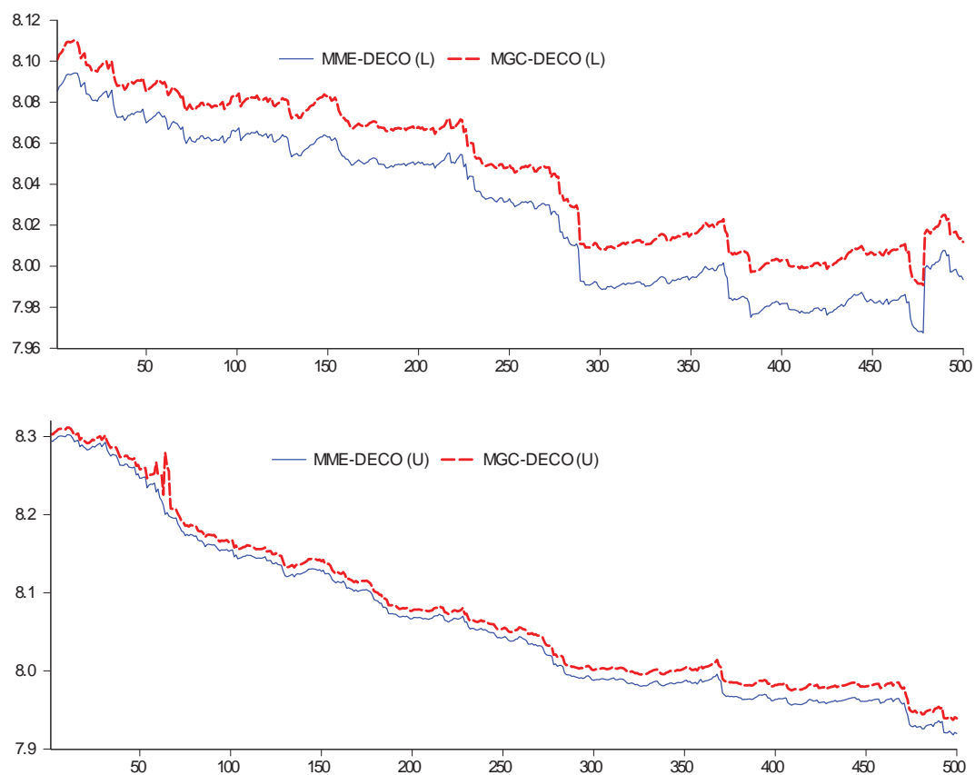
Figure 3: Overall goodness-of-fit of MGC- and MME-DECO
