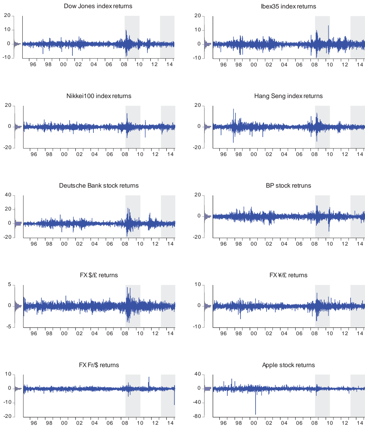
Figure 2: Daily percent log return series
