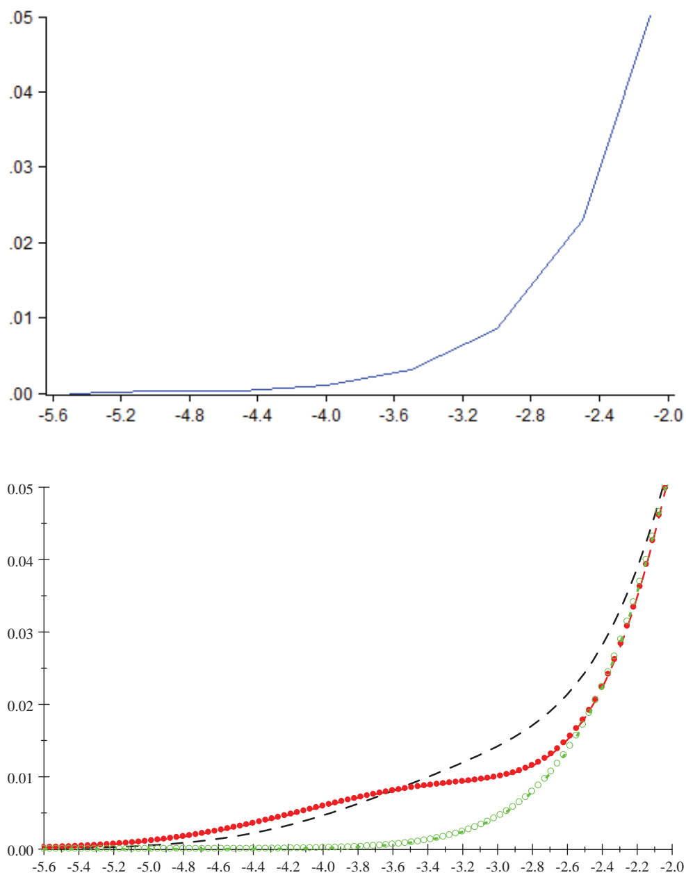
Figure 4: Fitted and empirical marginal densities (left tail)
