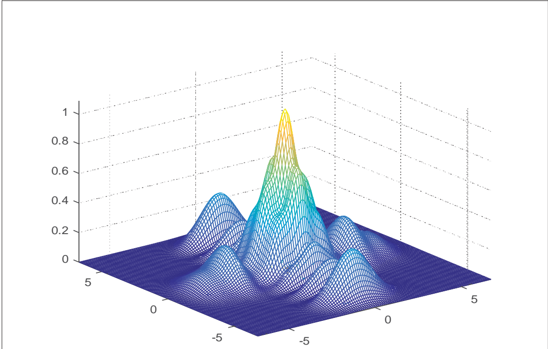
Figure 1.6: MGC-DECO. \rho_t = 0.01, \gamma_{14} = 0.2, \gamma_{16} = 0.02, \gamma_{18} = 0.003, \gamma_{24} = 0, \gamma_{16} = 0.02, \gamma_{28} = 0.007.
