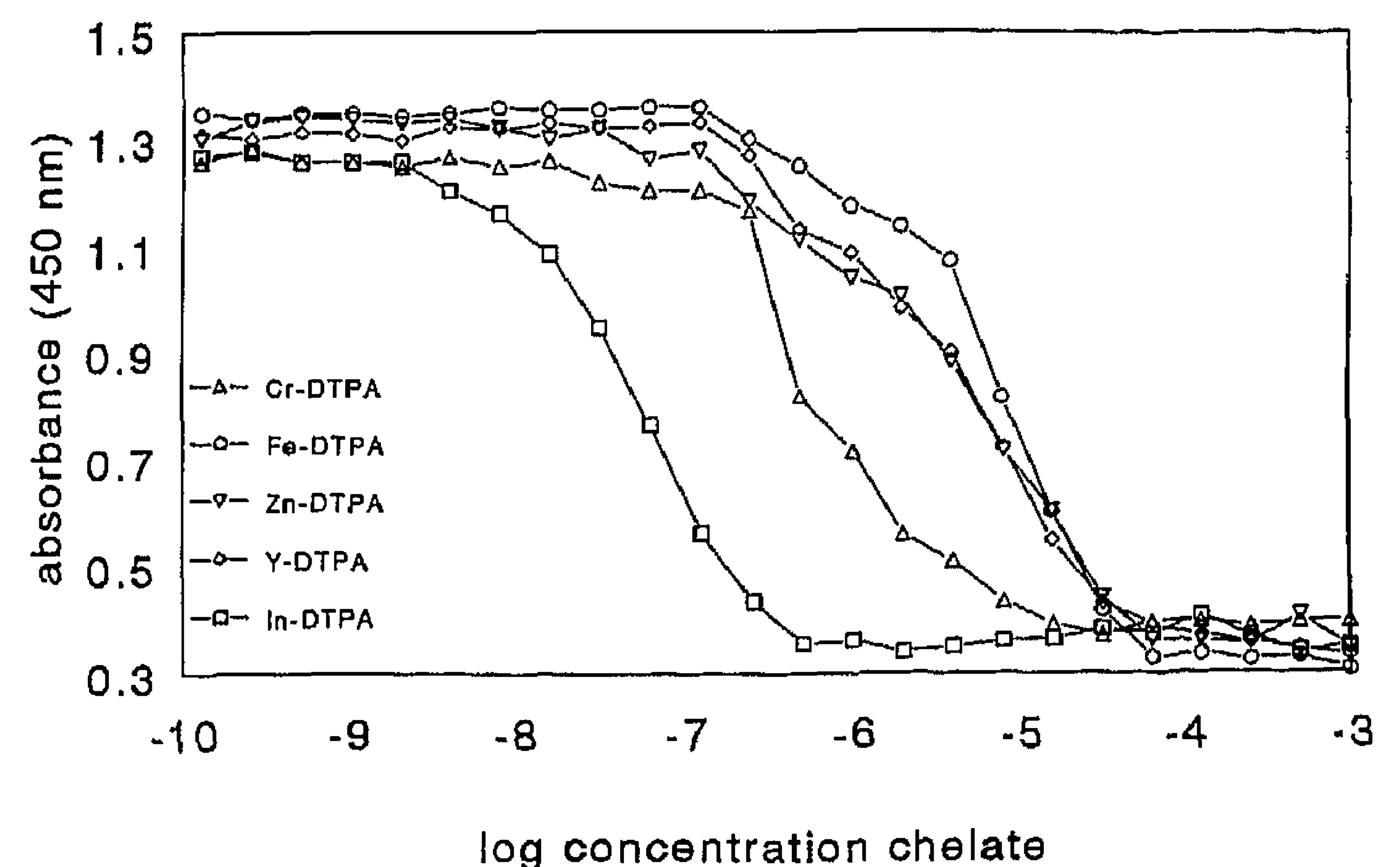
Fig. 1. Competitive antigen-binding assay of DTIn2. The amount of DTIn2 bound to the solid-phase-coated In-DTPA-BSA is plotted versus the concentration of the competing chelate added.
