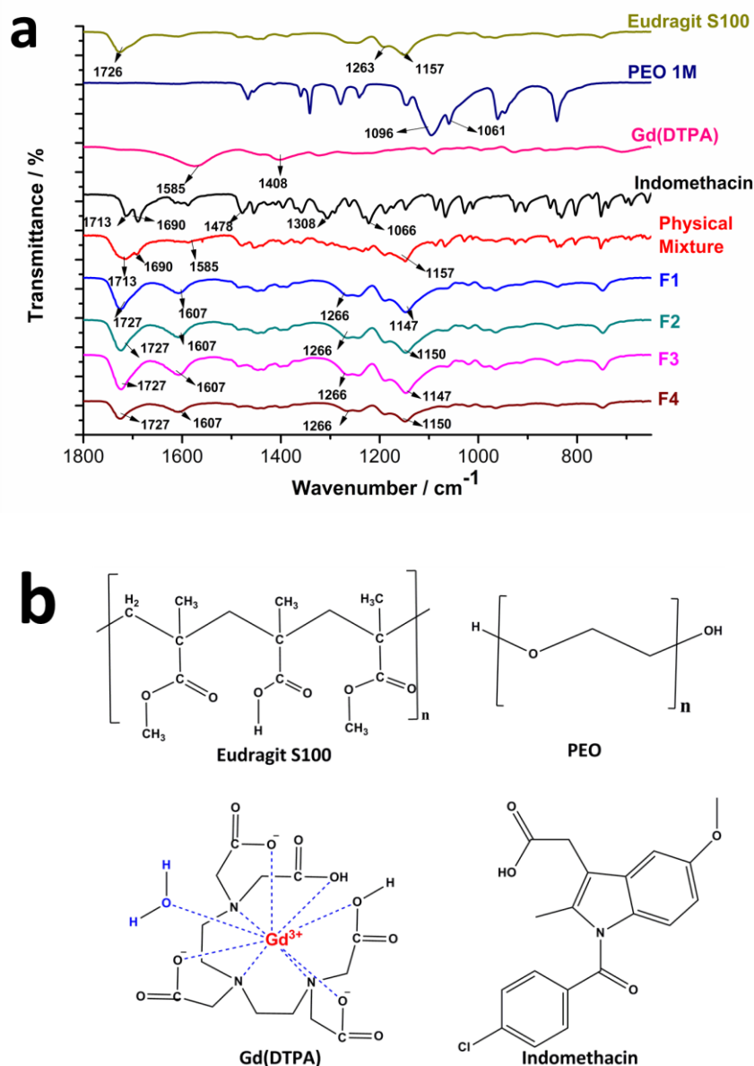
Figure 6. (a) FTIR spectra of the raw materials, a physical mixture, and fibers F1, F2, F3 and F4; (b) Chemical structures of the raw materials.
