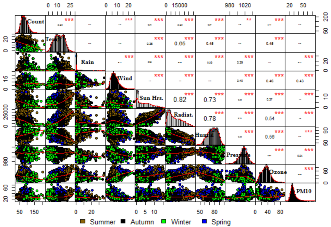
Figure 1: Scatter plot matrix of variables distribution, histograms, kernel density overlays, correlations, and significance
