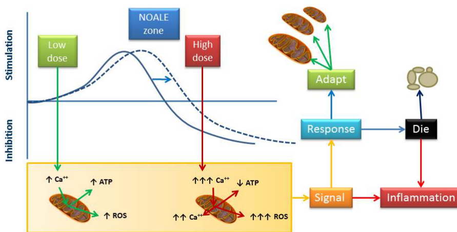
Figure 1: Hormesis – an integrated adaptive homodynamic epiphenomena to stress that increases robustness; mitochondrial example. Solid curve: Immediate response; this is where a “low” dose of a potentially damaging factor, below its No Observed Adverse Effect Level (NOAEL) appears to directly and immediately stimulate an adaptive response, and is a composite of an inhibitory effect of the factor plus a generally counteracting and over-compensating response. For instance, calcium influx into the mitochondrion, generated by a potentially toxic compound opening a plasma membrane calcium channel stimulates production of ATP and buffers calcium. However, too much calcium (or the factor itself) can inhibit mitochondrial function, potentially inducing cell death, ranging from non-inflammatory apoptosis to inflammatory necrosis. Whether or not the stimulation or inhibition is beneficial will therefore depend on context, for instance, it could stimulate neurogenesis or cancer growth via generation of ROS or kill the cells. Dashed curve: Adaptive response; inherent in the system is an overcompensation response. In the above example, increased calcium flux into the mitochondria could generate a ROS signal to enhance mitophagy, anti-oxidant defence and mitochondrial biogenesis, so improving overall calcium buffering and mitochondrial function within a cell. Along with activation of xenobiotic systems, this would make the cell more able to resist a potentially damaging factor if it were re-exposed to it, for instance, if it were a mitochondrial toxin. Hence the curve is shifted to the right and the NOALE and toxicity threshold is raised. The system could therefore be said to be more robust.
