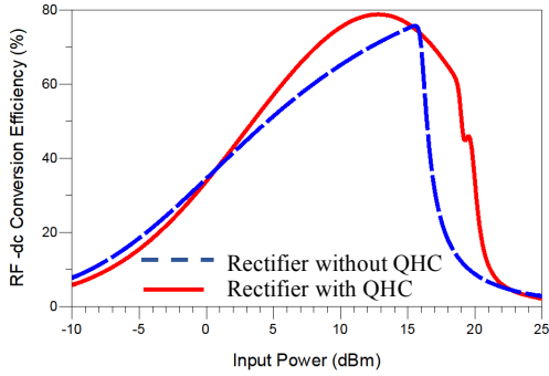
Fig. 5. Simulated efficiencies of the rectifiers with and without coupler versus input power for load ( R_{LOAD} ) of 5\text{ k}\Omega at 1.5\text{ GHz} .
