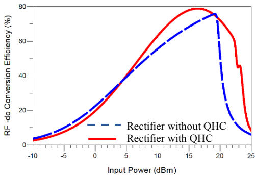
Fig. 7. Simulated efficiencies of the rectifiers with and without coupler versus input power for 3 MHz LTE QPSK signal.
