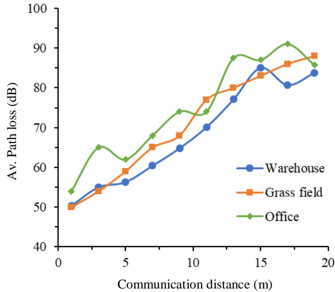
Figure 17. Relationship between communication distance and average path loss for different WSN environments.
