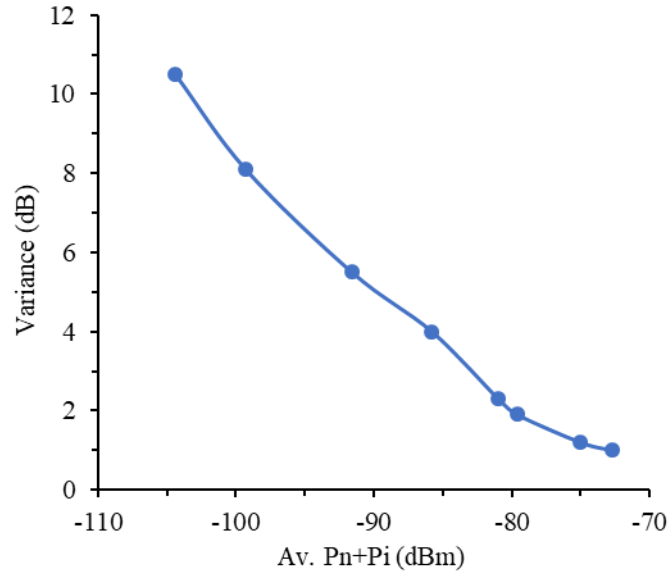
Figure 26. Variance in Av. ( P_n + P_i ) at different power levels.
