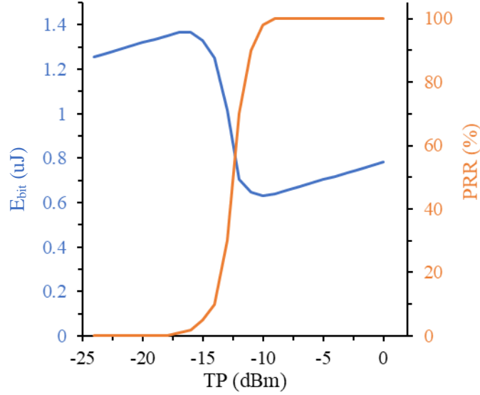
Figure 11. Relationship between TP, communication reliability and E_{bit} [13].
