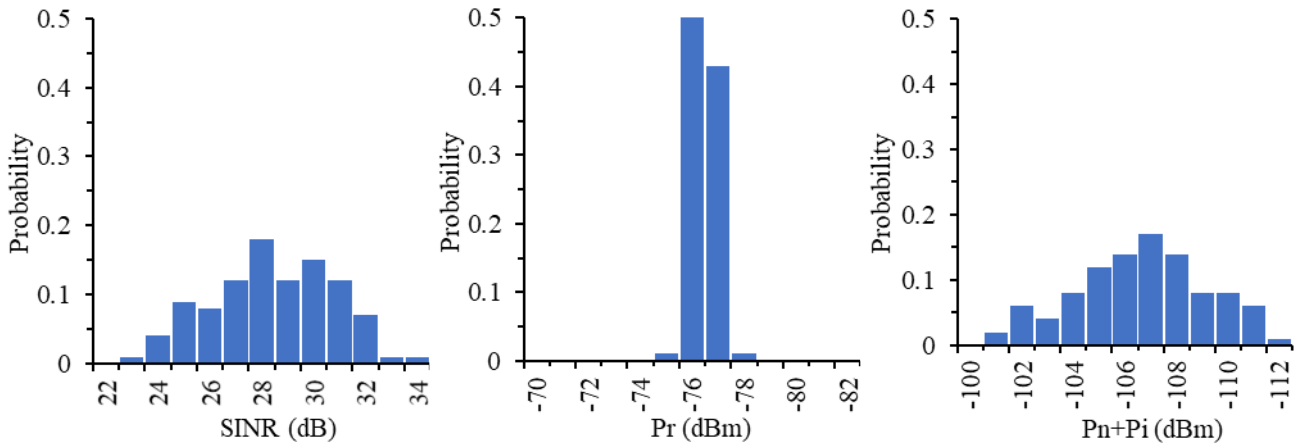
Figure 24. SINR (left), P_r (centre) and P_n + P_i (right) distributions.
