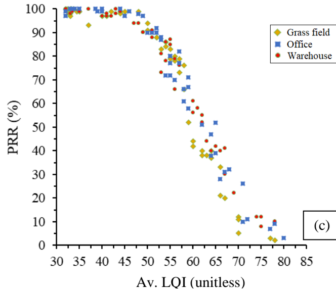
Figure 27. PRR against average RSSI (a), SINR (b) and LQI (c) in grass field, office and warehouse environments.
