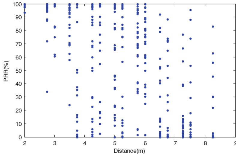
Figure 7. PRR as a function of communication distance for real-world communication links [53].
