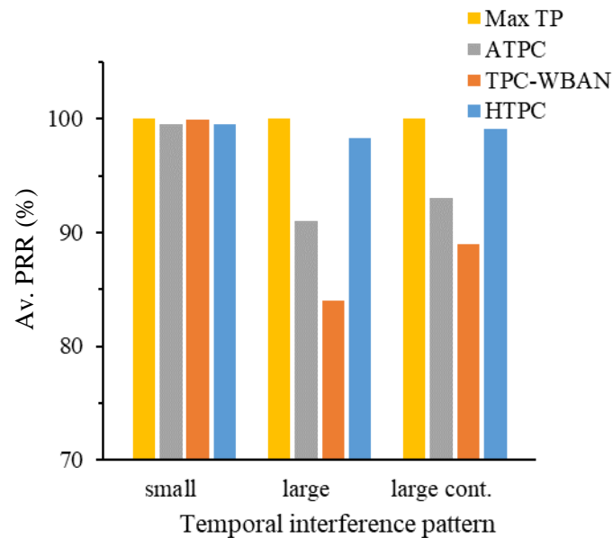
Figure 31. PRR performance evaluation of HTPC and other approaches.
