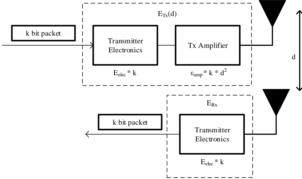
Figure 10. First order HCB energy model [74].
