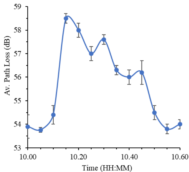
Figure 18. Average path loss over time in a grass field environment.
