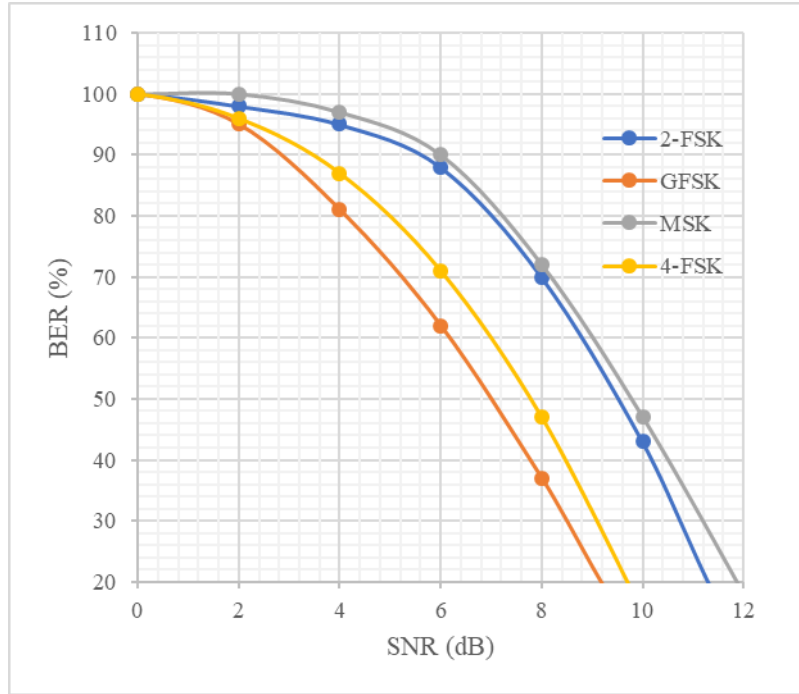
Figure 5. Theoretical BER over SNR for different modulation techniques [50].
