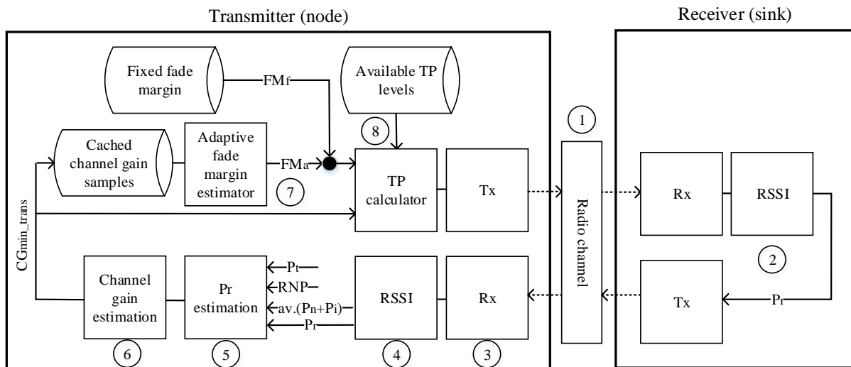
Figure 30. HTPC block diagram.
