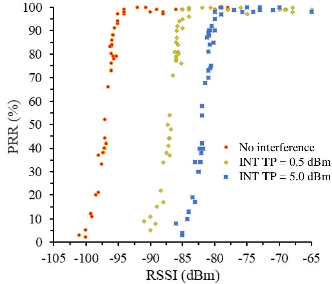
Figure 28. PRR against RSSI with a controllable source of interference in the network.
