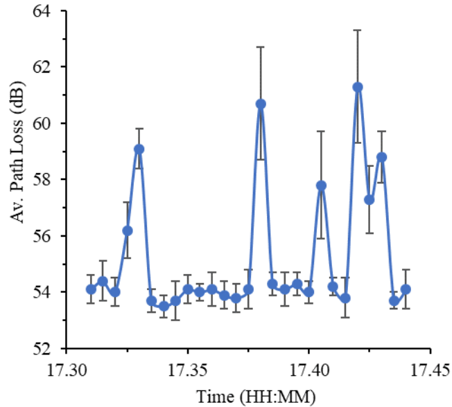
Figure 20. Average path loss over time in warehouse environment.
