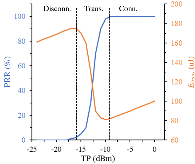
Figure 3. Relationship between TP, E_{trans} and PRR.
