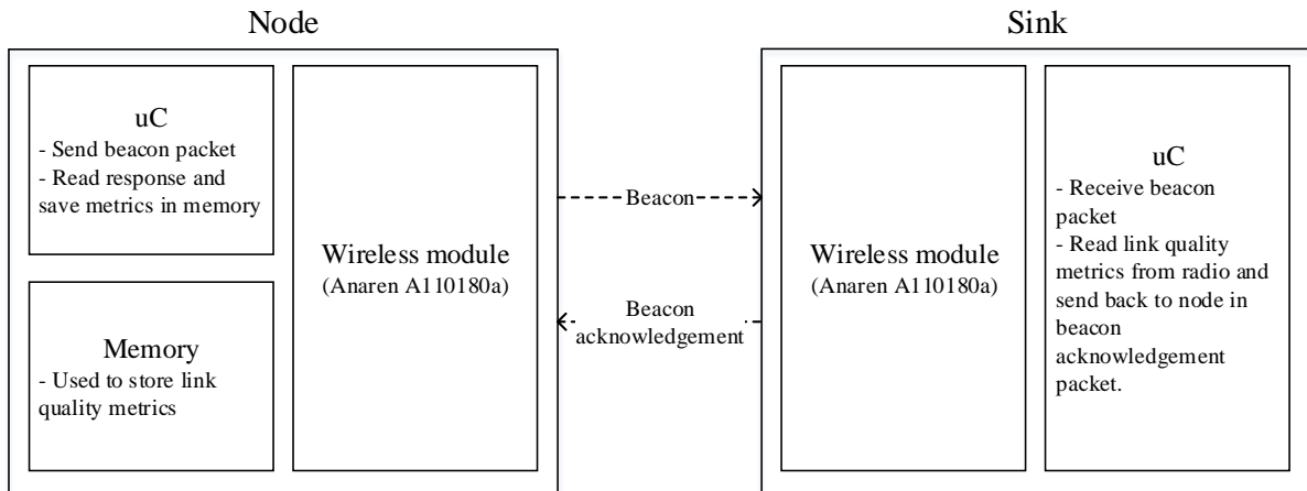
Figure 14. Experimental WSN block diagram.
