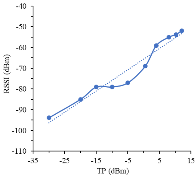
Figure 21. Relationship between RSSI and TP in warehouse environment.
