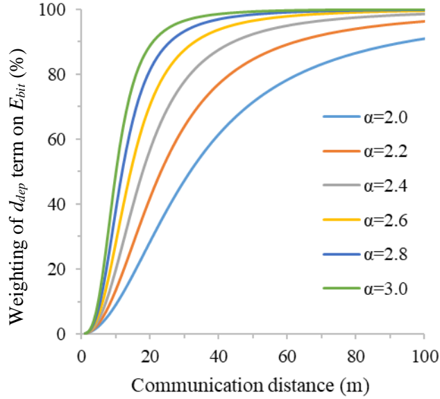
Figure 12. Weighting of distance dependent ( d_{dep} ) term on E_{bit} for varying communication distance and path loss exponent.
