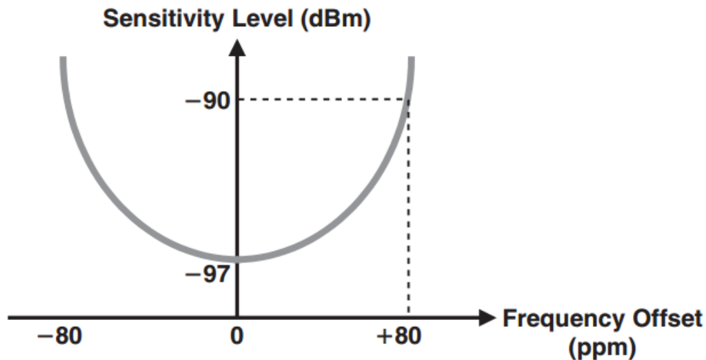
Figure 6. Receiver sensitivity as function of modulation inaccuracy [53].
