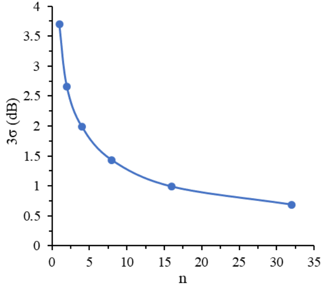
Figure 29. Third standard deviation ( 3\sigma ) of Av.(P_n + P_i) samples with different sample sizes ( n ).
