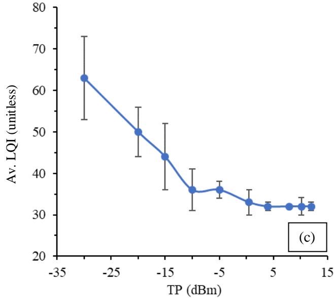
Figure 23. TP against average RSSI (a), SINR (b) and LQI (c).
