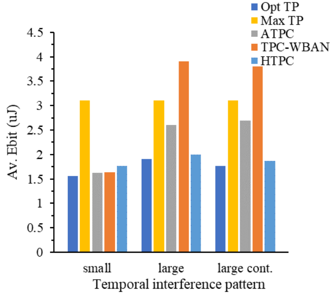
Figure 32. E_{bit} performance evaluation of HTPC and other approaches.
