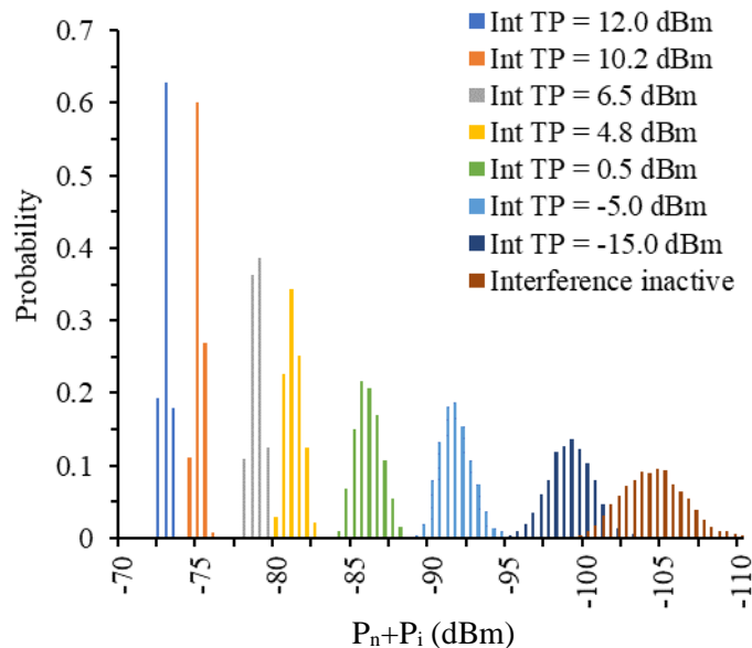
Figure 25. Distribution of P_n + P_i samples at different power levels.
