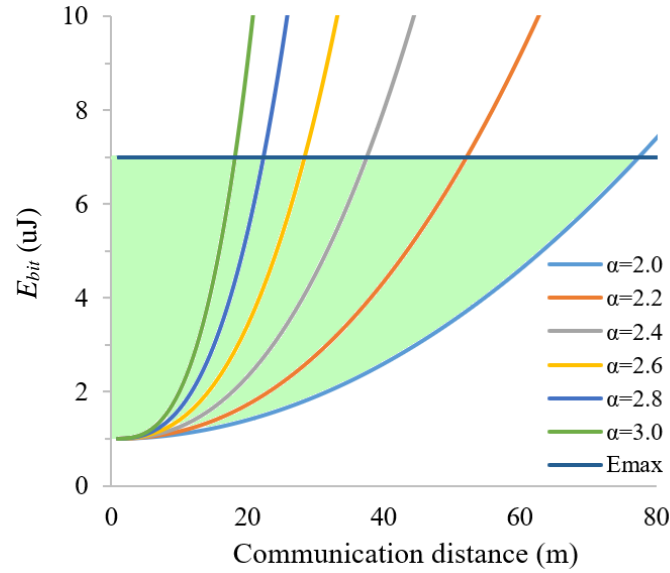
Figure 13. Potential energy savings through using the optimum transmission power.
