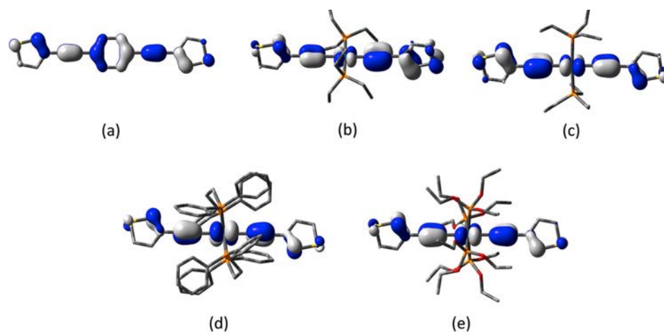
Figure 4 The isosurfaces ( \pm 0.04 ( e \text{ bohr}^{-3} ) 1/2 ) of the HOMOs for: (a) 11 , (b) 14 with the thienyl groups perpendicular to the Pt(II) square plane, (c) 14 with the thienyl groups and the Pt(II) coplanar, (d) 13 , and (e) 12 . From reference [49], reproduced by permission of the owner society.
