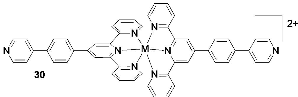
Scheme 9 Structures of molecules 25–30 .
