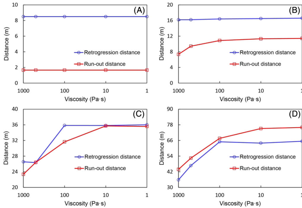
FIGURE 16 Effects of the viscosity on the final retrogression distance and the final run-out distance of the deposit collapse in sensitive clays of (A) St = 1 , (B) St = 2 , (C) St = 4 , and (D) St = 8 [Colour figure can be viewed at wileyonlinelibrary.com ]
