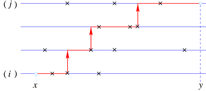
FIGURE 4.1. A staircase path from (x, i) to (y, j) jumps upwards at skeleton points (denoted by \times ) but may skip several of them before deciding to make a jump
